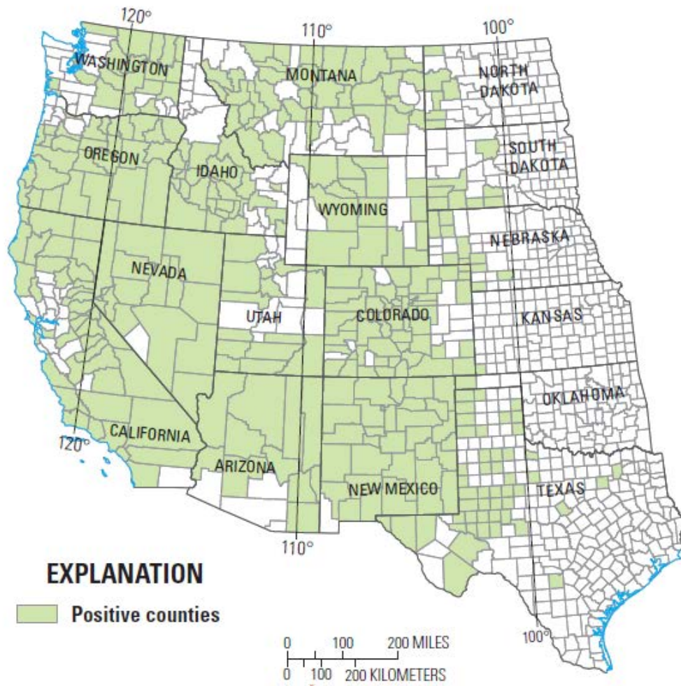
Figure 2. U.S. counties with plague-positive animal or flea samples (Abbott and Rocke 2012).
