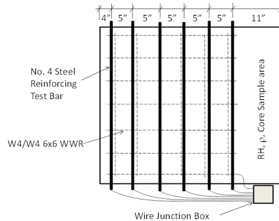
Figure 2 – Topical Treatment Test Specimen Photograph (Left) and Configuration A (Right)
