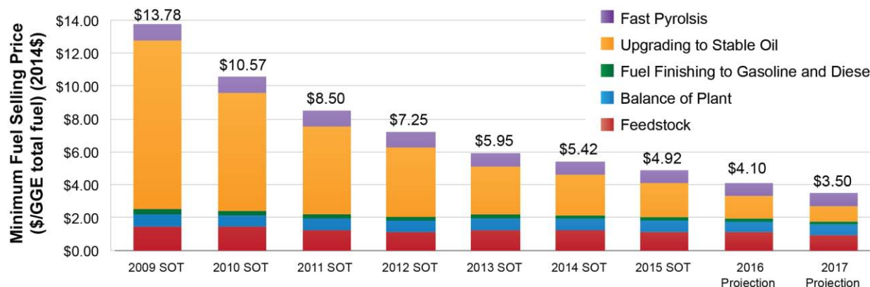
Figure 2-23: Cost projection breakdown for the fast pyrolysis design case
