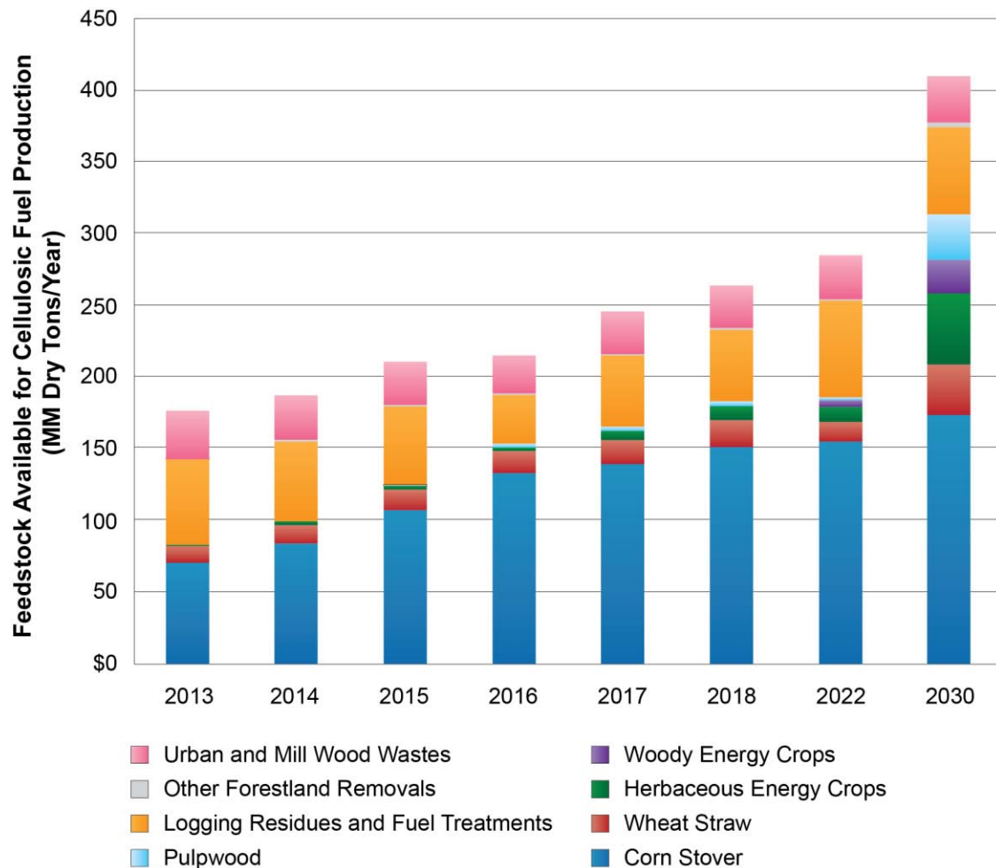
Figure 2-11: Historical and projected volumes of biomass available at a delivered cost of $84/dry ton (2014$) for various biomass types, accommodating multiple conversion processes 28
