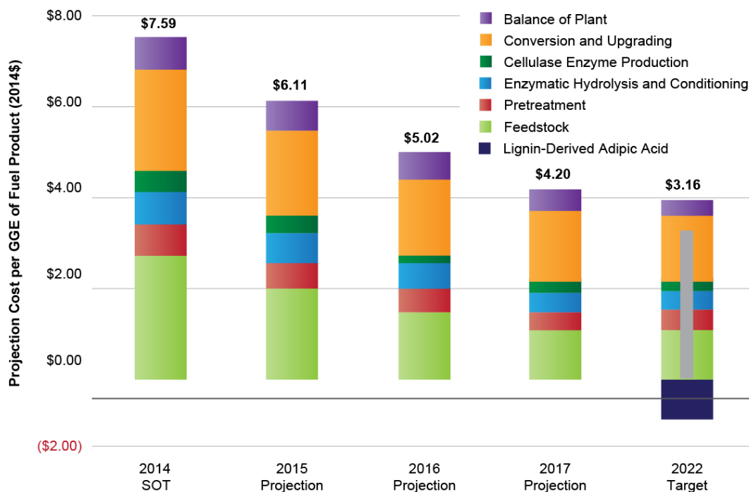
Figure 2-28: Cost projections for the low-temperature deconstruction and catalytic sugar upgrading design case
