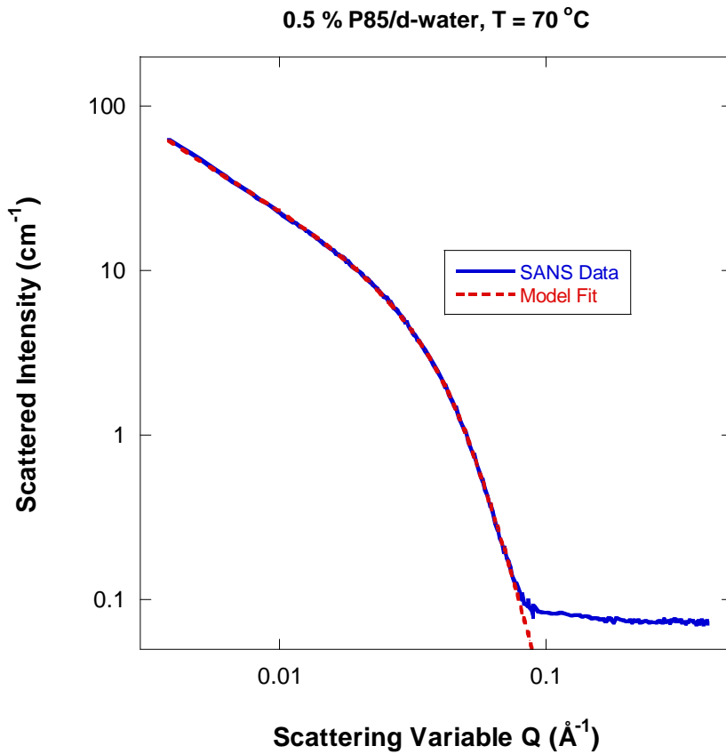
Figure 6: Fit of the generalized Guinier-Porod model to the SANS data from 0.5% P85/d-water at 70 °C where cylindrical micelles are formed.
