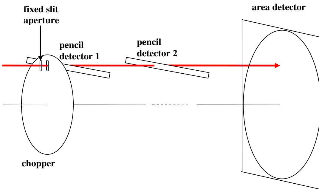
Figure 3: Schematic representation of the time-of-flight setup comprising a chopper, two pencil detectors and the area detector. The fixed slit aperture is located just before the chopper.
