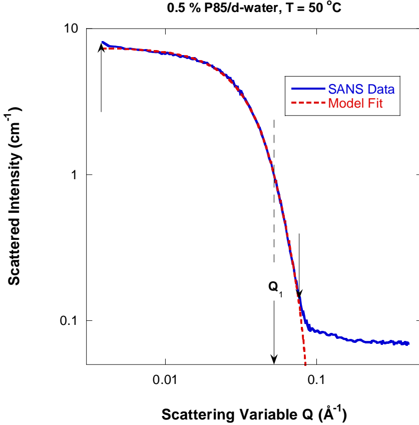
Figure 5: SANS data and fit to the Guinier-Porod model for 0.5% P85/d-water at 50 °C where spherical micelles are formed. Note that the high-Q background has been excluded from the fit. The fitting region is delimited by arrows.
