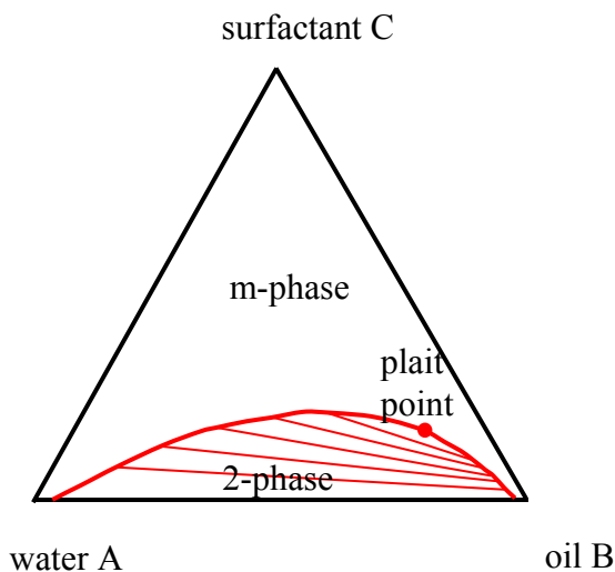
Figure 3: Schematic representation of a generic ternary mixture phase diagram. The m-phase is the micelle-formation phase.
