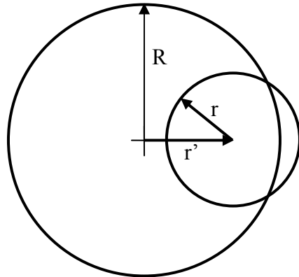
Figure 4: Representation of the geometry used to calculate the radial pair correlation function for a sphere.
