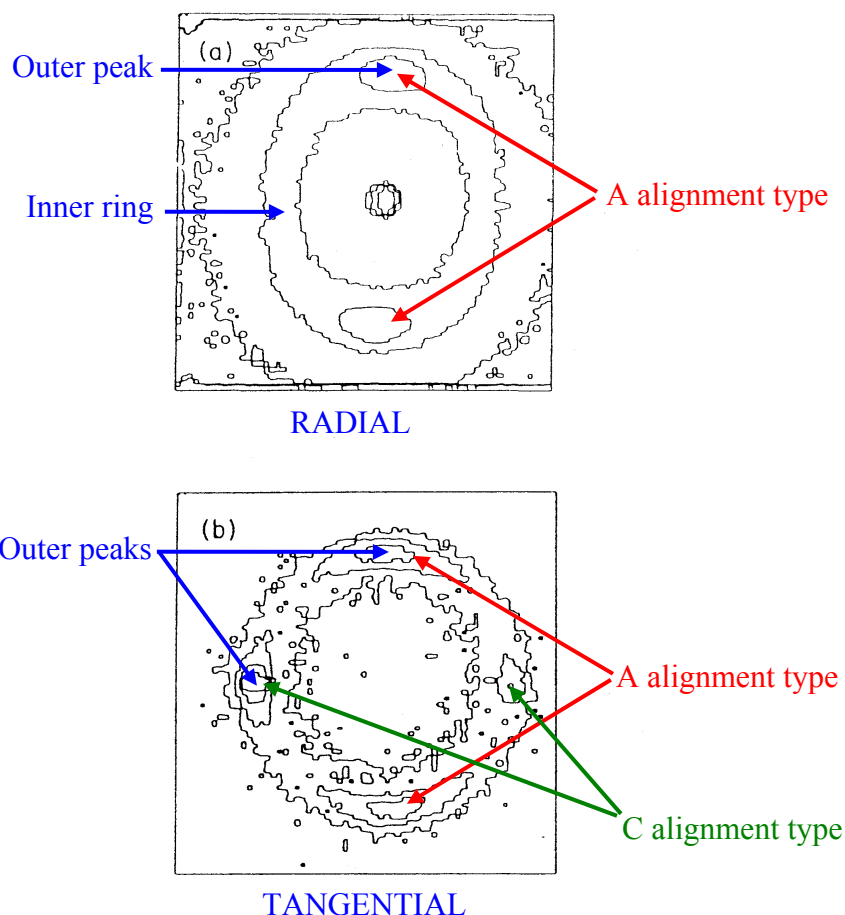
Figure 3: Iso-intensity contour plots for an oscillatory shear rate of 5835 \text{ s}^{-1} at a temperature of 49.7 \text{ }^{\circ}\text{C} (i.e., in the nematic phase) for radial (top) and tangential (bottom) beam geometries. The top contour plot shows an inner scattering ring and two outer scattering peaks in the vertical direction pointing to the A alignment type. The bottom contour plot shows four outer scattering peaks in the vertical and horizontal directions pointing to a mixture of A and C alignment types.
