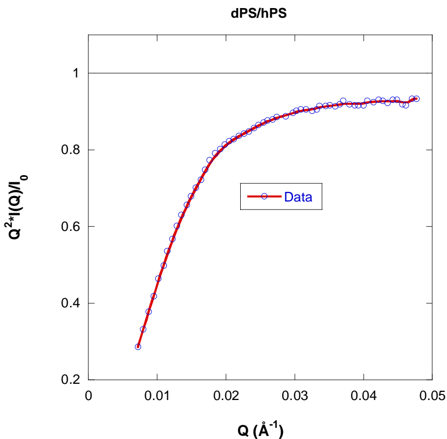
Figure 11: Kratky plot for an isotopic blend mixture of dPS and hPS with M_w = 174,000 g/mol and 195,000 g/mol, 50 % fraction (g/g) measured at ambient temperature. The line is a smoothing fit as a guide to the eye.
