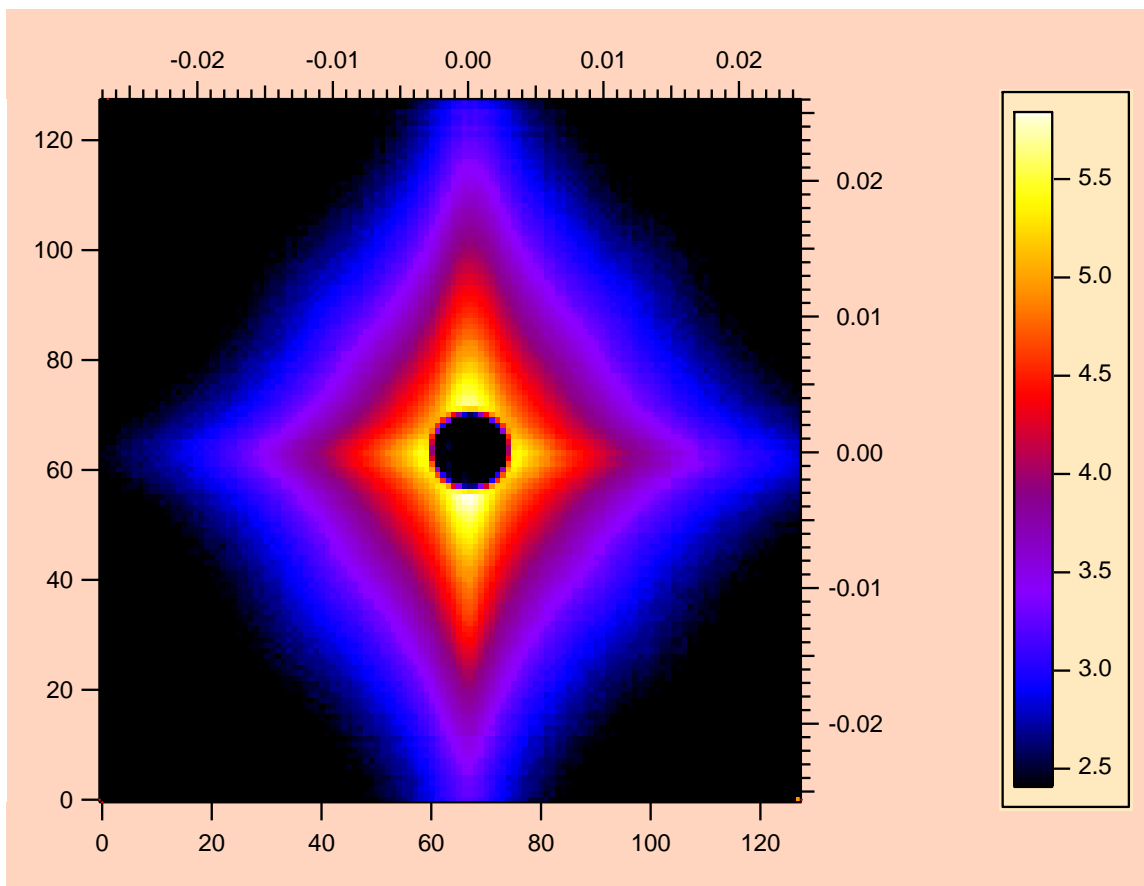
Figure 5: SANS data from the high T_c superconducting NdBa 2 Cu 3 O 7 cuprate at 100 K. Most of the scattering is due to the nuclear structure. The oriented structures characterizing the two crystals forming the twinned crystal are orthogonal (with orthorhombic symmetry) yielding the cross-like SANS patterns.
