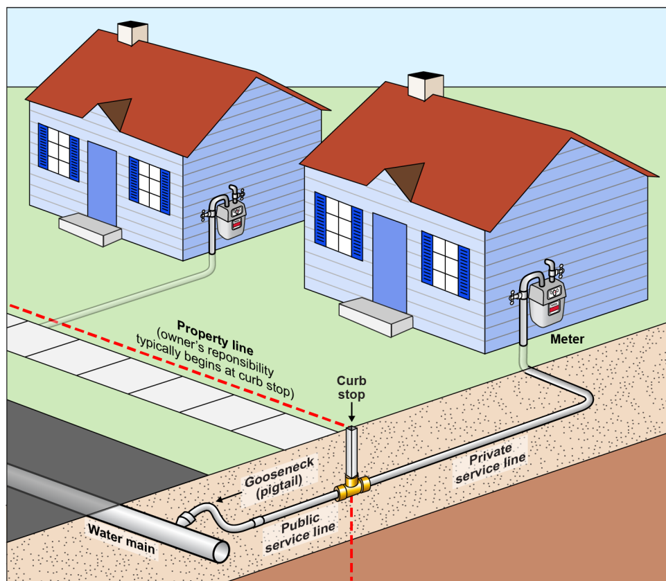
Figure 1: Typical Location of Water Main, Service Line, and Other Pipes That Deliver Drinking Water to Homes
