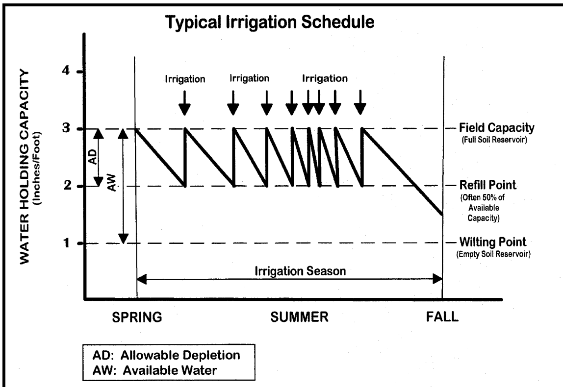
Figure 7: Irrigation Scheduling Based on Soil Moisture Status
