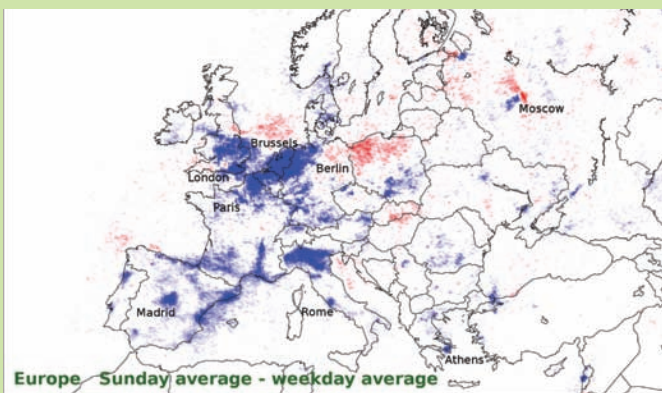
NO 2 varies with levels of human activity during the week. The maps show that on Sunday, NO 2 levels in the United States (top, left) and Europe (bottom, left) are much lower than midweek values (blue areas).
