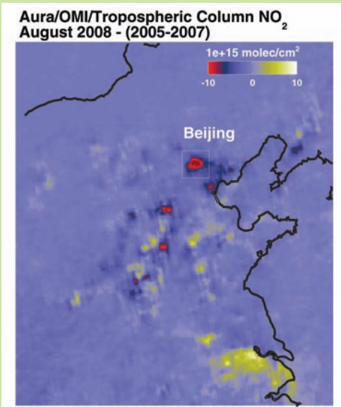
Left, map of changes in \text{NO}_2 for August compared to previous years. Above, monthly mean \text{NO}_2 amounts over Beijing compared with previous years. Emission controls applied during the Beijing Olympic Games reduced this pollutant.
