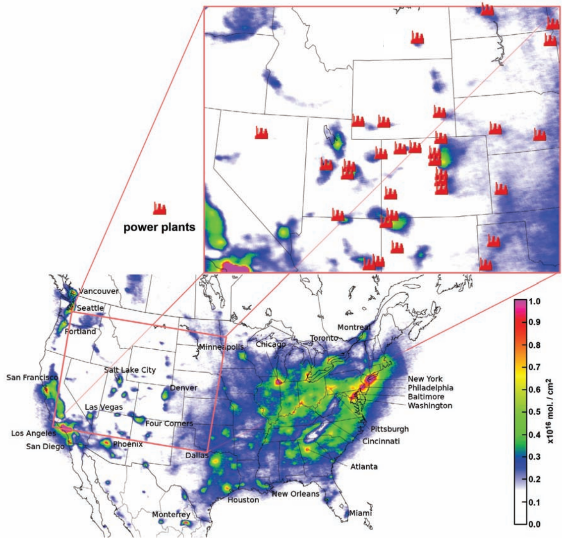
The maps of the tropospheric column of NO 2 produced by the OMI team give us a clear picture of industrial and agricultural activity across the globe. The inset
