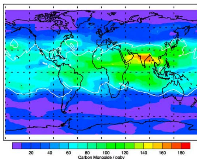
Figure 5. CO measured by MLS at 147 hPa (upper troposphere in the tropics, lower stratosphere at mid- and high-latitudes) for 30 August 2004. White curves are contours of potential vorticity ( \pm 2.0 \times 10^{-6} \text{ K m}^2 \text{ kg}^{-1} \text{ s}^{-1} ) defining the dynamical tropopause.
