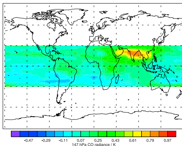
Figure 7. Tropical 147 hPa CO radiance measured by MLS for 30 August 2004. The specific analysis used to derive this radiance is only valid in the tropical troposphere. Range in values corresponds approximately to 0–180 ppbv retrieved CO.
