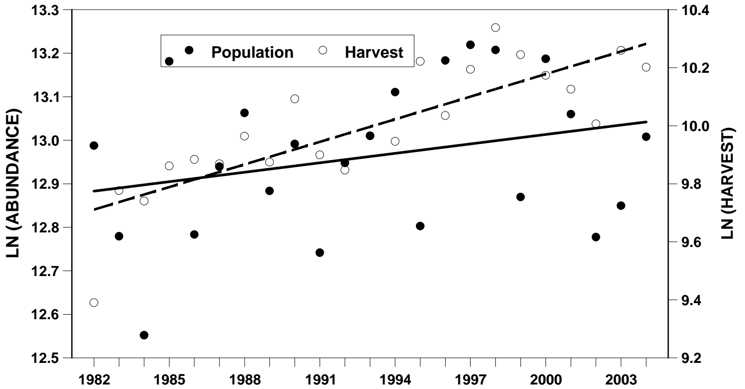
Figure 15. Trend analyses of indices to abundance and harvest of Mid-Centroid sandhill cranes
