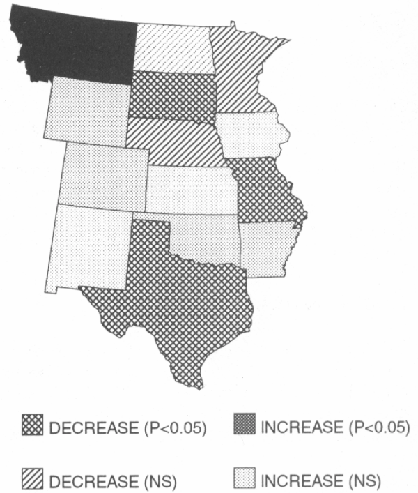
Fig. 9. Trends in number of mourning doves heard per route by state in the Central Management Unit, 1991-2000.
