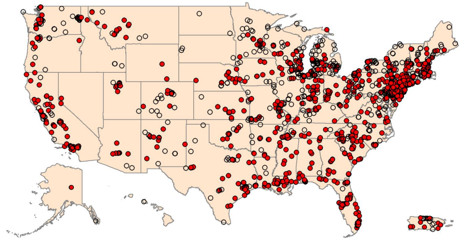
Nonfederal NPL Sites Located in Areas that May Be Impacted by Flooding, Storm Surge, Wildfires, or Sea Level Rise
