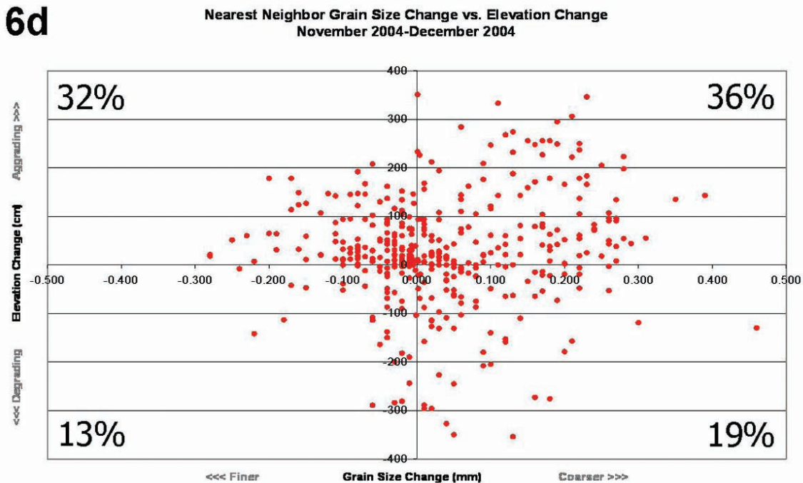
Figure 6. (continued) Plots from the nearest neighbor analysis for each survey interval showing relations between changes in riverbed elevation and bed-surface grain size. During the first two intervals, there were minimal tributary sand inputs and coarsening dominated, but during the third interval, there were large tributary sand inputs and fining and aggradation were more prevalent. During the 2004 beach/habitat-building flows (BHBF) experiment (interval 4), the large number of points that aggraded can be largely attributed to collection methods that emphasized eddy sandbars, although the trend toward coarsening can only be attributed to the winnowing effects of the higher flow.
