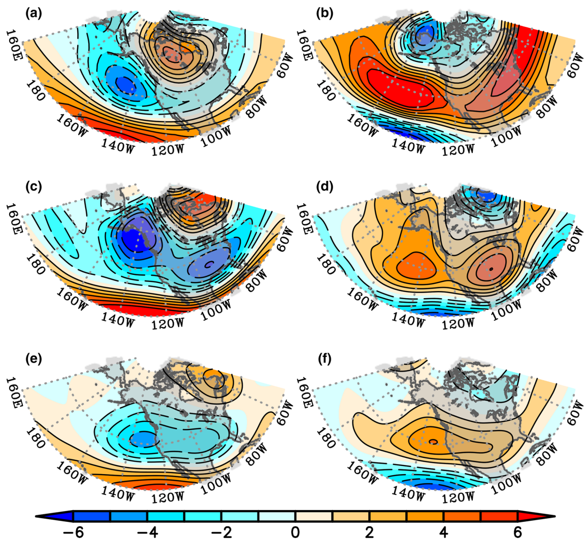
Fig. 14 Composite of 200 hPa streamfunction anomaly ( 10^6 \text{ s}^{-1} ) for boreal winters (DJF) during El Niño events: observed (a), HRCTL (c), and HRIE (e). Similarly, for La Niña events: observed (b), HRCTL (d), and HRIE (f)
