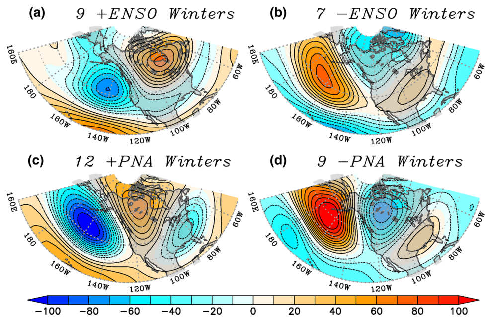
Fig. 1 Composite of 200 hPa geopotential height anomaly during DJF for warm ENSO events (a), cold ENSO events (b), warm PNA winters (c), and cold PNA winters (d). Contour interval is 10 m. The number in each sub-title corresponds to the number of events in the composite
