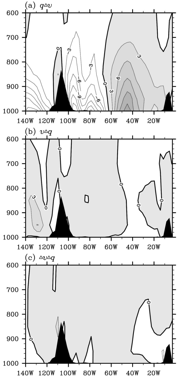
FIG. 12. Meridional moisture transport difference ( \text{g kg}^{-1} \text{ m s}^{-1} ) between the CTRL and NO_AWP runs at 30°N during September–October (SO) contributed by (a) the meridional wind change q\Delta v , (b) the specific humidity change v\Delta q , and (c) the product of the meridional wind and specific humidity changes \Delta v\Delta q . \Delta v ( \Delta q ) represents the meridional wind (specific humidity) difference between the CTRL and NO_AWP runs. The unit on the vertical axis is mb. The positive moisture transport difference is shaded and the contour interval is 3 \text{ g kg}^{-1} \text{ m s}^{-1} .
