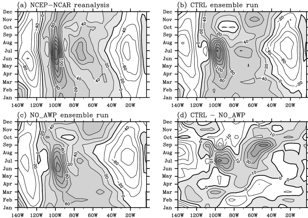
FIG. 10. Time-longitude sections of the vertically integrated meridional moisture transport [\int_{300\text{mb}}^{\text{sfc}}(qv/g) dp; \text{kg m}^{-1} \text{s}^{-1}] at 30°N from (a) the NCEP-NCAR reanalysis, (b) the CTRL ensemble run, (c) the NO_AWP ensemble run, and (d) the difference between the CTRL and NO_AWP runs. In (a)–(c), the northward moisture transport is shaded and the contour interval is 20 \text{kg m}^{-1} \text{s}^{-1} . In (d), the positive moisture transport is shaded and the contour interval is 10 \text{kg m}^{-1} \text{s}^{-1} .
