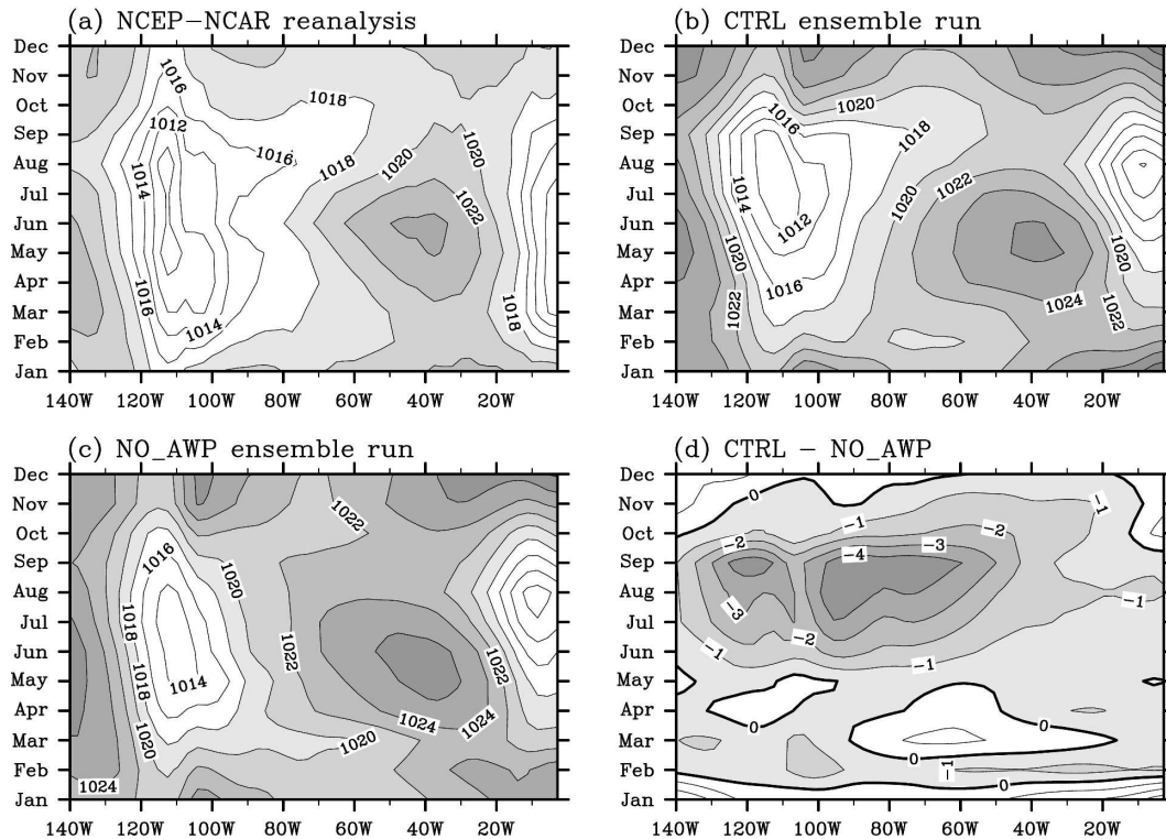
FIG. 3. Time-longitude sections of SLP (mb) at 30°N from (a) the NCEP-NCAR reanalysis, (b) the CTRL ensemble run, (c) the NO_AWP ensemble run, and (d) the difference between the CTRL and NO_AWP runs. In (a)–(c), the SLP higher than 1018 mb is shaded and the contour interval is 2.0 mb. In (d), the negative SLP difference is shaded and the contour interval is 1.0 mb.
