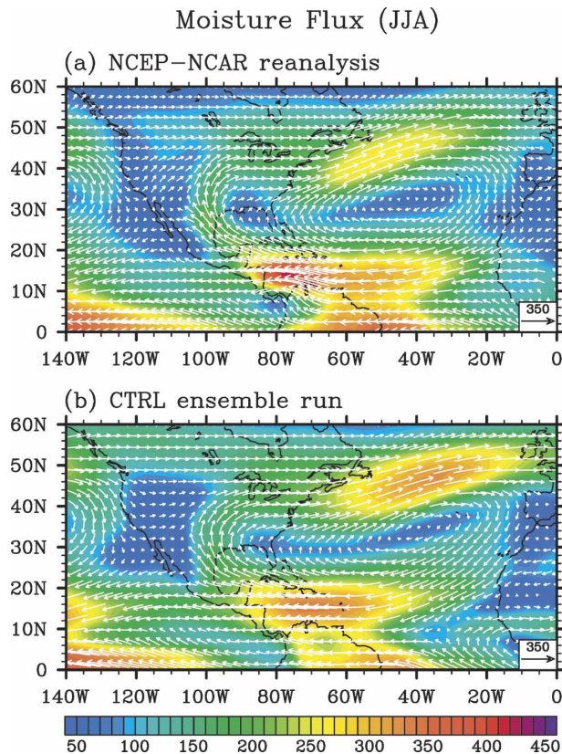
FIG. 4. Summer (JJA) vertically integrated moisture flux [ \mathbf{Q} = \int_{300\text{mb}}^{\text{stc}} (q\mathbf{u}/g) dp , where q is specific humidity, \mathbf{u} is vector wind, p is pressure, and g is gravity; in unit of \text{kg m}^{-1} \text{s}^{-1} ] calculated from (a) the NCEP-NCAR reanalysis and (b) the CTRL ensemble run. Arrows indicate the moisture flux vector and colors represent the amplitude of the moisture flux.
