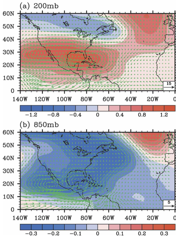
FIG. 18. Geopotential height ( 10^2 m) and wind ( \text{m s}^{-1} ) difference between the CTRL and NO_AWP runs during ASO at (a) 200 and (b) 850 mb.
