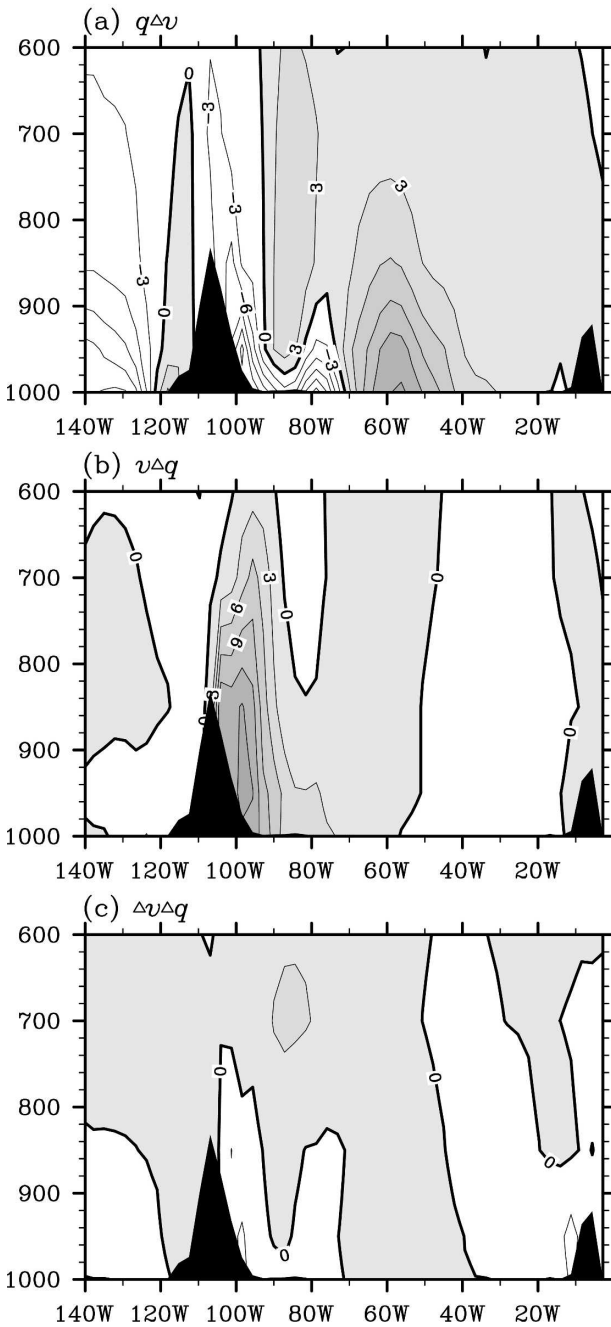
FIG. 11. Meridional moisture transport difference ( \text{g kg}^{-1} \text{ m s}^{-1} ) between the CTRL and NO_AWP runs at 30°N during JJA contributed by (a) the meridional wind change q\Delta v , (b) the specific humidity change v\Delta q , and (c) the product of the meridional wind and specific humidity changes \Delta v\Delta q . \Delta v ( \Delta q ) represents the meridional wind (specific humidity) difference between the CTRL and NO_AWP runs. The unit on the vertical axis is mb. The positive moisture transport difference is shaded and the contour interval is 3 \text{ g kg}^{-1} \text{ m s}^{-1} .
