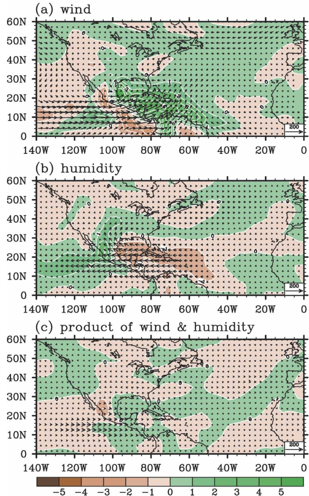
FIG. 16. The moisture convergence (contour; \text{mm day}^{-1} ) and transport (vector; \text{kg m}^{-1} \text{ s}^{-1} ) difference between the CTRL and NO_AWP runs during JJA contributed by (a) the wind change -\nabla \cdot [\int_{300\text{mb}}^{\text{sfic}} (q\Delta\mathbf{u}/g) dp] and \int_{300\text{mb}}^{\text{sfic}} (q\Delta\mathbf{u}/g) dp , (b) the specific humidity change -\nabla \cdot [\int_{300\text{mb}}^{\text{sfic}} (\mathbf{u}\Delta q/g) dp] and \int_{300\text{mb}}^{\text{sfic}} (\mathbf{u}\Delta q/g) dp , and (c) the product of the wind and specific humidity changes -\nabla \cdot [\int_{300\text{mb}}^{\text{sfic}} (\Delta q\Delta\mathbf{u}/g) dp] and \int_{300\text{mb}}^{\text{sfic}} (\Delta q\Delta\mathbf{u}/g) dp . \Delta\mathbf{u}(\Delta q) represents the wind vector (specific humidity) difference between the CTRL and NO_AWP runs.
