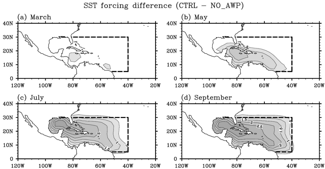
FIG. 1. SST forcing difference between the CTRL and NO_AWP model runs in (a) March, (b) May, (c) July, and (d) September. The SST difference larger than 0.5^{\circ}\text{C} is shaded. The AWP box (from 5^{\circ} to 30^{\circ} between 40^{\circ}\text{W} and the coast of the Americas) is marked.
