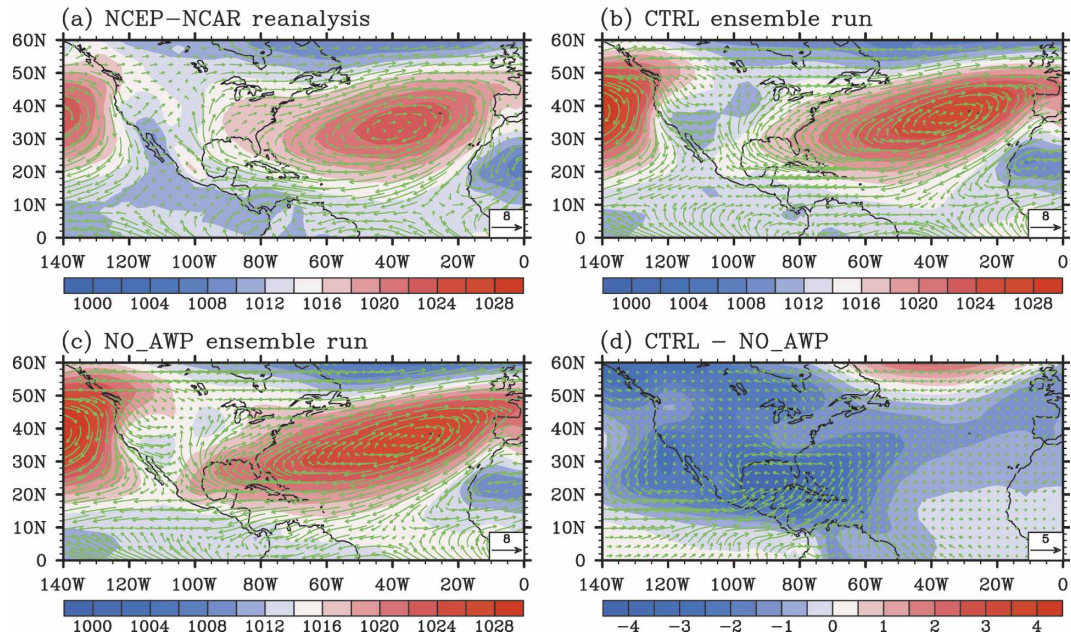
FIG. 2. Horizontal structure of SLP (mb) and the 925-mb wind vector ( \text{m s}^{-1} ) during the summer (JJA) from (a) the NCEP-NCAR reanalysis, (b) the CTRL ensemble run, (c) the NO_AWP ensemble run, and (d) the difference between the CTRL and NO_AWP runs.
