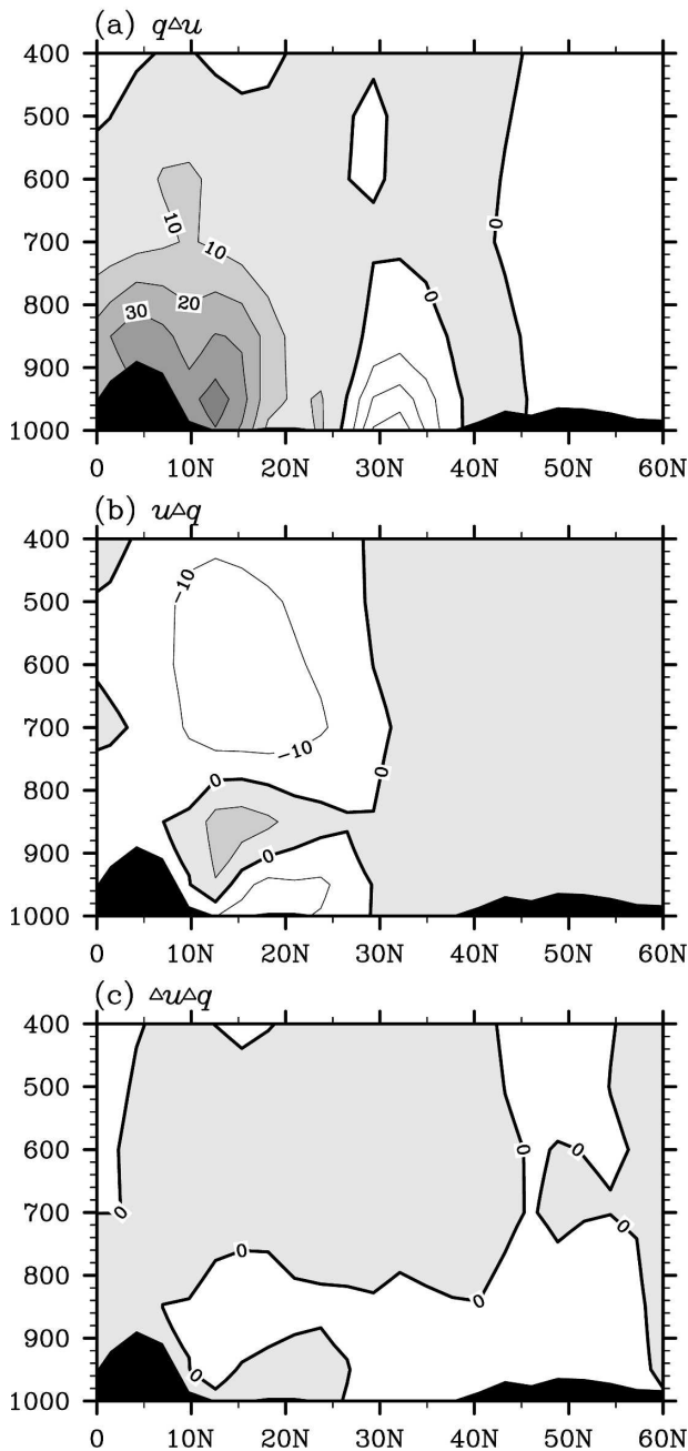
FIG. 6. Zonal moisture transport difference ( \text{g kg}^{-1} \text{m s}^{-1} ) between the CTRL and NO_AWP runs at 75°W during the summer (JJA) contributed by (a) the zonal wind change q\Delta u , (b) the specific humidity change u\Delta q , and (c) the product of the zonal wind and specific humidity changes \Delta u\Delta q . Here \Delta u ( \Delta q ) represents the zonal wind (specific humidity) difference between the CTRL and NO_AWP runs. The unit on the vertical axis is mb. The positive moisture difference is shaded and the contour interval is 10 \text{ g kg}^{-1} \text{m s}^{-1} .
