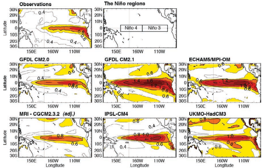
FIG. 4. SST std dev (°C) for 100 yr of monthly data for models in Fig. 3b. Observations are taken from HadISST1.1 (1900–99). The location of the Niño regions discussed in the text is also shown.
