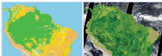
Two ways Dr. Papeş uses MODIS data to look at vegetation. Left image is combined Terra and Aqua MODIS Land Cover Type (MCD12Q1) with colors representing land cover type based on the International Geosphere-Biosphere Programme (IGBP) classification scheme (e.g., green represents broadleaf forest vegetation, yellow represents croplands, and red represents urban/built-up areas). Right image is a Terra MODIS Enhanced Vegetation Index (EVI; MOD13Q1) showing areas with high biomass (dark green areas) and areas with low biomass (brown areas). Both images show land cover type and vegetation as of January 1, 2018. NASA Worldview images.
