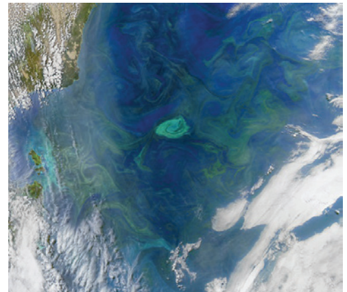
Blooms of phytoplankton are clearly seen as blue/green swirls of color in this Aqua/MODIS image of the Tasman Sea off the south coast of Australia acquired on November 1, 2019. NASA image available through the NASA Ocean Color Image Gallery.
