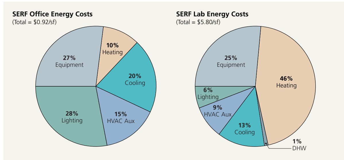
Annual predicted area normalized energy cost for SERF base-case building.
