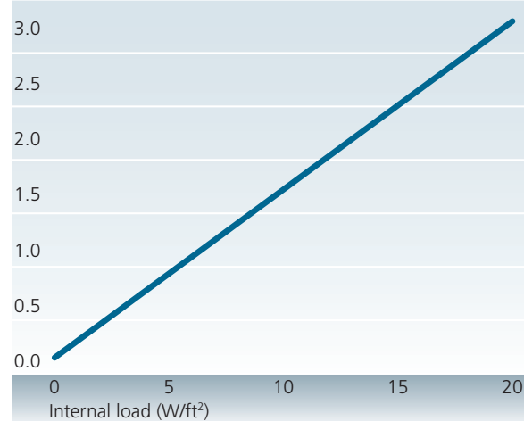
Quantity of 55°F supply air required to offset internal loads.
