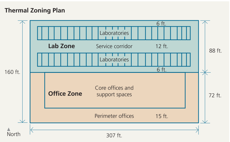
Simple base-case building schematic of the SERF. Designers described two zones, an office zone and a lab zone, to evaluate the very different load profiles for those major functions.
