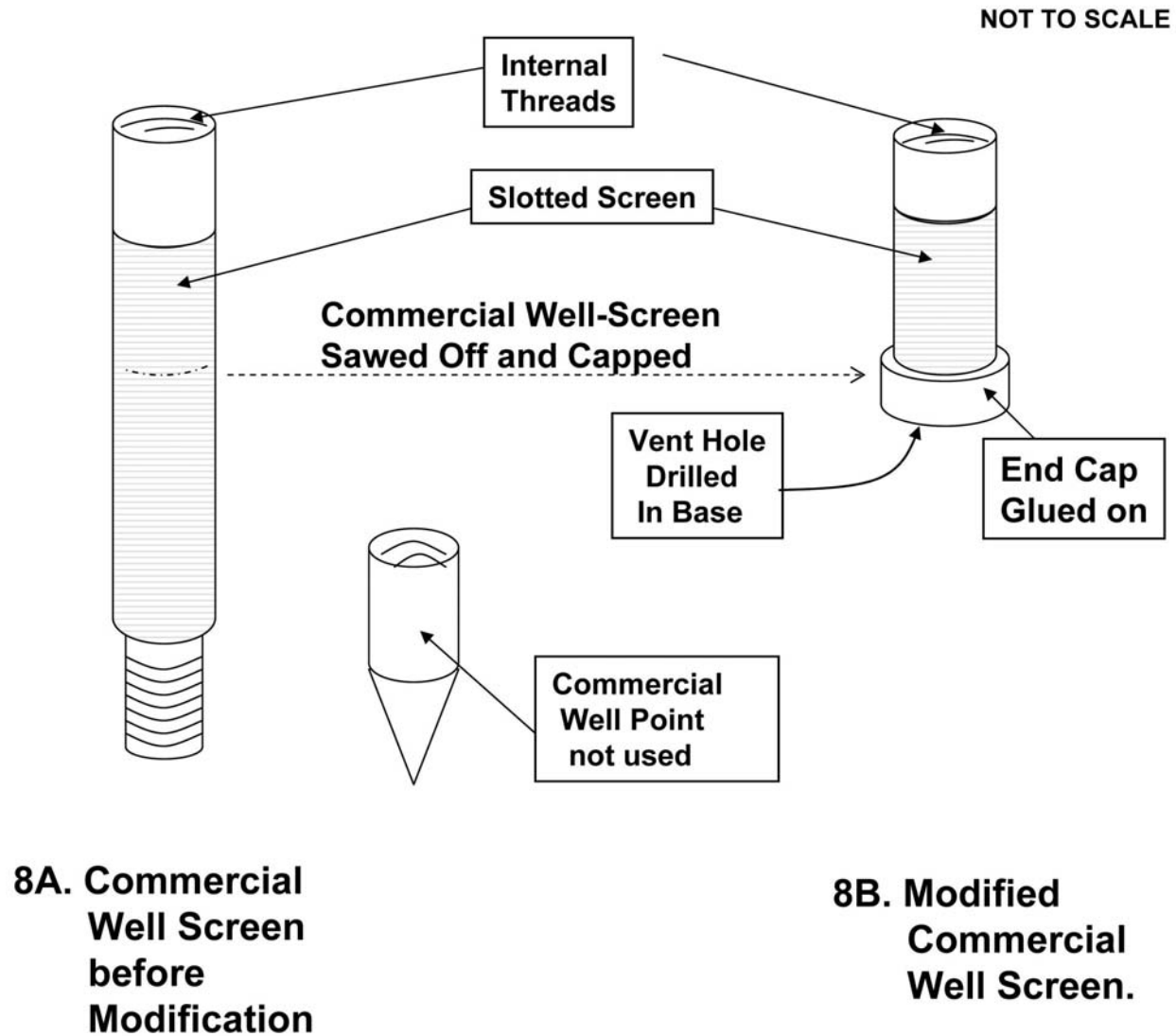
Figure 8. Modified commercial well screen. (8A) Commercial well screen with threads at both top and bottom. (8B) Screen after sawing off lower threaded portion of pipe and closing with vented PVC plug. Figure modified from Miner and Simon (1997).
