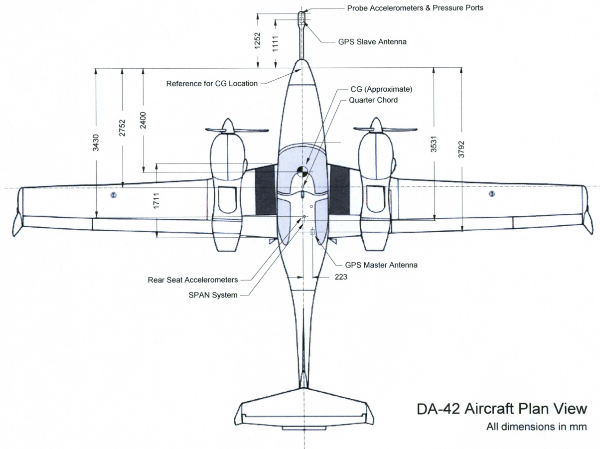
Figure 10. DA-42 GPS/INS configuration.
