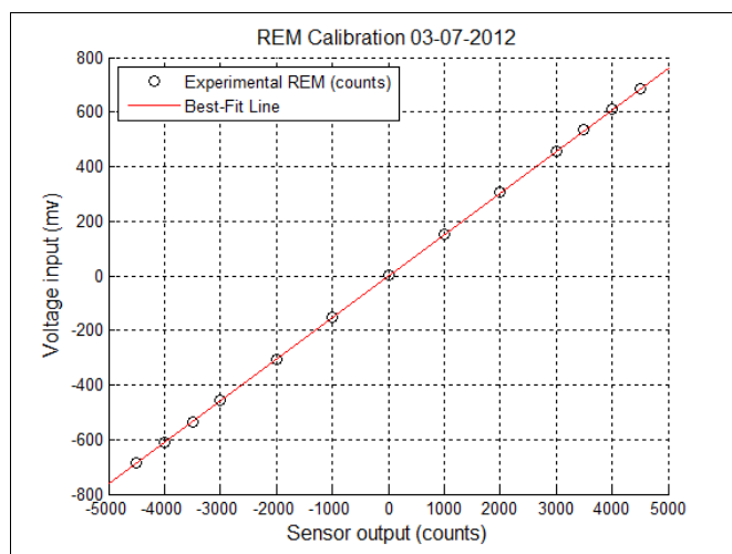
Figure 15. BAT-REM Calibration Data.
