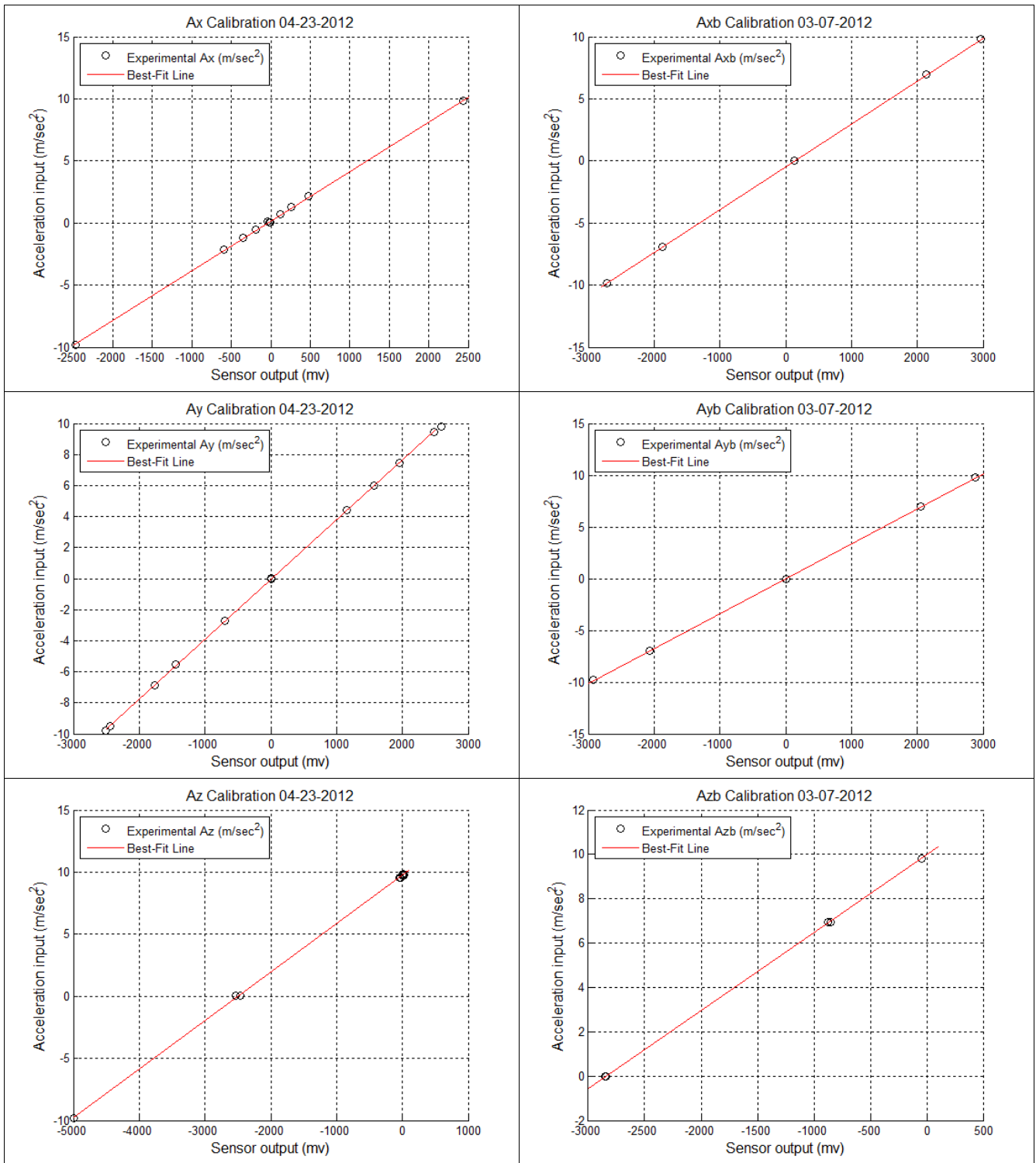
Figure 7. Accelerometer calibration data for Ax, Axb, Ay, Ayb, Az, Azb.
