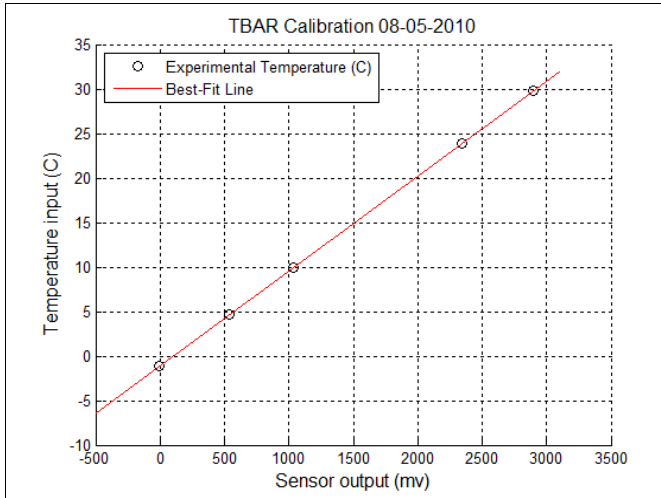
Figure 11. TBar calibration data.
