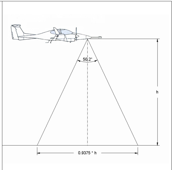
Figure 14. Canon Powershot G15 profile view of camera viewing angle from the DA-42.
