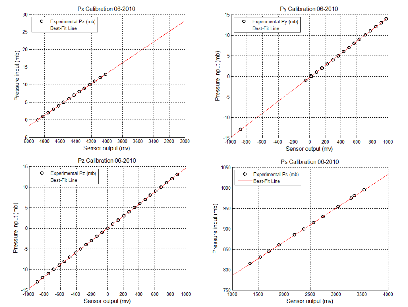
Figure 6. Pressure calibration data for Px, Py, Pz, and Ps.
