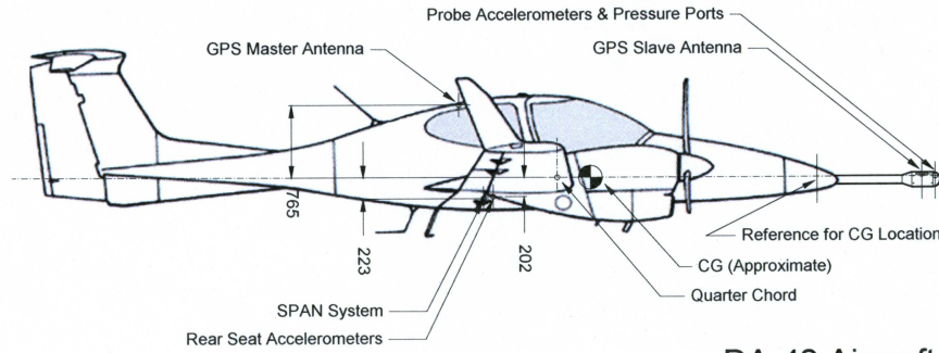
DA-42 Aircraft Side View
