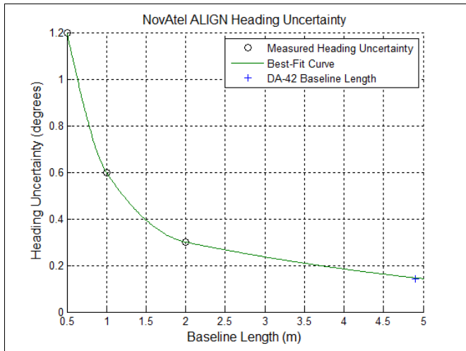
Figure 9. NovAtel ALIGN heading uncertainty.
