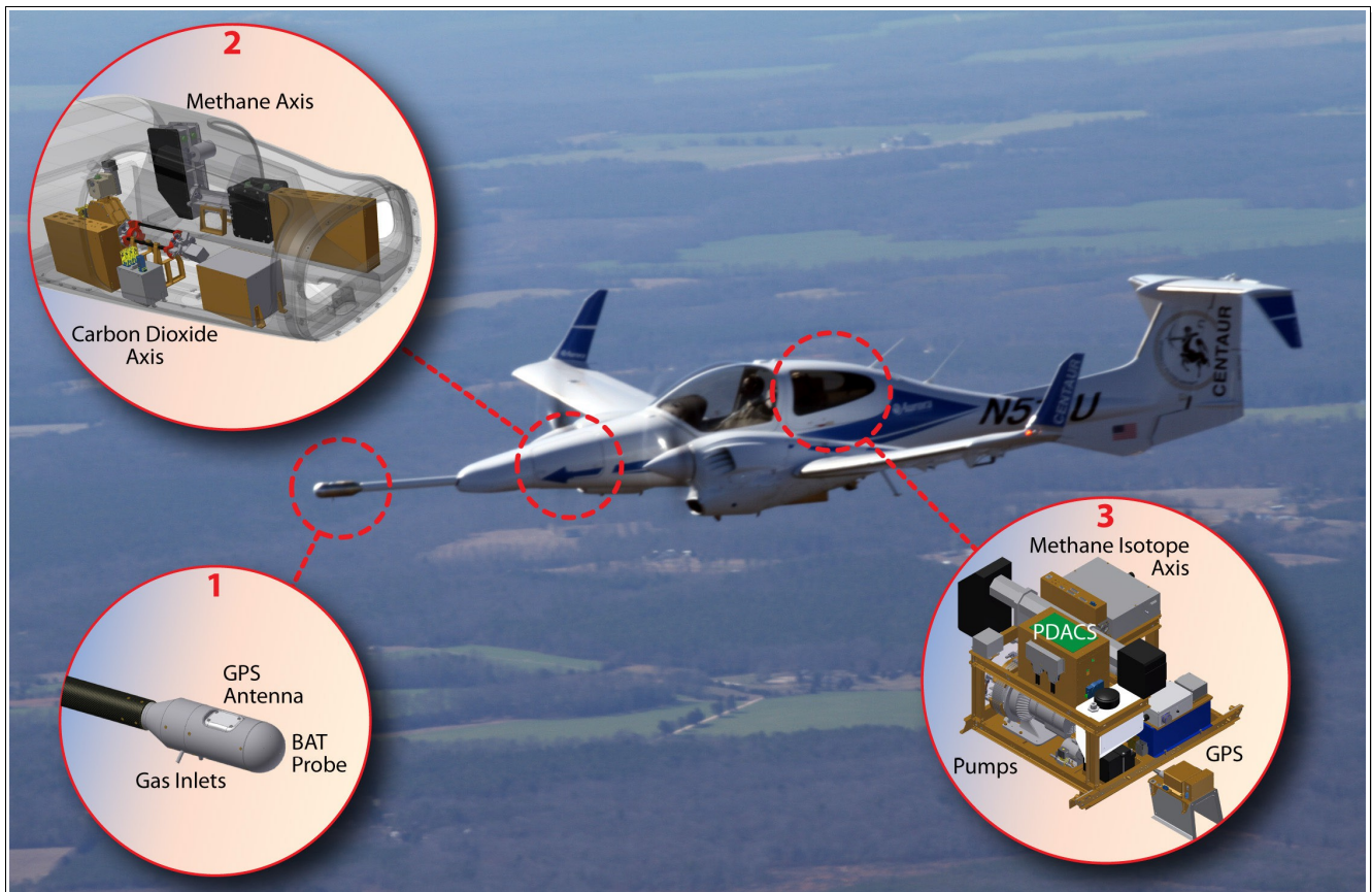
Figure 4. Diagram of the Harvard gas analyzer instruments and the ATDD BAT probe.
