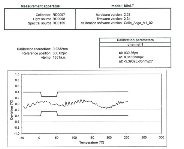
Figure 12. Fiber-optic temperature sensor calibration data.
