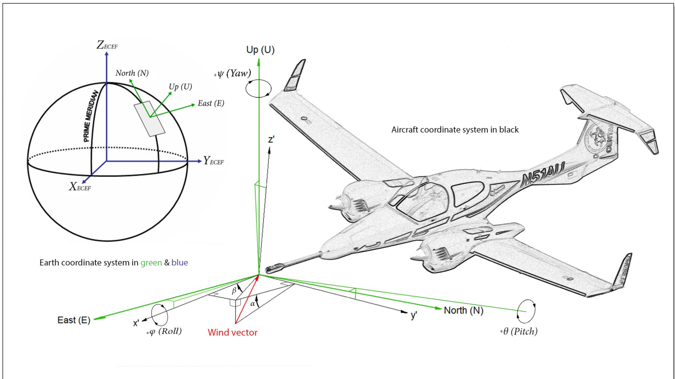
Figure 5. Diagram of Earth coordinate system and aircraft coordinate system.
