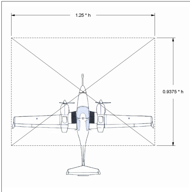
Figure 13. Canon Powershot G15 plan view of camera viewing angle from the DA-42.
