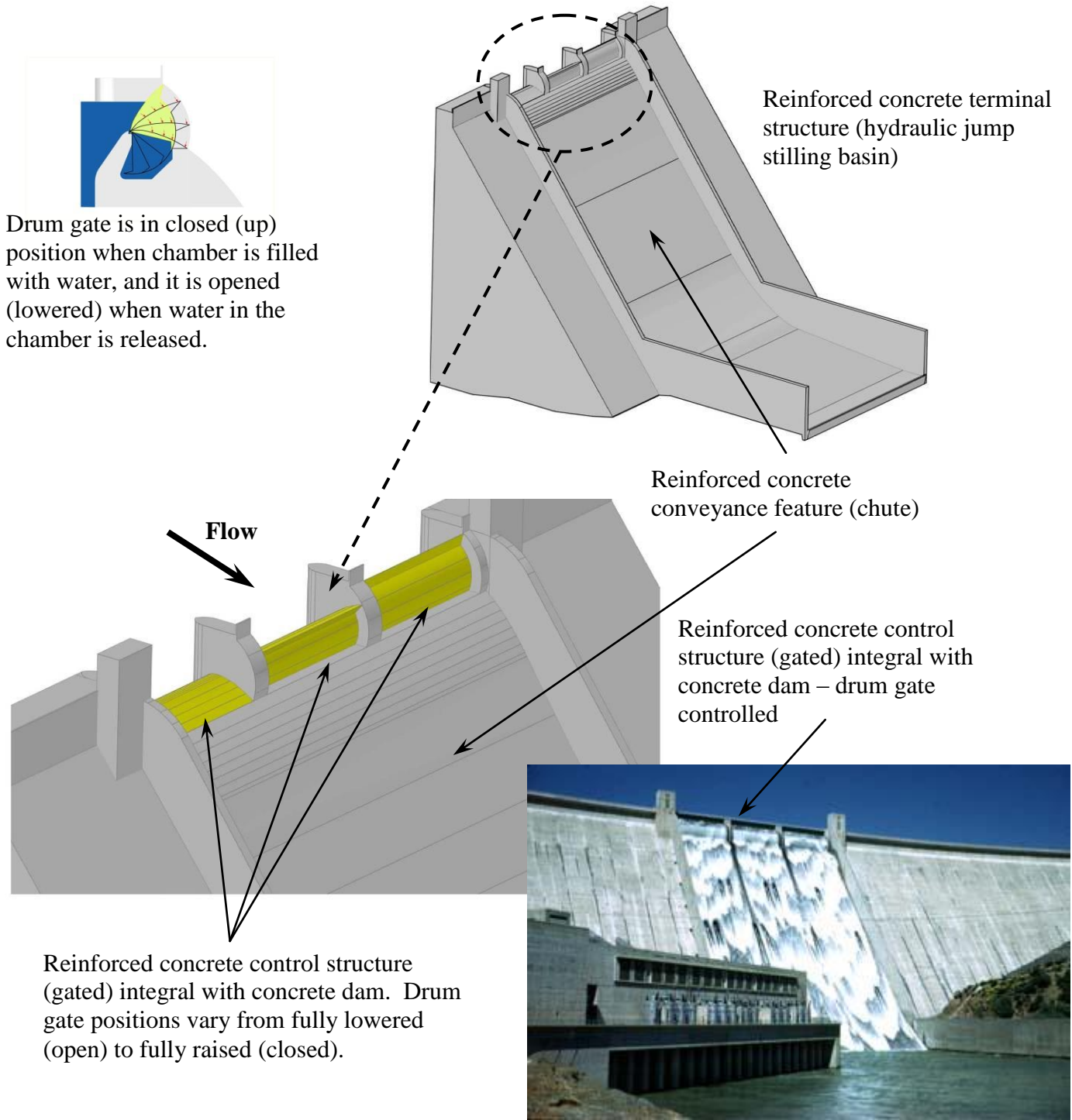
Gated service spillway integral with concrete dam, Shasta Dam, California
