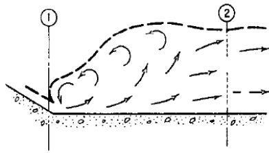
Type I – Hydraulic jump, horizontal apron
