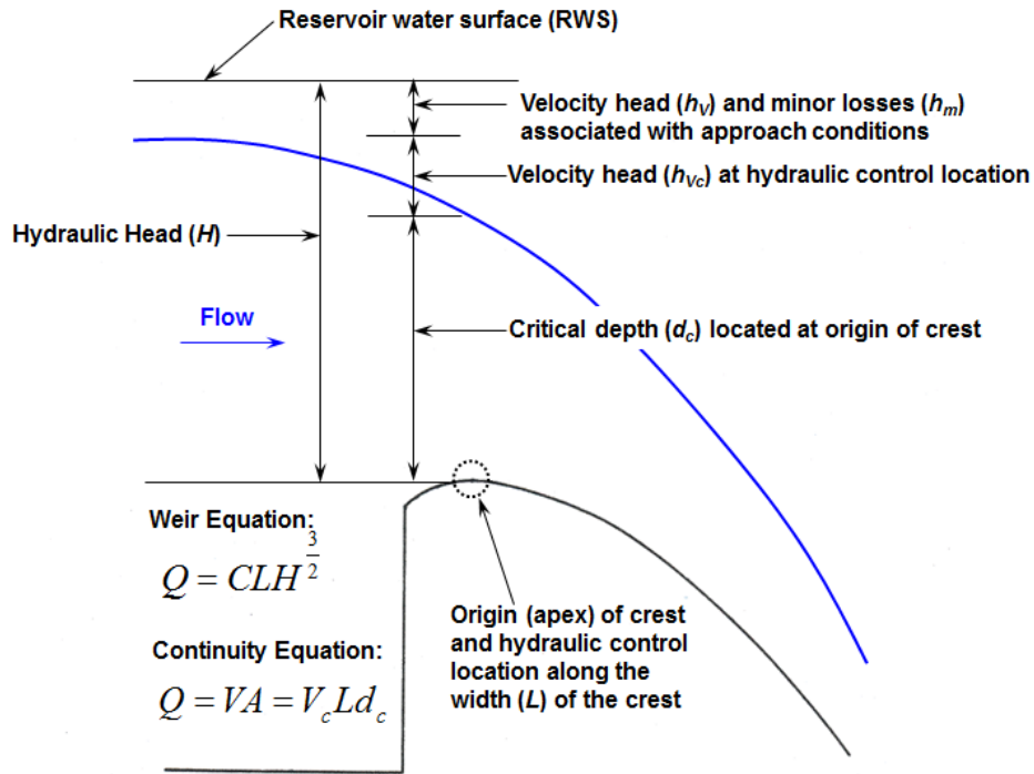
Figure 3.6.1.1-1. Crest control.
