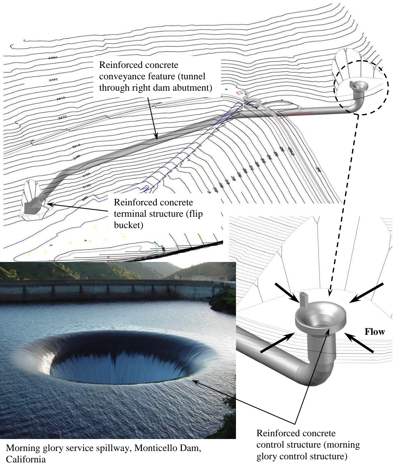
Figure 3.5.2.1-4. Drop inlet (morning glory) spillway.
