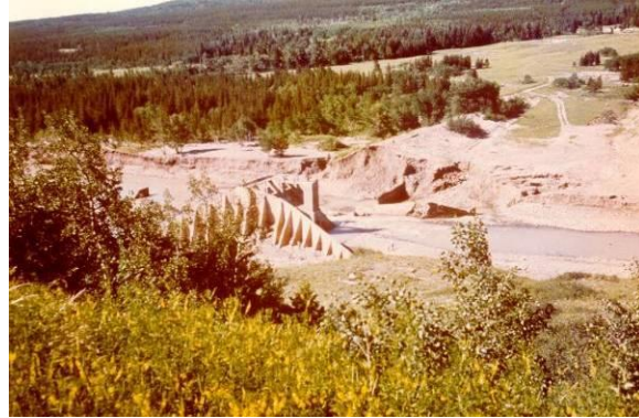
1964 Dam Remnant after Flood-induced Overtopping Failure – Lower Two Medicine Dam, Montana.
