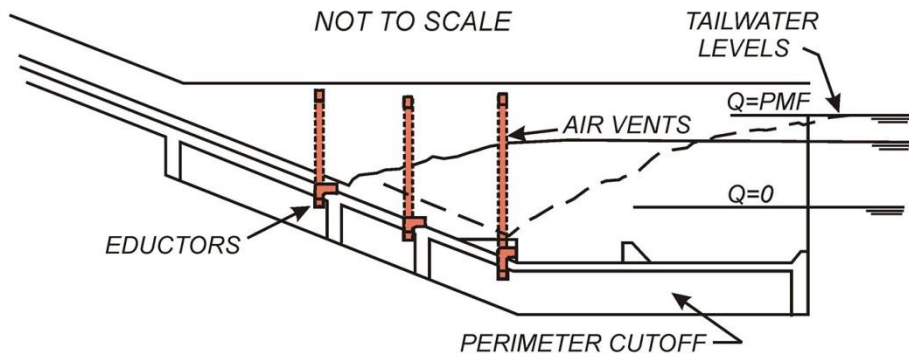
Figure 3.7.3.1-4. Air supply/demand.
