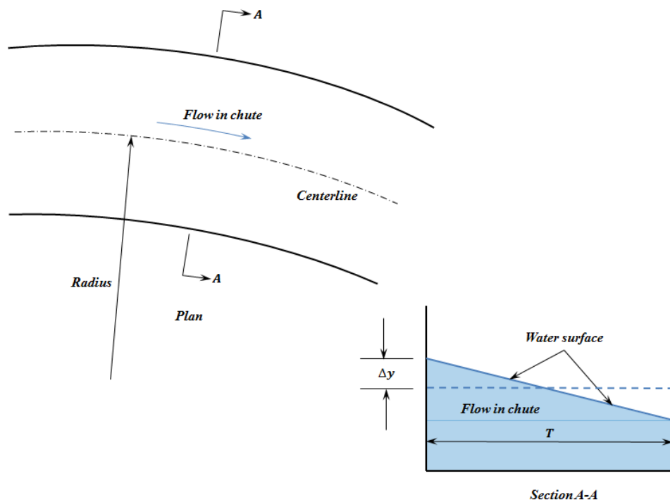
Figure 3.6.4.1.4-2. Superelevation illustration.
