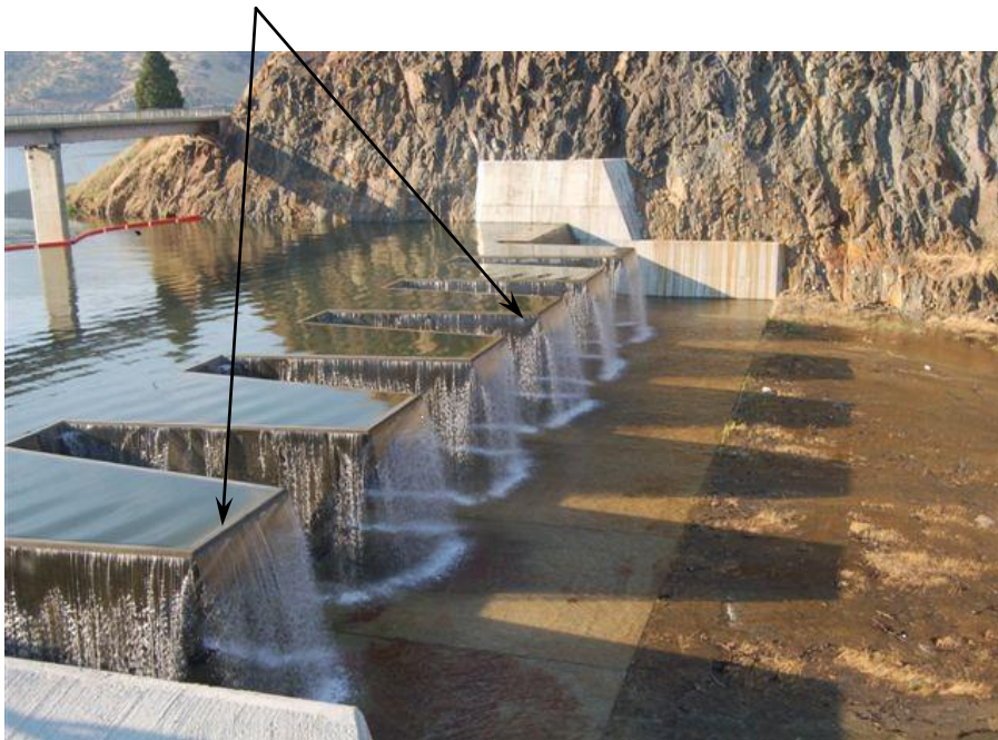
Fusegate spillway, Terminus Dam, California (courtesy of the U.S. Army Corps of Engineers, Sacramento District, Rick Poepelman).
