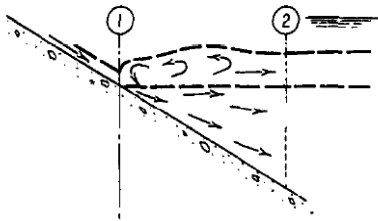
Type V – Hydraulic jump, sloping apron
