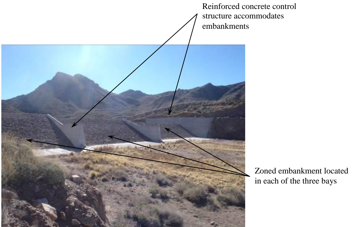
Three segment fuseplug auxiliary spillway, Reclamation dam
