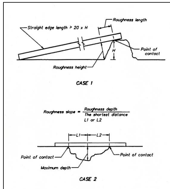
Figure 3.8.6.3-2. Measuring surface roughnesses.
