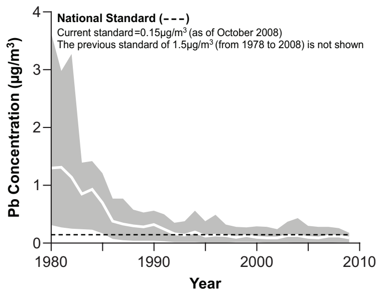
Figure 3.4: U.S. Pb Air Concentration From 1980-2009
