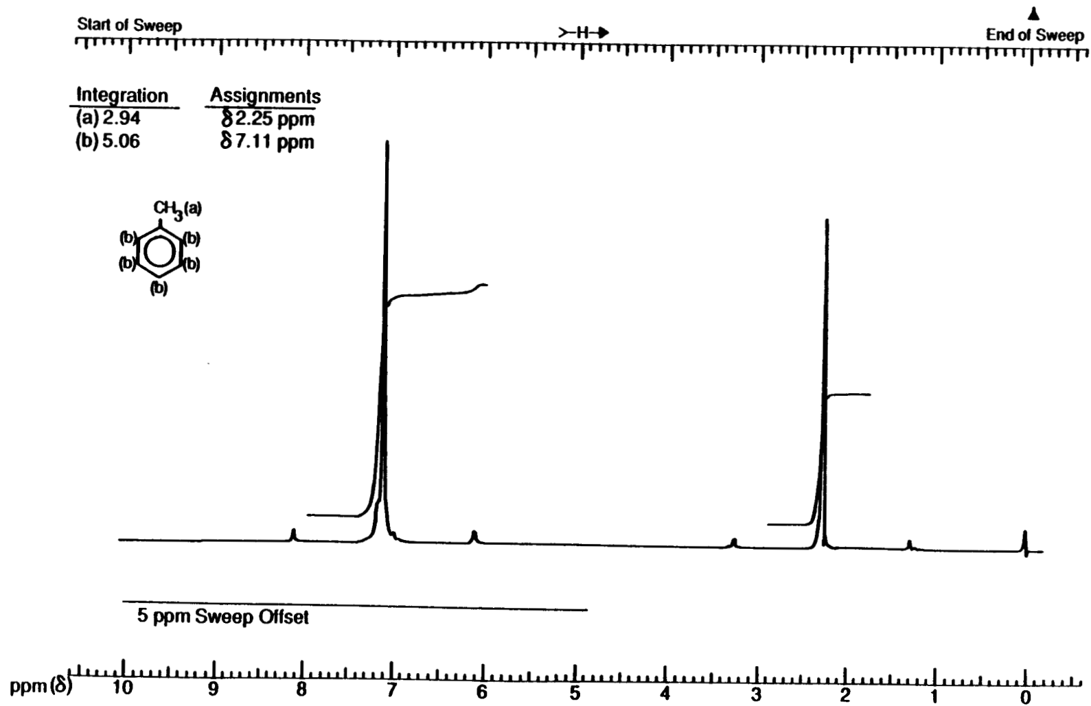
FIGURE 12. NUCLEAR MAGNETIC RESONANCE SPECTRUM OF TOLUENE (LOT NO. H-12-19-80)
