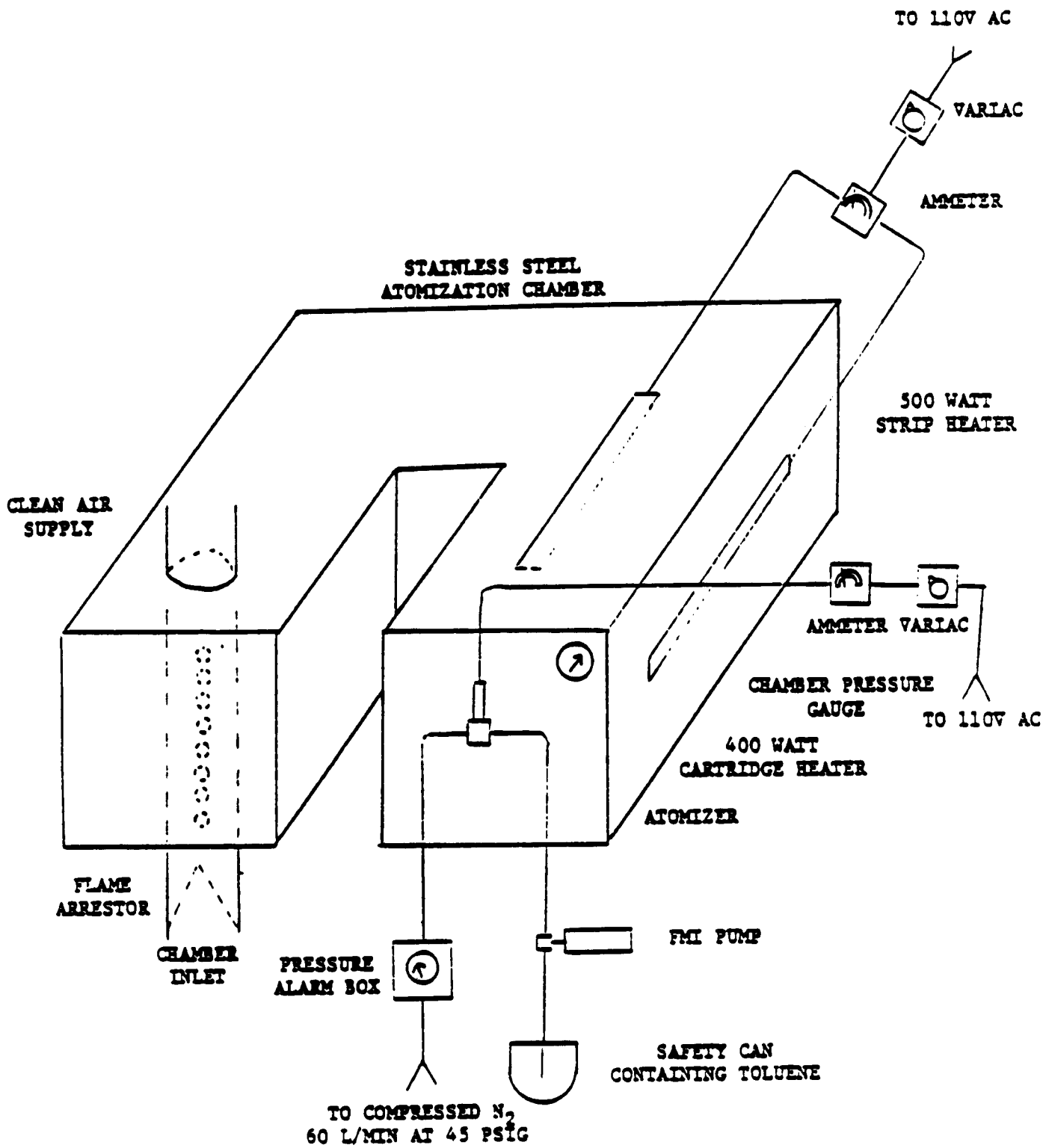
FIGURE 13. TOLUENE VAPOR GENERATION SYSTEM
