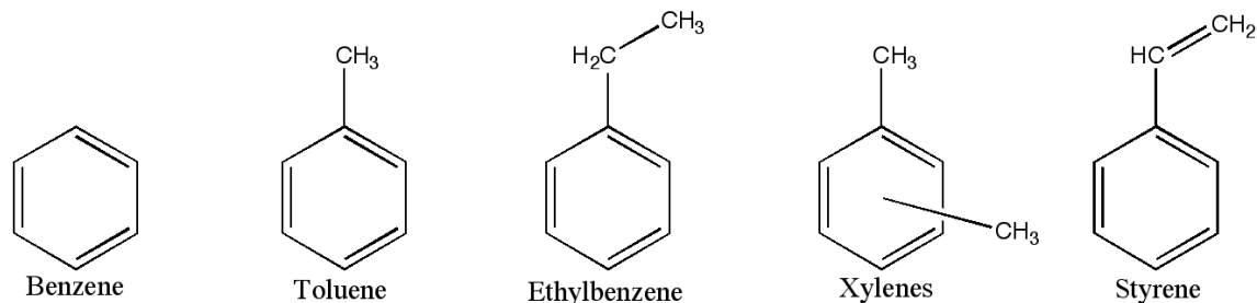
Figure 1-2. Chemical structure of cumene analogues
