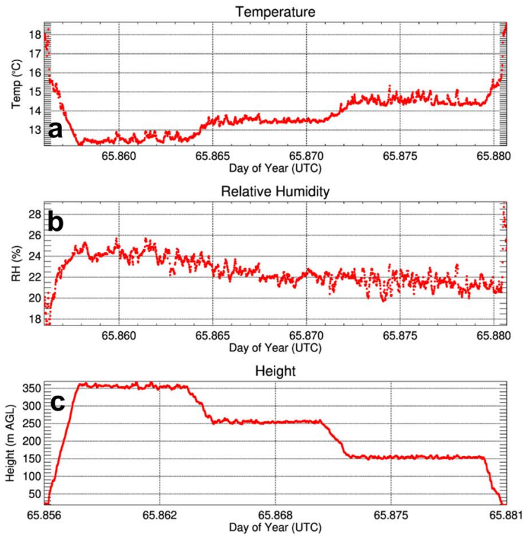
Figure 8: Temperature (a), humidity (b), and height AGL (c) during the BST S2 flight on 6 March 2019 between 20:32 and 21:07 UTC.
