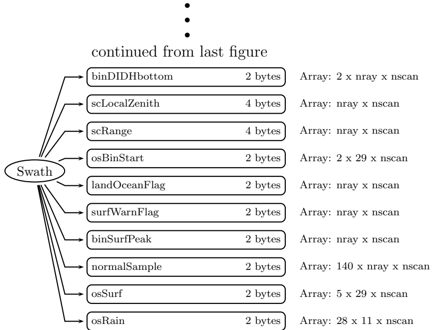
Figure 22: Data Format Structure for 1C21, PR Reflectivities
