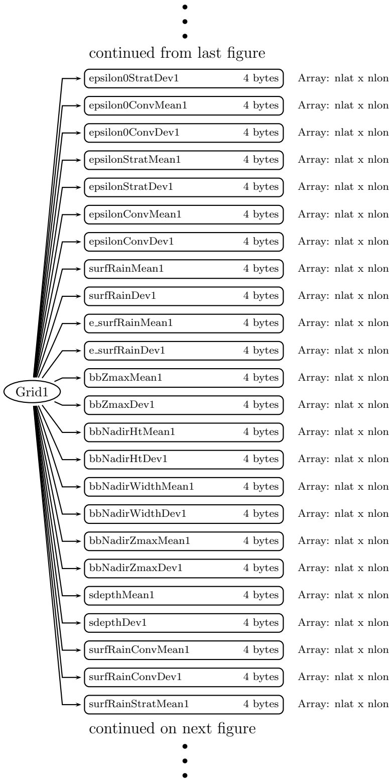
Figure 61: Data Format Structure for 3A25, Grid1, Grid1
