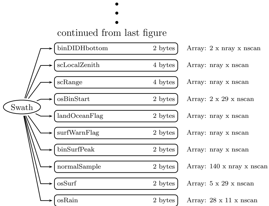
Figure 14: Data Format Structure for 1B21, PR Power
