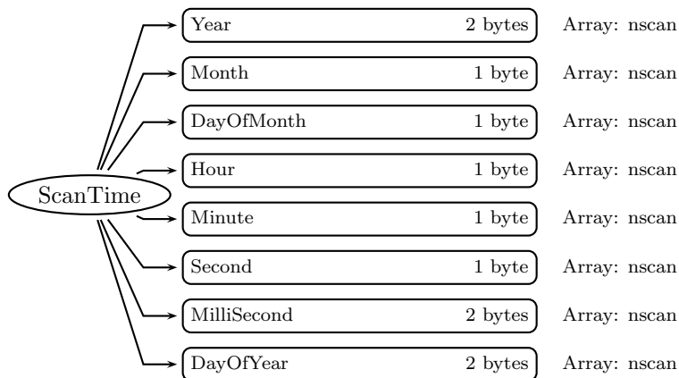
Figure 91: Data Format Structure for 2H31, ScanTime
