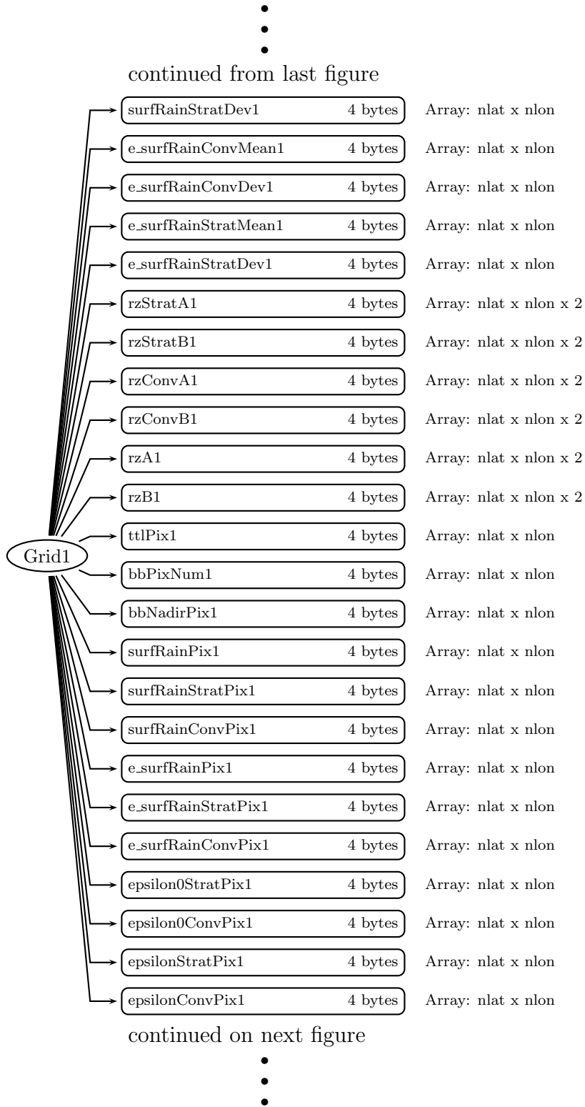
Figure 62: Data Format Structure for 3A25, Grid1, Grid1
