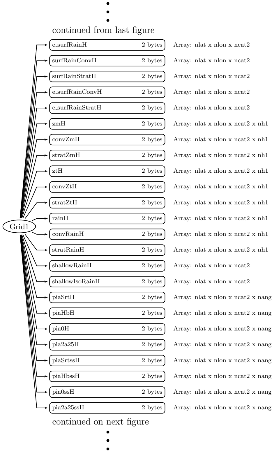
Figure 64: Data Format Structure for 3A25, Grid1, Grid1
