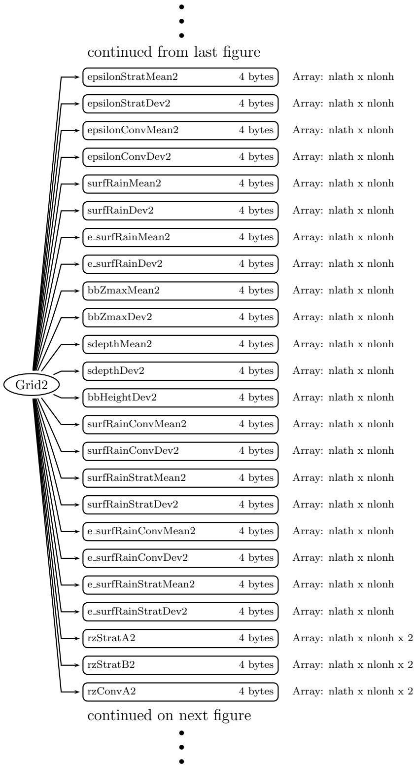
Figure 67: Data Format Structure for 3A25, Grid2, Grid2
