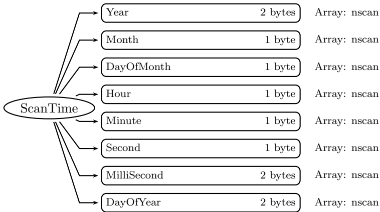
Figure 77: Data Format Structure for 2N25, ScanTime
