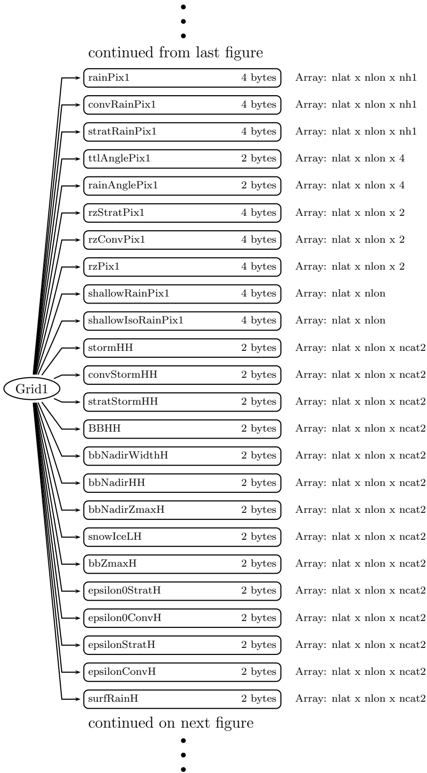
Figure 63: Data Format Structure for 3A25, Grid1, Grid1
