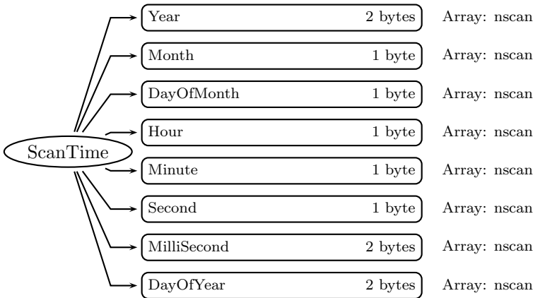
Figure 85: Data Format Structure for 2H25, ScanTime
