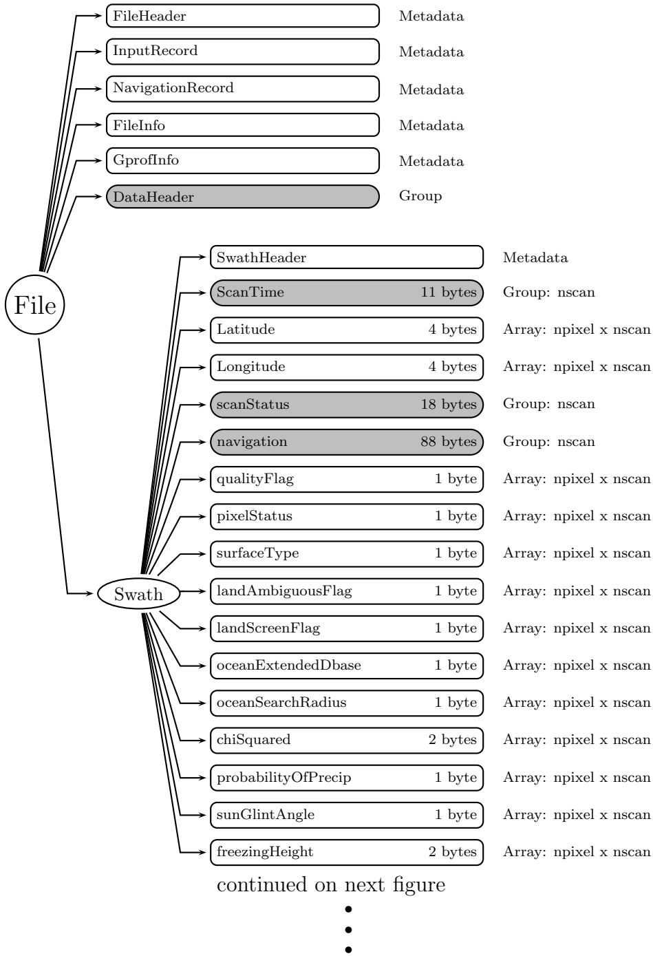
Figure 29: Data Format Structure for 2A12, TMI Profiling
