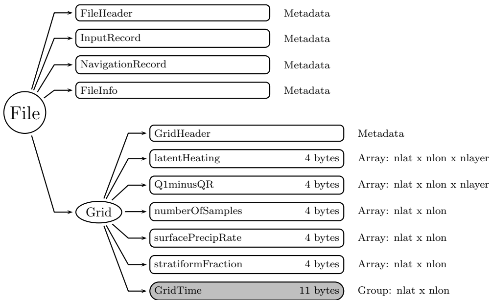
Figure 80: Data Format Structure for 3G12, TRAIN Gridded Orbital Heating
