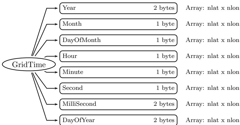
Figure 93: Data Format Structure for 3G31, GridTime
