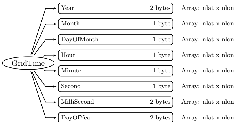
Figure 87: Data Format Structure for 3G25, GridTime
