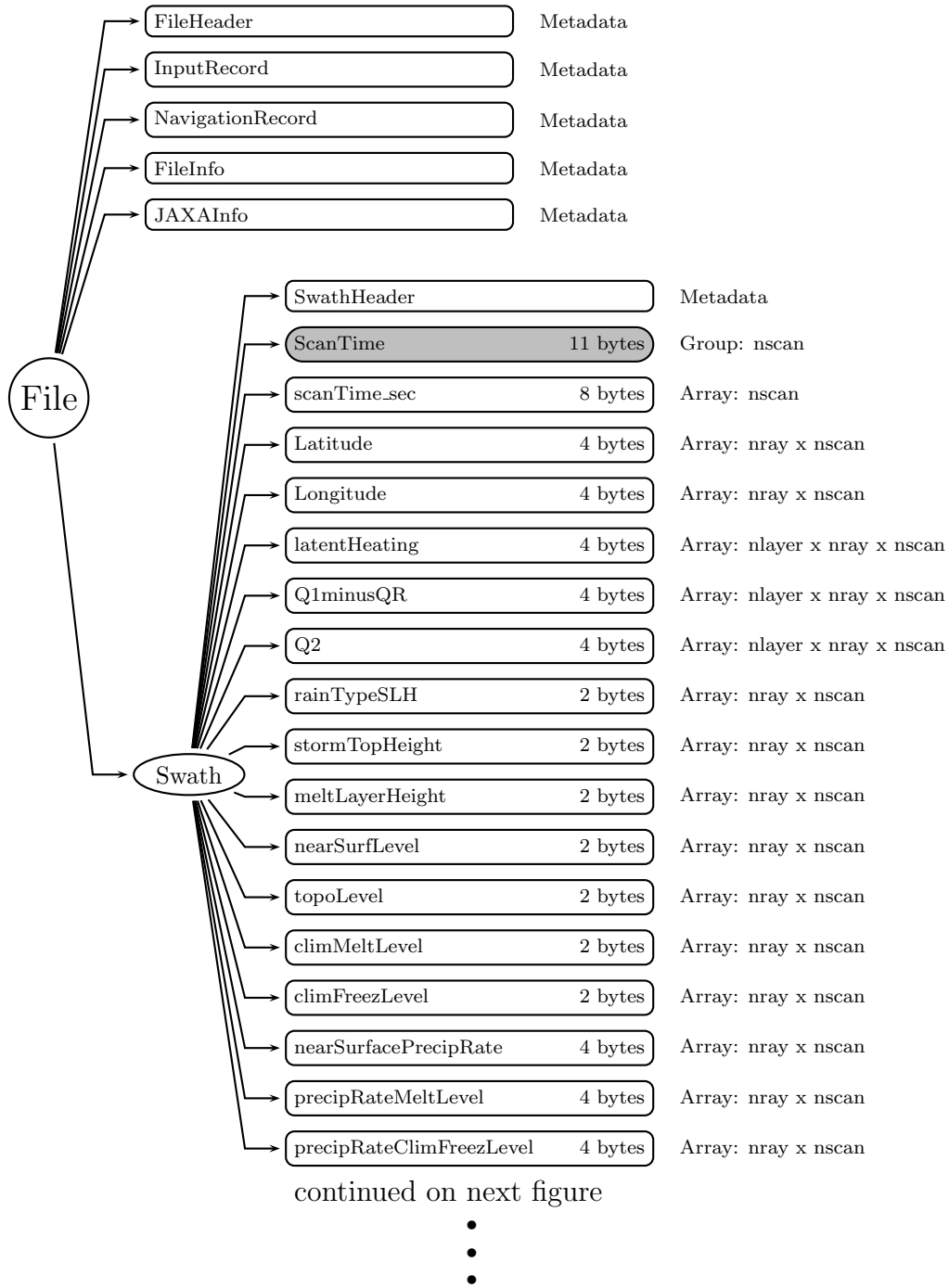
Figure 83: Data Format Structure for 2H25, Spectral Latent Heating
