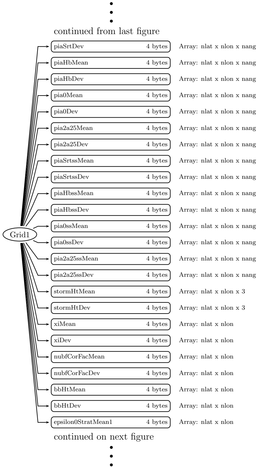
Figure 60: Data Format Structure for 3A25, Grid1, Grid1
