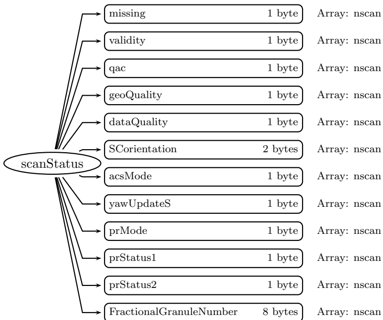
Figure 54: Data Format Structure for 2B31, scanStatus
