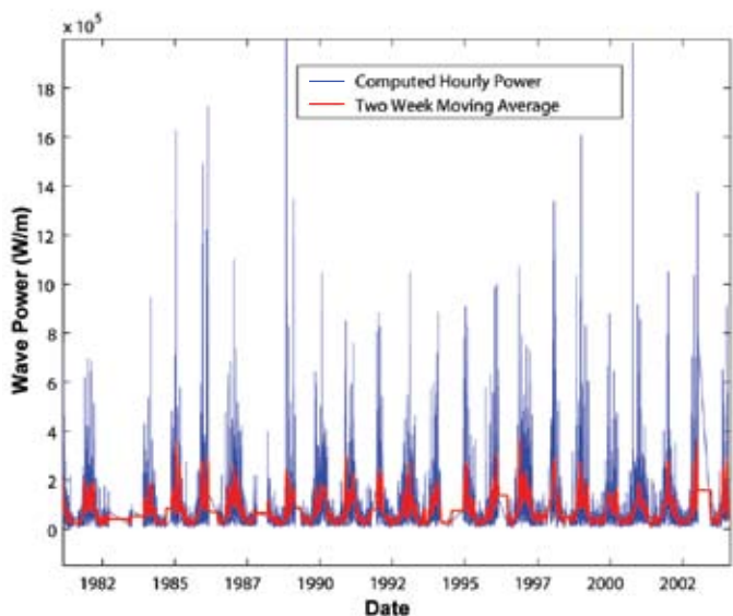
Figure 5. Time series of wave power computed from wave data from NOAA Buoy #51001 located near Nihoa Island in the Northwestern Hawaiian Islands. Data courtesy of NOAA Data Buoy Center.
