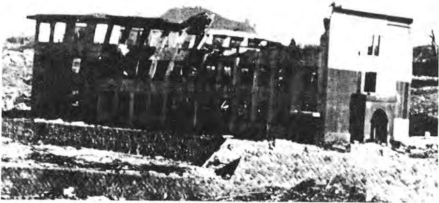
Figure 5.22b. Effects of horizontal loading on wall facing explosion (0.4 mile from ground zero at Nagasaki).
