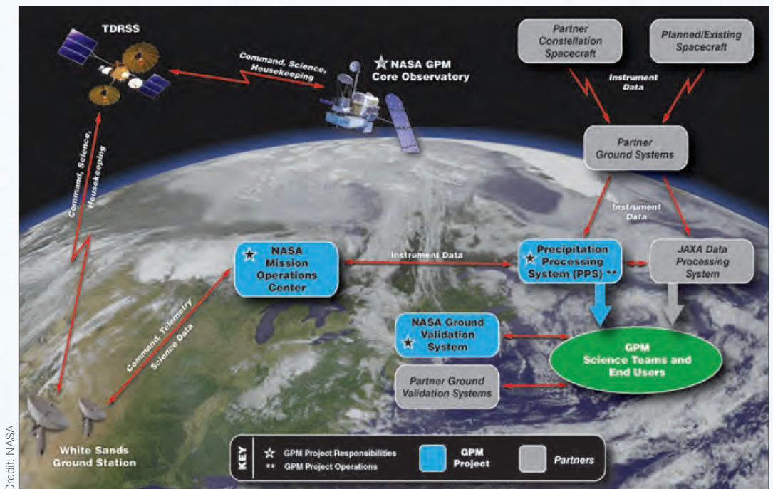
This graphic shows how data travel from the GPM Core Observatory and the constellation satellites to the NASA Precipitation Processing System at NASA's Goddard Space Flight Center.
