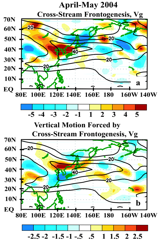
Fig. 18. April-May 2004: Anomalous (a) 200-hPa geostrophic frontogenesis in the cross-stream direction (shading, \times 10^{-11} \text{ K (ms}^{-1}\text{)} ), and (b) the associated anomalous quasi-geostrophic vertical motion at 300-hPa (shading, \times 10^{-4} \text{ hPa s}^{-1} ). The mean 200-hPa geostrophic wind speeds (contours, interval is 10 \text{ m s}^{-1} ) are overlaid in both panels. In (a) frontogenesis is shown red and frontolysis is blue. In (b) ascending motion is shown blue and descending motion is red.
