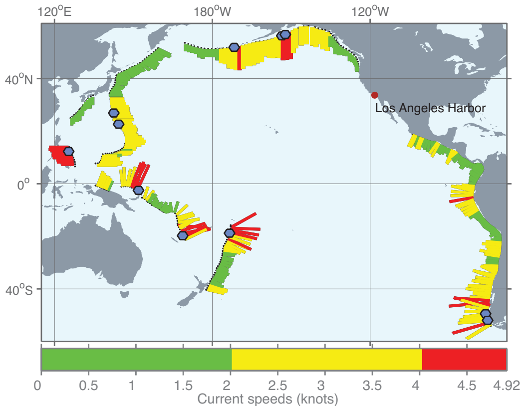
Figure 4.3: The maximum current velocities at the Los Angeles tide gauge, in knots, from tsunamis triggered by synthetic Mw 9.3 earthquakes along subduction zones around the Pacific Basin as modeled with the Los Angeles tsunami forecast model.
