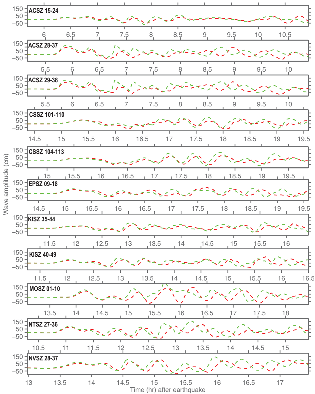
Figure 4.4: Comparison of the time series of the different synthetic tsunami events for the ports of Los Angeles and Long Beach, California, from high-resolution model (red) and forecast model (green). Sources are given in the left-hand side of each time series.
