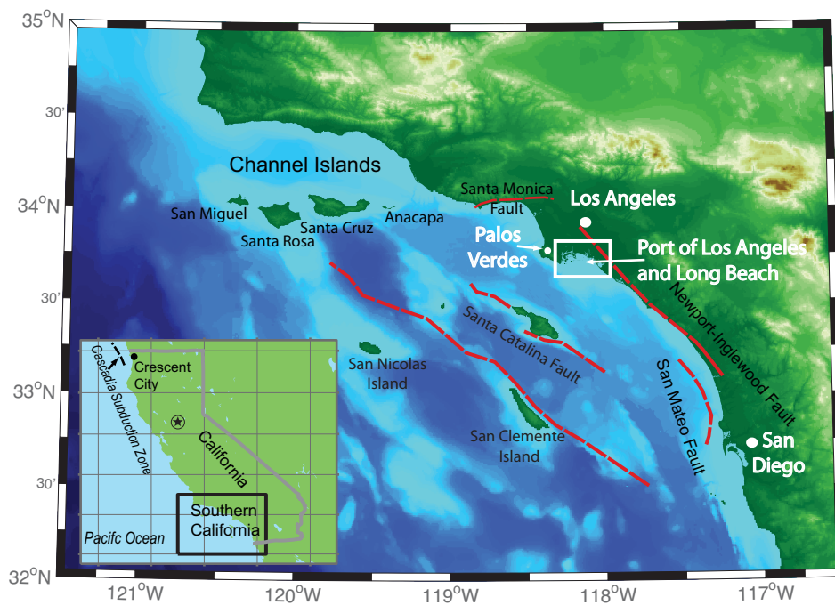
Figure 1.2: Regional setting showing geographic features of Southern California and surrounding major offshore fault lines with respect to the ports of Los Angeles and Long Beach.
