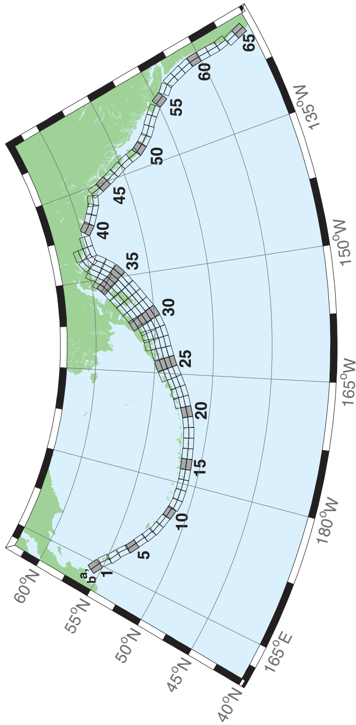
Figure C.1: Aleutian-Alaska-Cascadia Subduction Zone unit sources.
