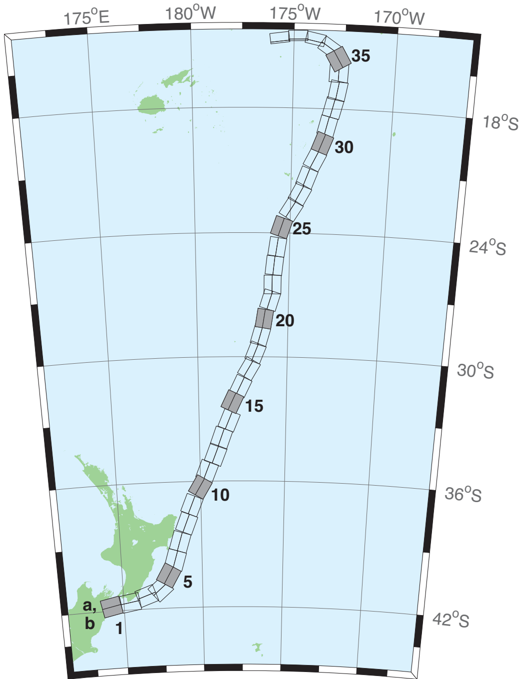
Figure C.7: New Zealand-Keradec-Tonga Subduction Zone unit sources.
