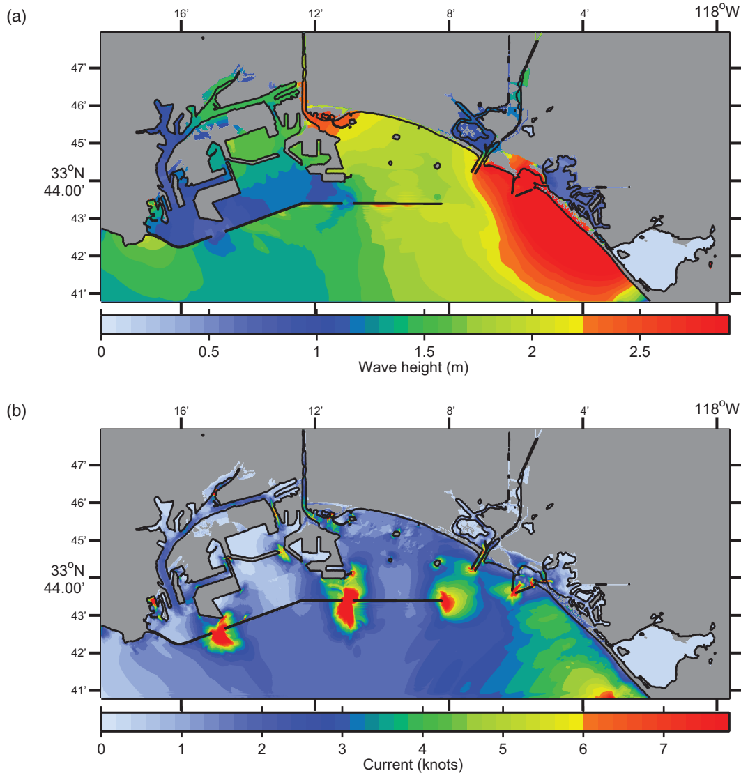
Figure 4.5: Maximum wave amplitudes (a) and currents (b) at the ports of Los Angeles and Long Beach from the synthetic tsunami ACSZ 29. The figure is represented in larger scale in Appendix B as Figures B.5 and B.6 , together with the results from the rest of the synthetic scenarios.
