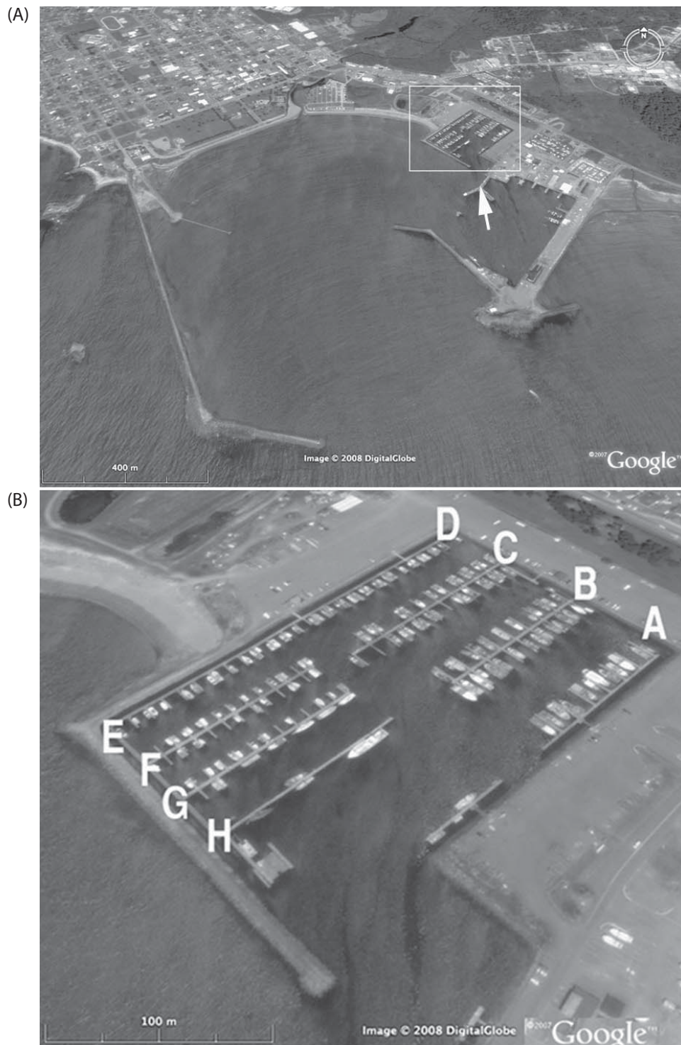
Figure 2.1: A Google Earth view of Crescent City and Crescent City Harbor. The upper figure shows Crescent City with the white box marking the small-boat basin, and the lower figure shows the small boat basin, where the Docks F, G, and H were damaged during the 2006 Kuril Islands Tsunami (Dengler et al. , 2009).
