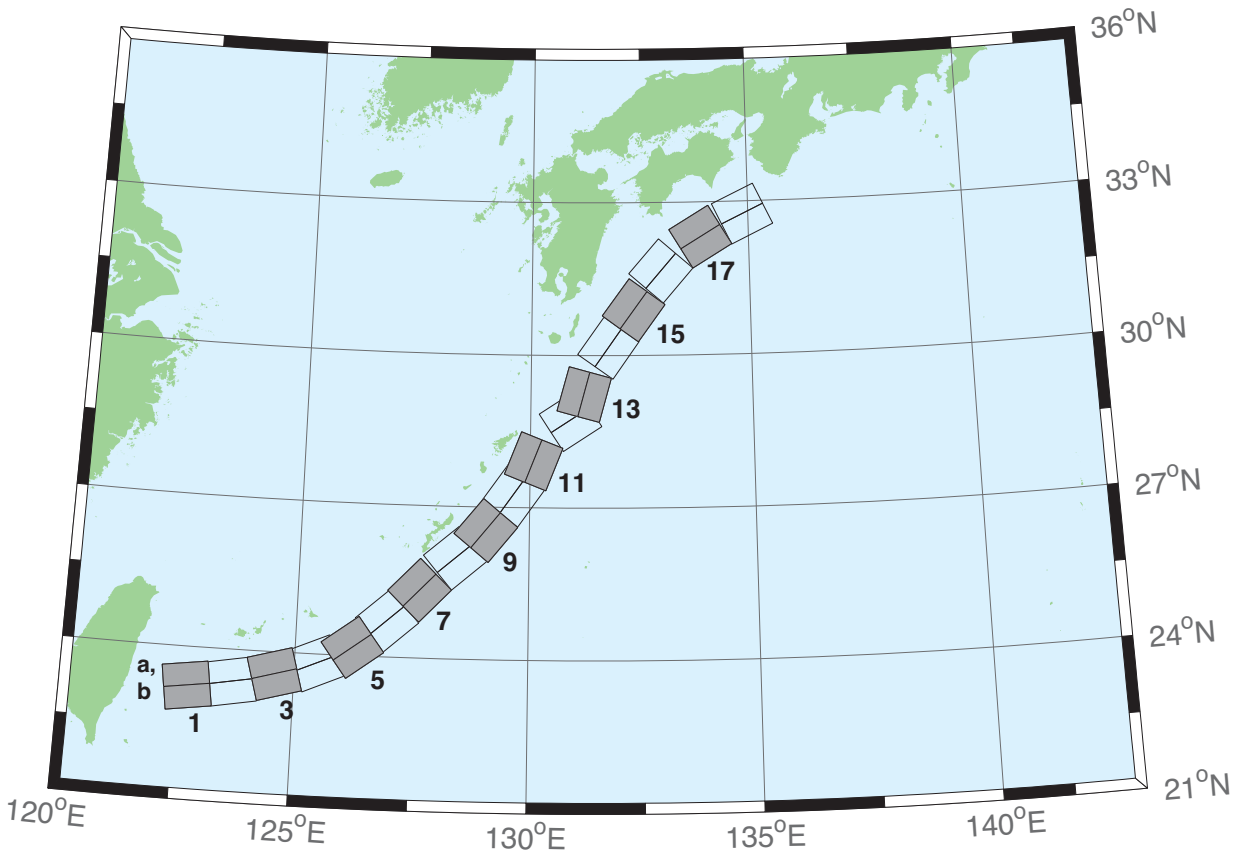
Figure C.9: Ryukyu-Kyushu-Nankai Zone unit sources.
