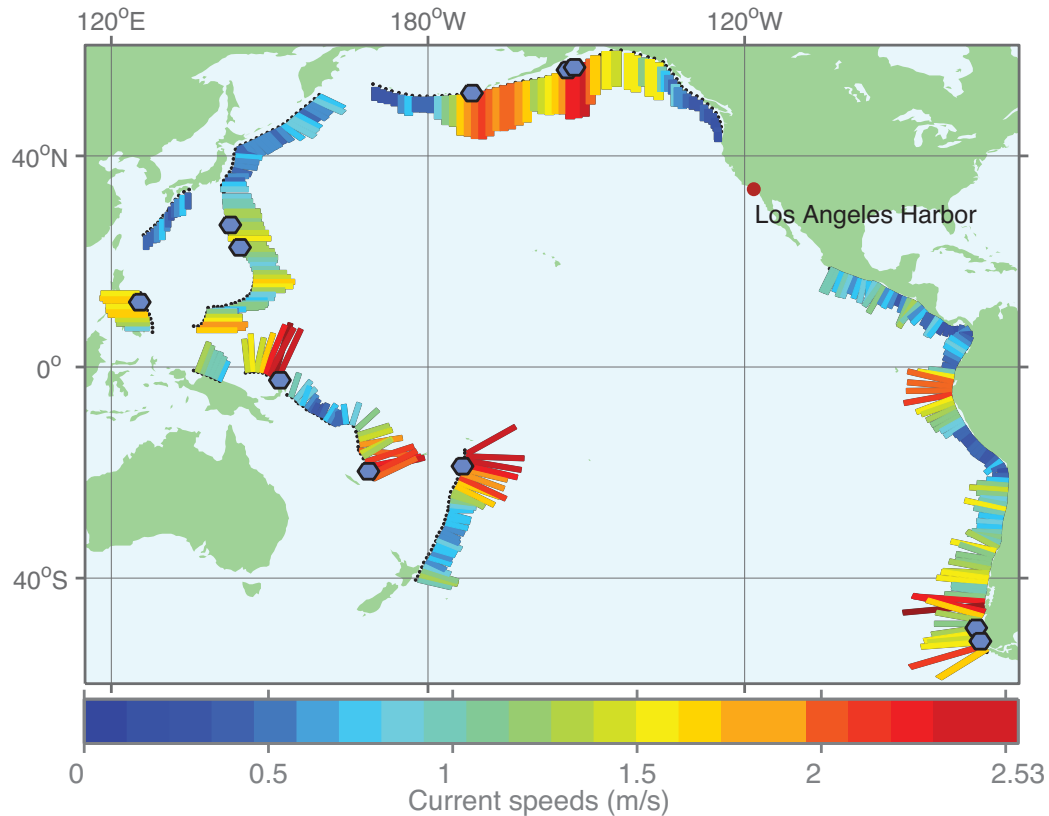
Figure 4.2: The maximum current velocities at the Los Angeles tide gauge, in meters/sec, from tsunamis triggered by synthetic Mw 9.3 earthquakes along subduction zones around the Pacific Basin as modeled with the Los Angeles tsunami forecast model.
