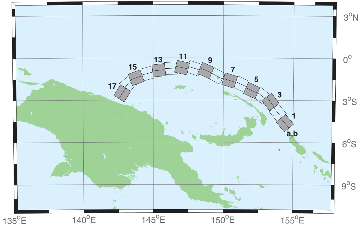
Figure C.5: Manus–Oceanic Convergent Boundary Subduction Zone unit sources.
