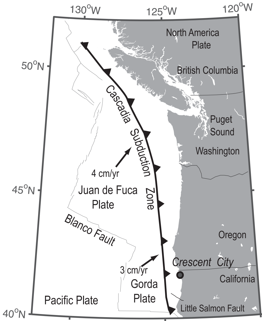
Figure 2.3: Map of the Cascadia Subduction Zone, the Juan de Fuca, Gorda, and Pacific Plates (modified from Satake et al. , 2003). Cascadia extends northward from Northern California to just north of Vancouver Island in British Columbia, Canada.
