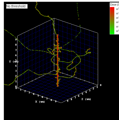
1 GeV/u ^{56}\text{Fe} nucleus LET \sim 150 keV/ \mu\text{m}
