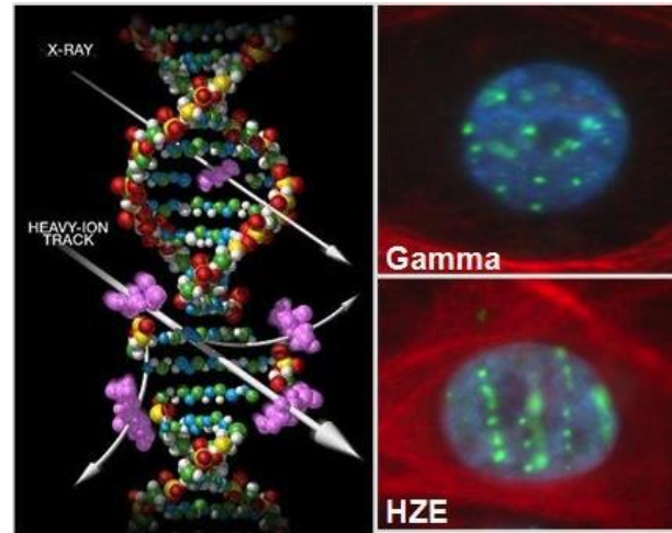
1 GeV/u ^{56}\text{Fe} nucleus LET \sim 150 keV/ \mu\text{m}
