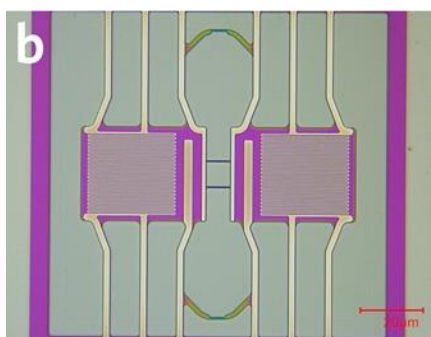
Figure 3.8 Prototype of Electro-Thermal Discovery Platform fabricated in the CINT Integration Laboratory.
