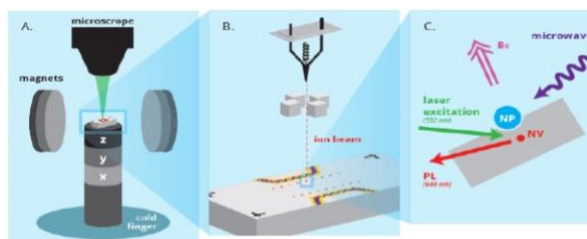
Figure 3.2 Schematic of the QSNMR Discovery Platform.
