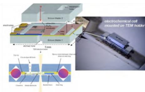
Figure 4.2 CINT's Electrochemical Discovery Platform.
