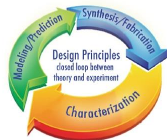
Figure 3.1 CINT leverages its diverse scientific community in an on-going cycle of scientific discovery.
