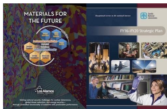
Figure 2.2 LANL (left) and SNL (right) strategic plans.
