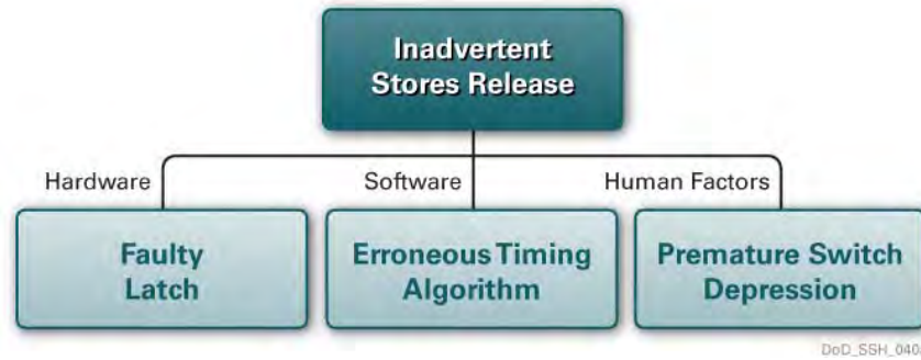
Figure 4-25: Hazard Analysis Segment
