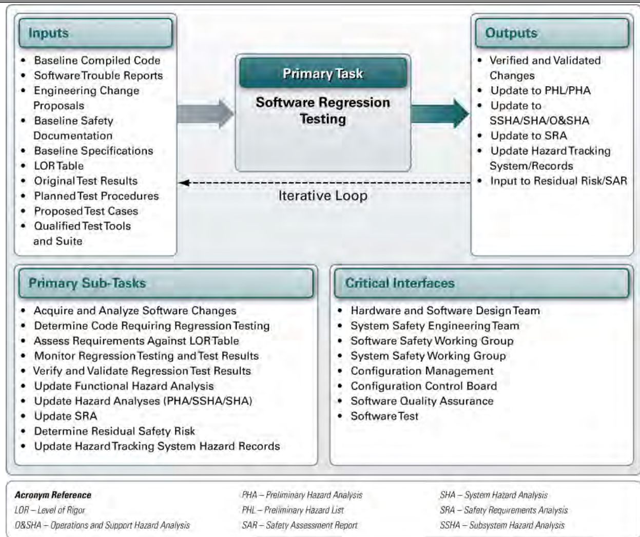
Figure 4-45: Software Regression Testing
