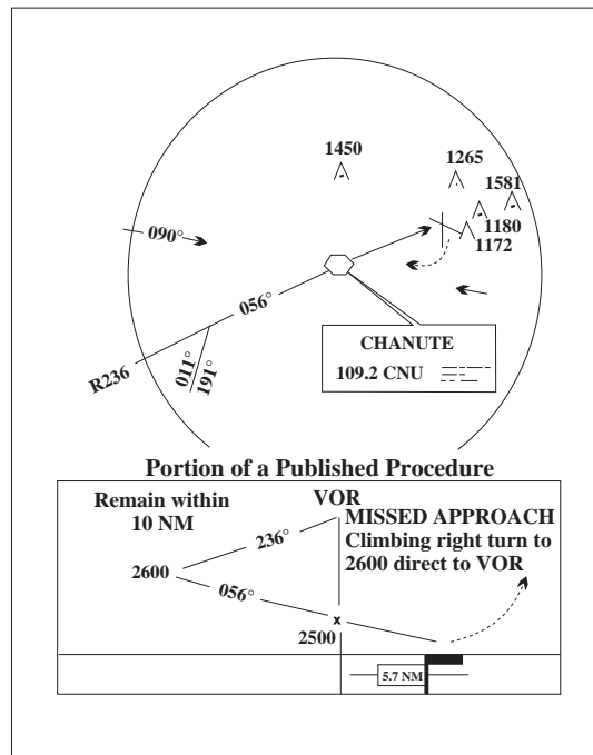
FIG ENR 1.5-37 Missed Approach
