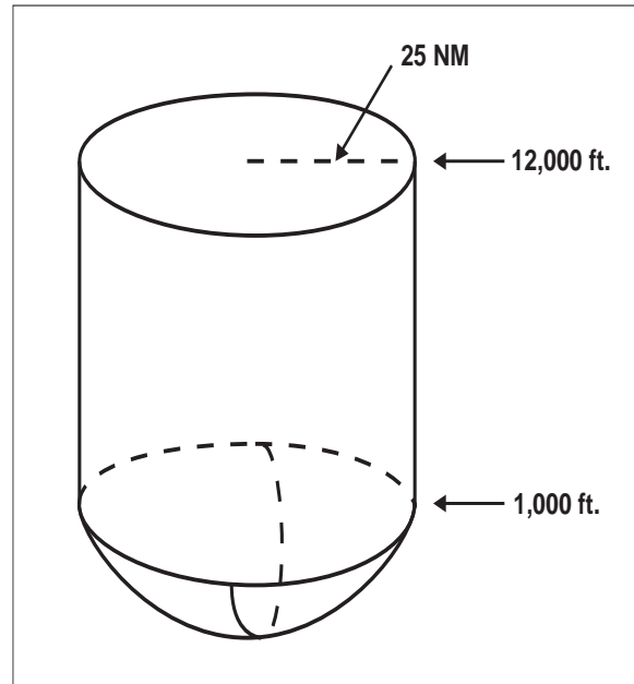
FIG GEN 3.4-3 Standard Terminal Service Volume (See FIG GEN 3.4-4 for altitudes below 1,000 feet.)
