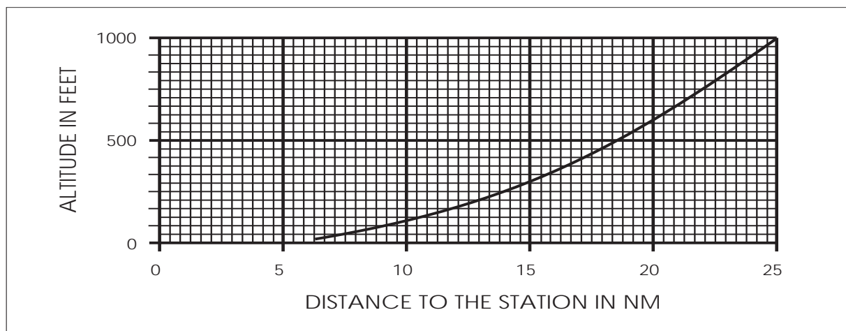
FIG GEN 3.4-4 Service Volume Lower Edge Terminal
