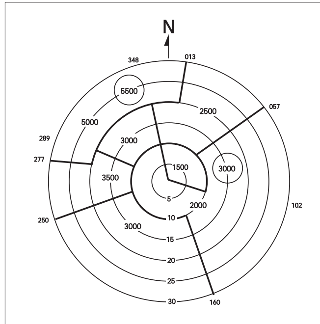
FIG ENR 1.5-26 Minimum Vectoring Altitude Charts
