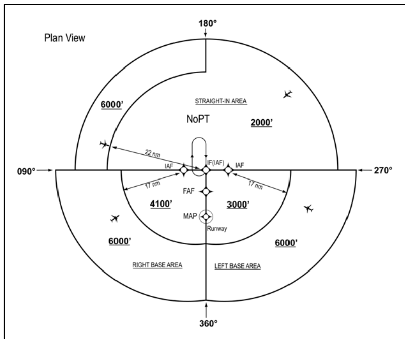
FIG ENR 1.5-20 Sectored TAA Areas
