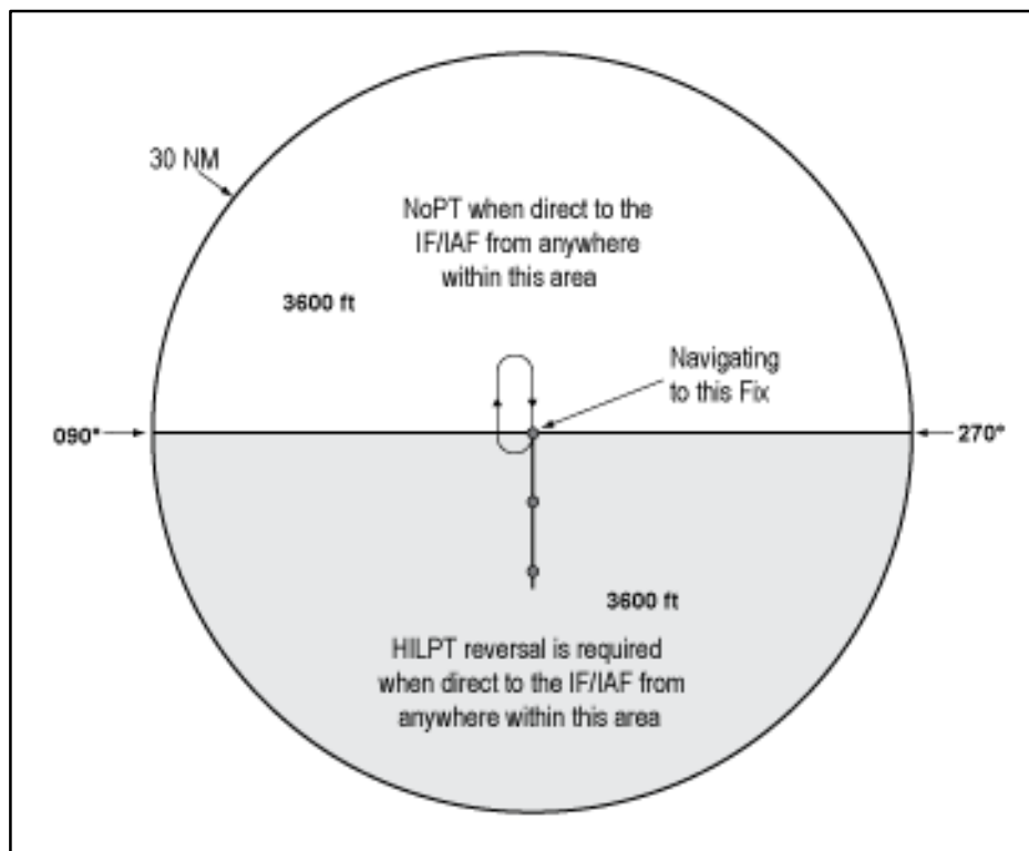
FIG ENR 1.5-22 TAA with Left and Right Base Areas Eliminated
