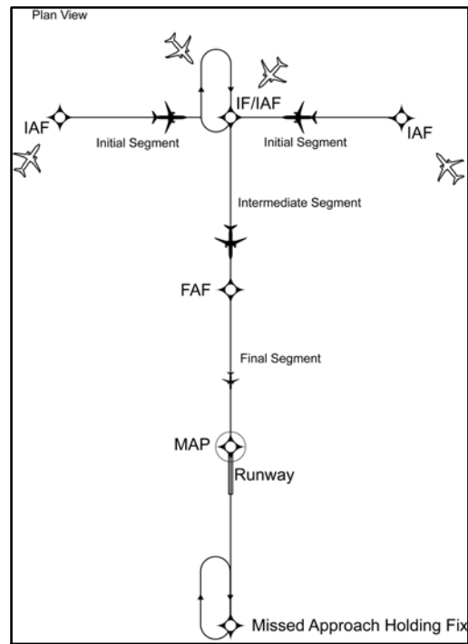
FIG ENR 1.5-17 Basic "T" Design
