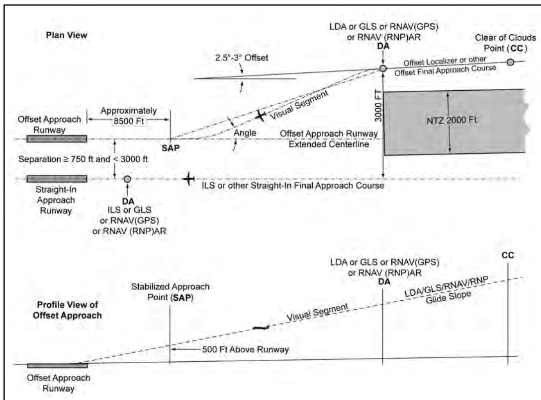
FIG ENR 1.5-34 SOIA Approach Geometry
