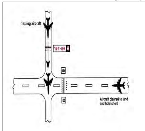
FIG ENR 1.1-8 Land and Hold Short of an Intersecting Taxiway
