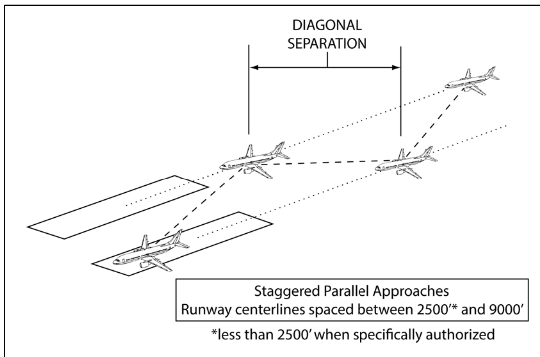
FIG ENR 1.5-31 Simultaneous (Parallel) Dependent Approaches
