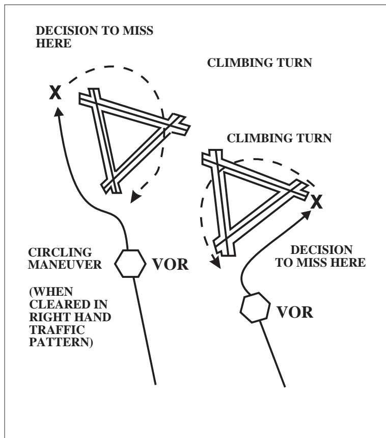
FIG ENR 1.5-36 Circling and Missed Approach Obstruction Clearance Areas
