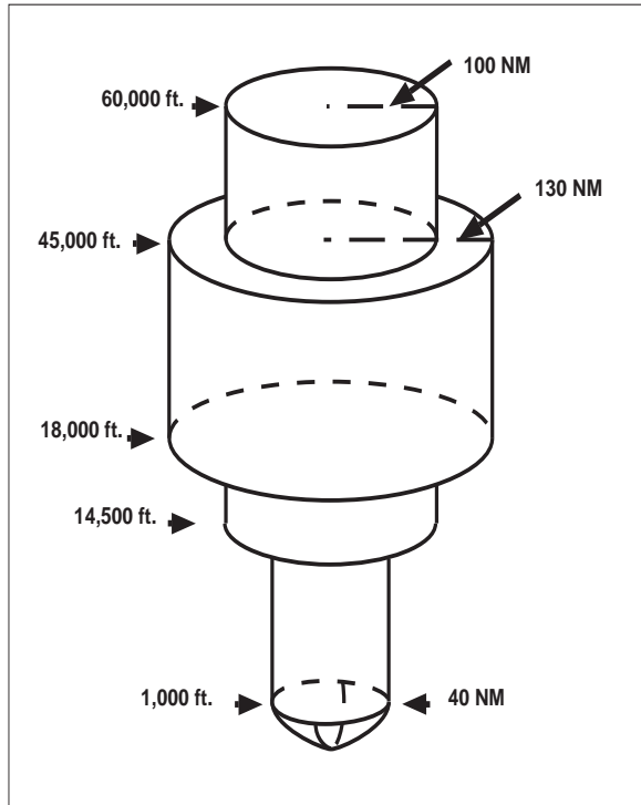
FIG GEN 3.4-1 Standard High Altitude Service Volume (See FIG GEN 3.4-5 for altitudes below 1,000 feet.)
