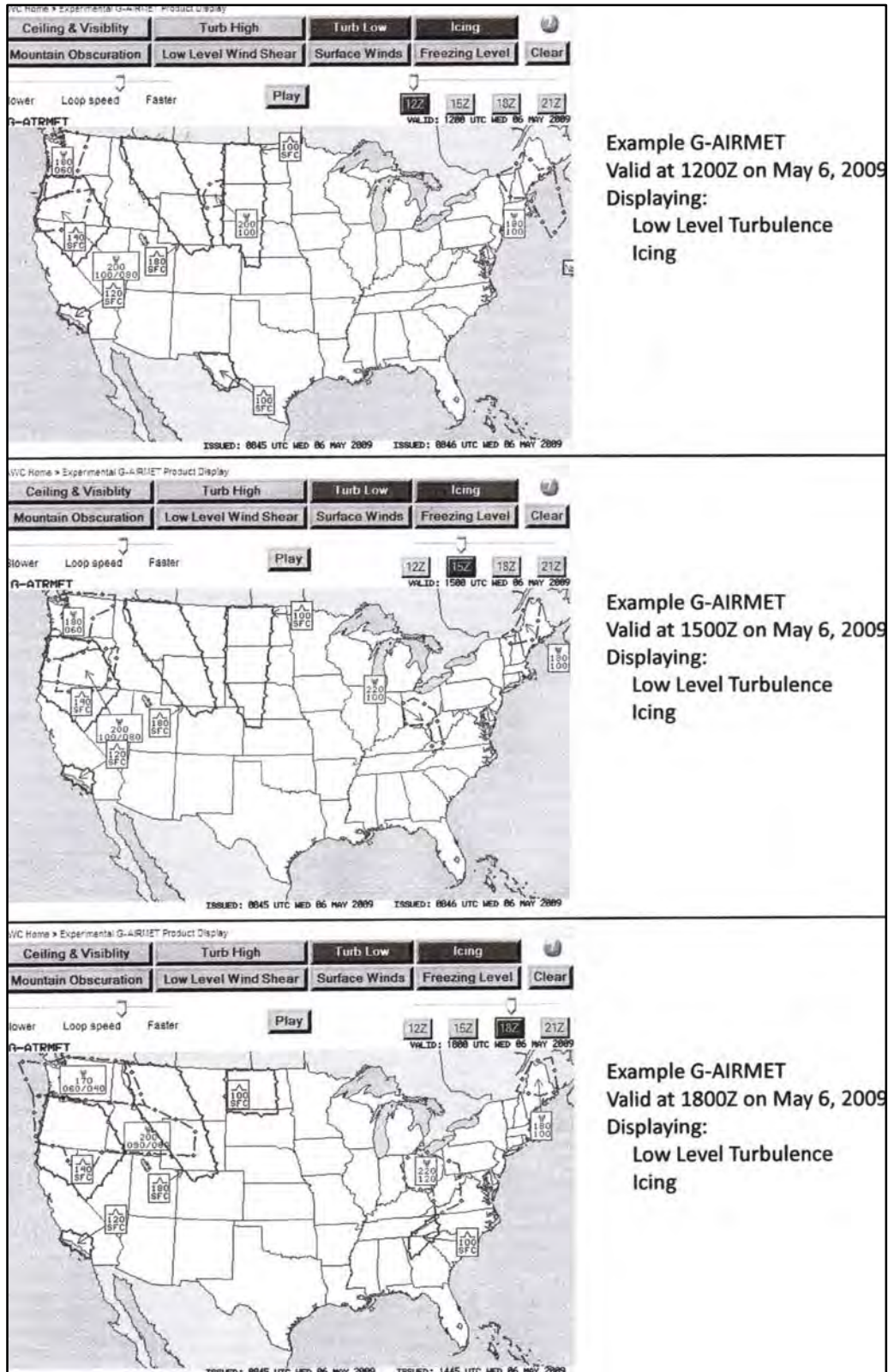
FIG GEN 3.5-4 G-AIRMET Graphical Product
