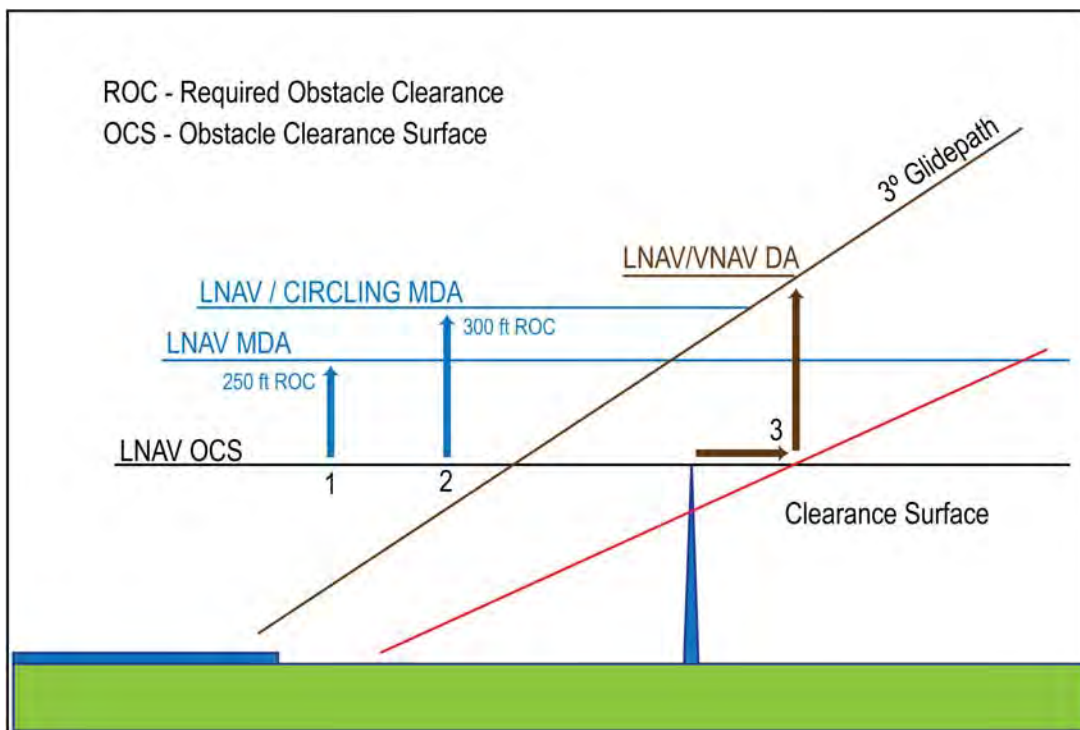
FIG ENR 1.5-28 Explanation of LNAV and/or Circling Minima Lower than LNAV/VNAV DA
