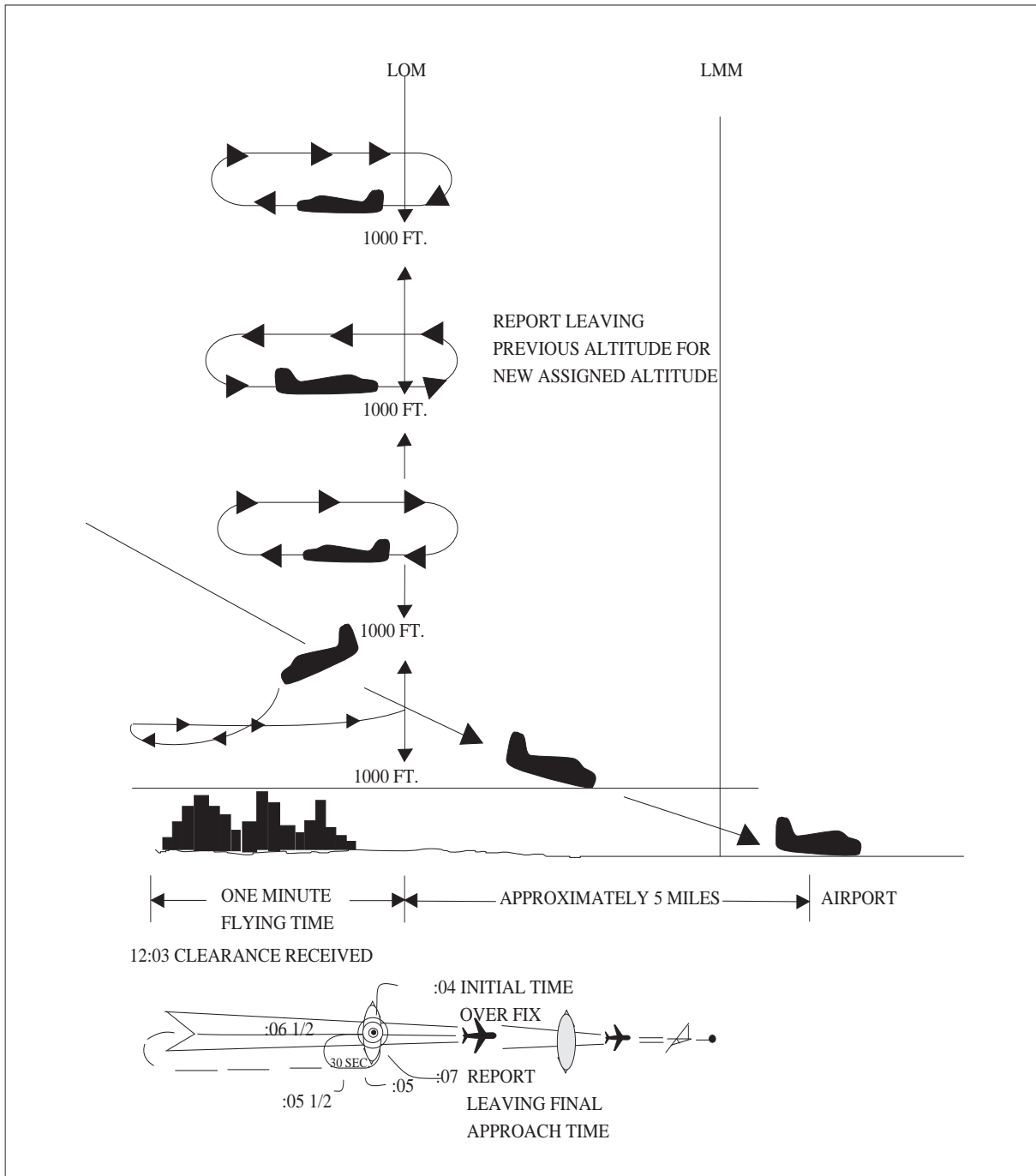
FIG ENR 1.5-35 Timed Approaches from a Holding Fix
