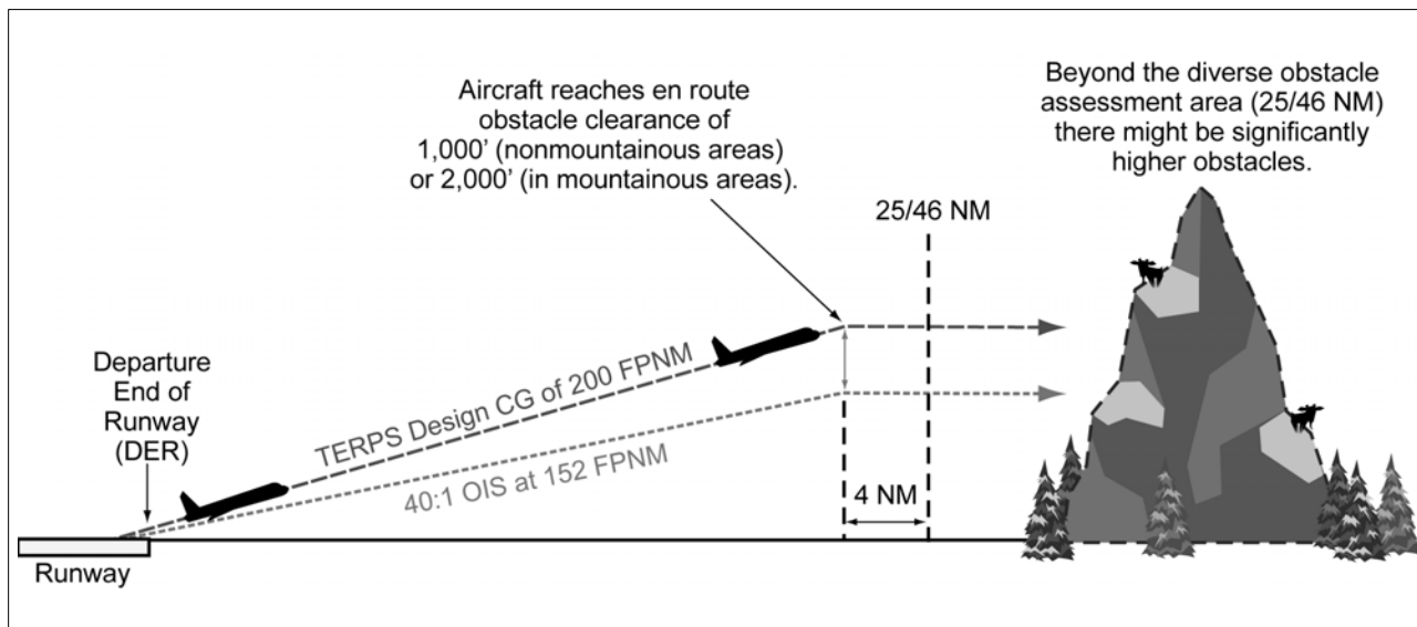
FIG ENR 1.5-39 Diverse Departure Obstacle Assessment to 25/46 NM
