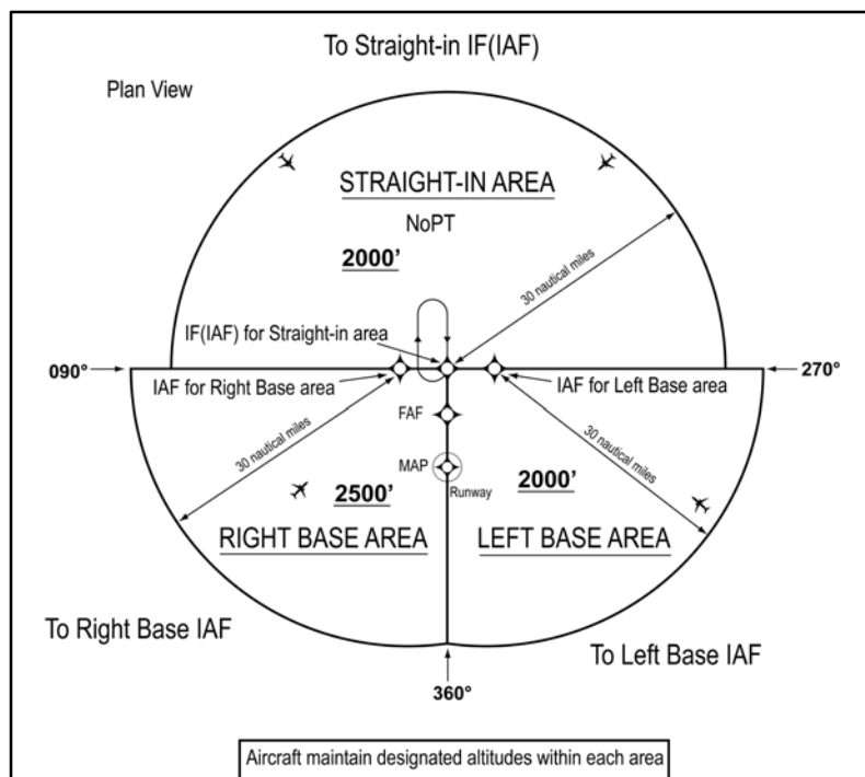
FIG ENR 1.5–19 TAA Area
