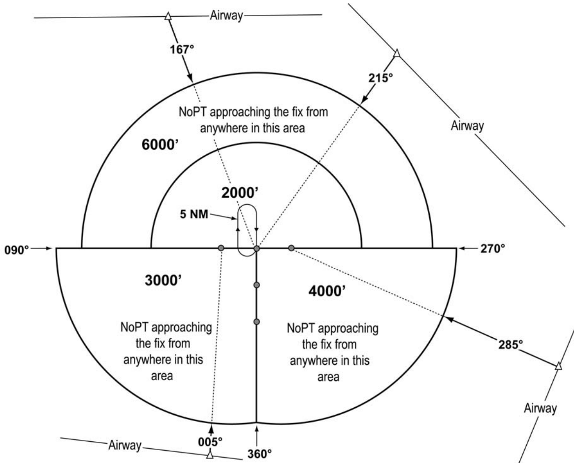
FIG ENR 1.5-25 Examples of a TAA with Feeders from an Airway
