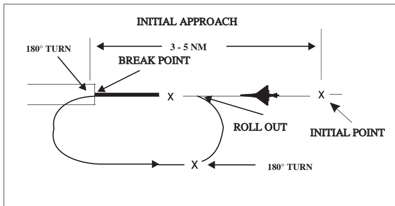
FIG ENR 1.5-38 Overhead Maneuver
