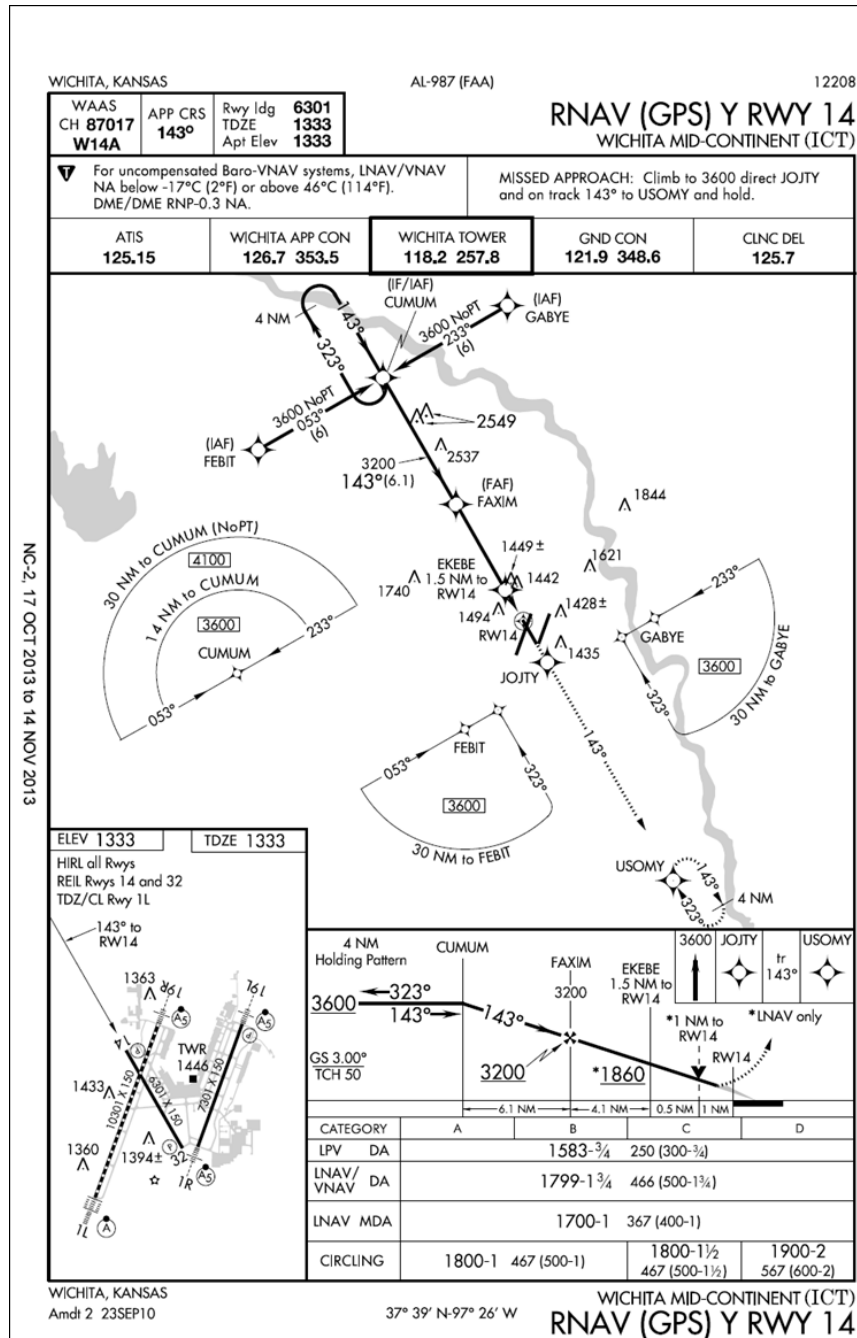
FIG ENR 1.5-21 RNAV (GPS) Approach Chart
