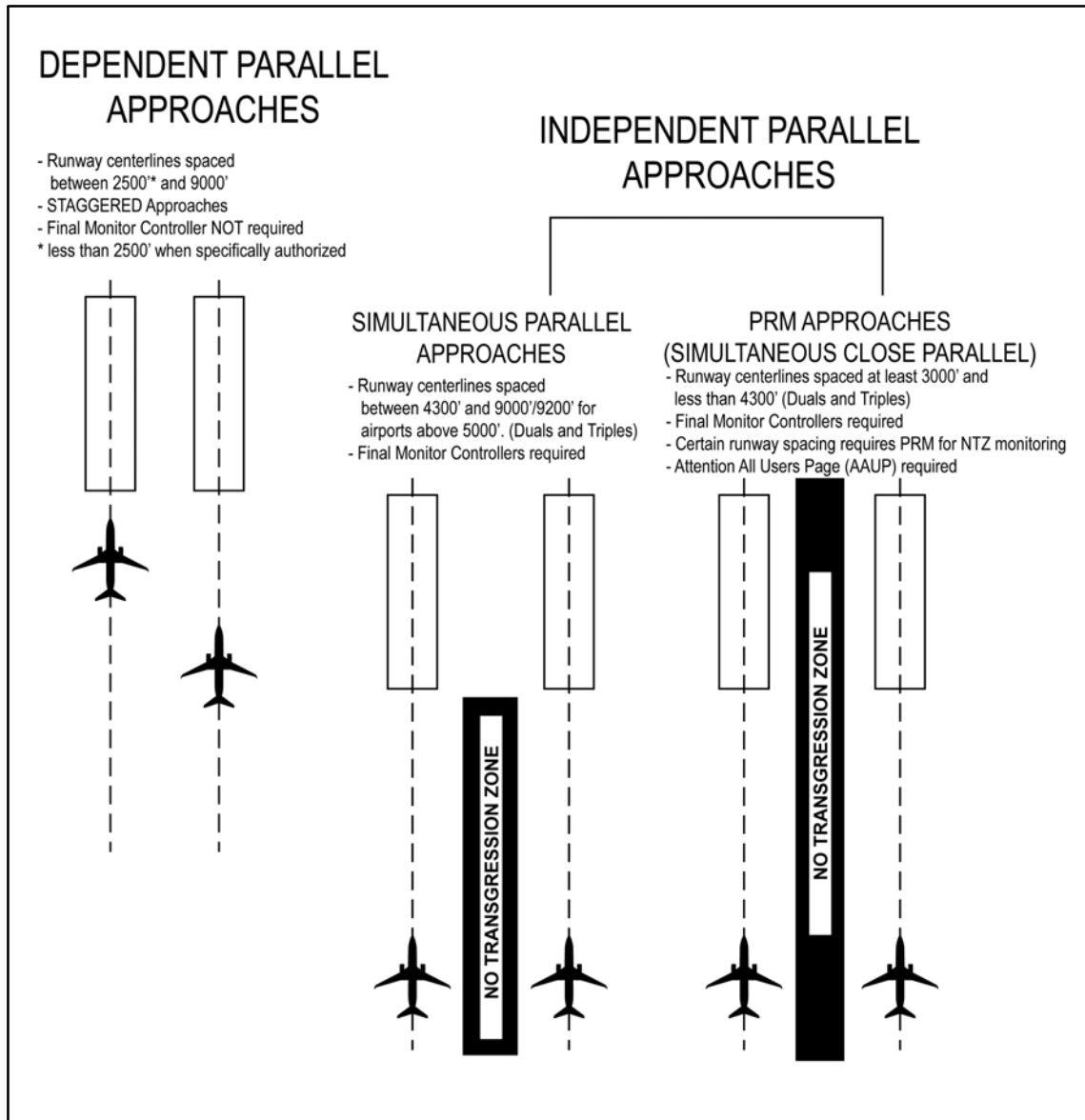
FIG ENR 1.5-30 Simultaneous Parallel Approaches (Parallel Runways and Approach Courses and Offset Approach Courses between 2.5 and 3.0 degrees)
