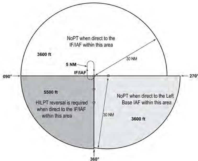
FIG ENR 1.5-24 TAA with Right Base Eliminated
