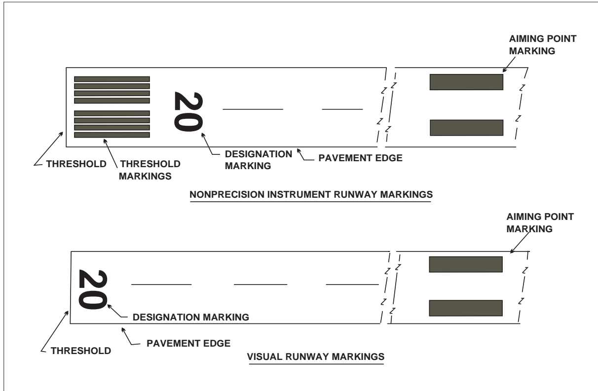
FIG AD 1.1-16 Nonprecision Instrument Runway and Visual Runway Markings
