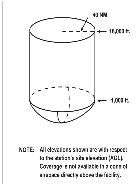
FIG GEN 3.4-2 Standard Low Altitude Service Volume (See FIG GEN 3.4-5 for altitudes below 1,000 feet.)
