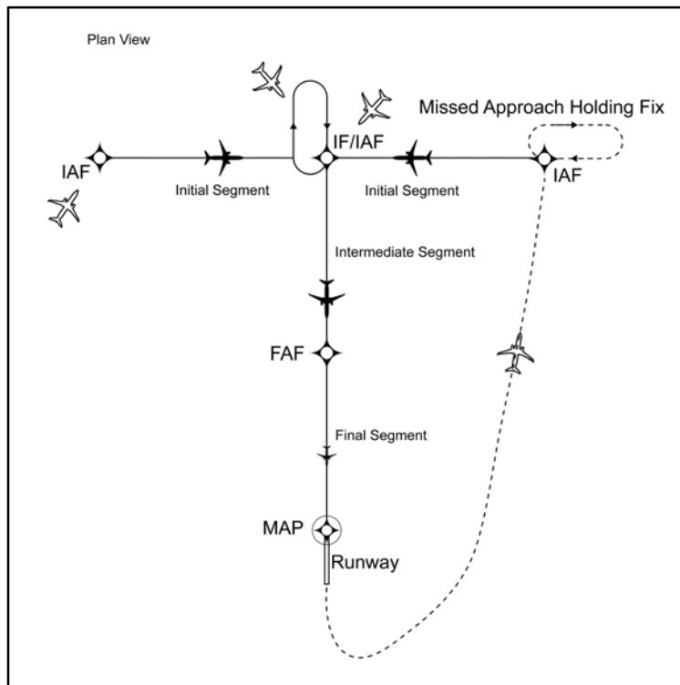
FIG ENR 1.5-18 Basic "T" Design
