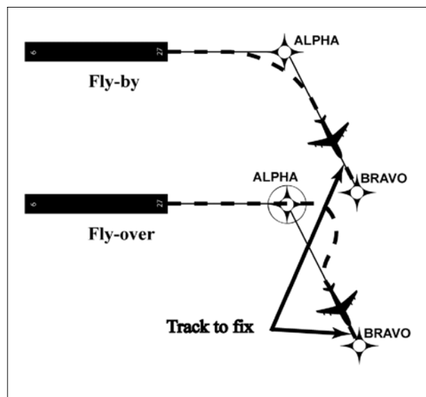
FIG ENR 1.17-3 Track to Fix Leg Type
