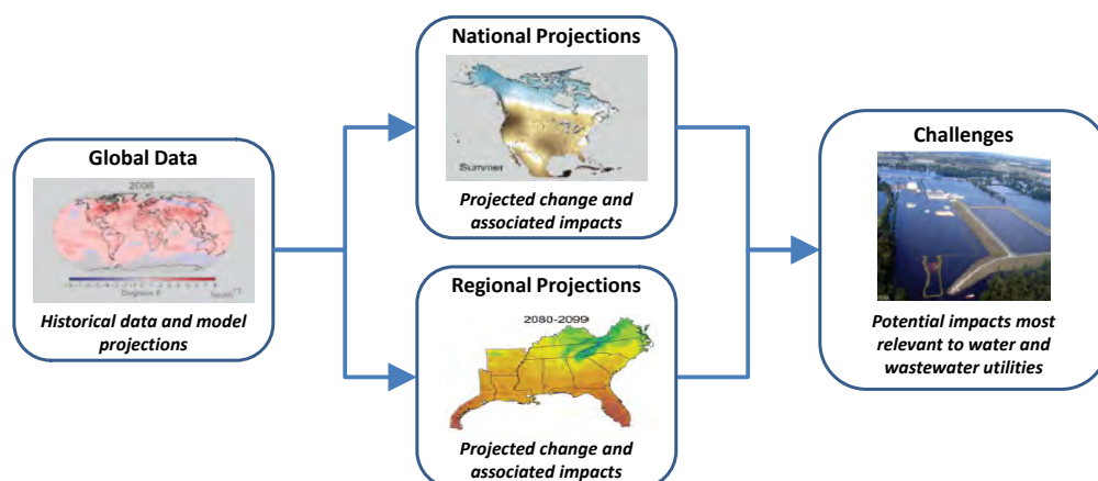
Figure 1.1. Scheme to translate climate data and model outputs into challenges for water utilities. Model run images from USGCRP (2009).
