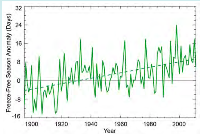
Difference in Mean Annual Freeze-Free Season Length for the U.S. Great Plains (Deviations from the 1901-1960 Average)
