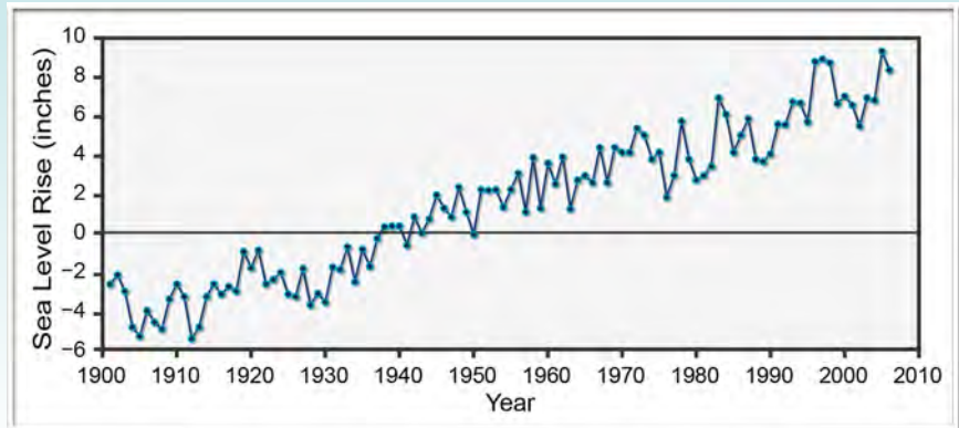
Observed Sea-Level Rise in New York City
