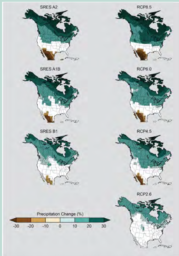
Figure 1.2. Comparison of projected wintertime precipitation changes between SRES and RCP scenarios (USGCRP 2014).
