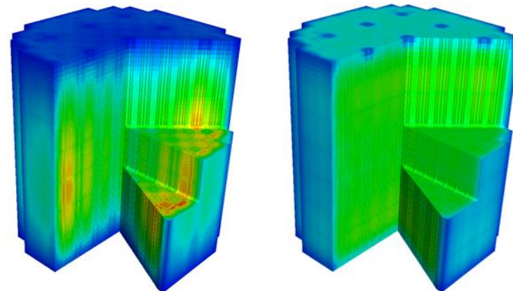
The beginning (left) and end (right) from a simulation of 3D pin power distribution at the Watts Bar nuclear power plant.
