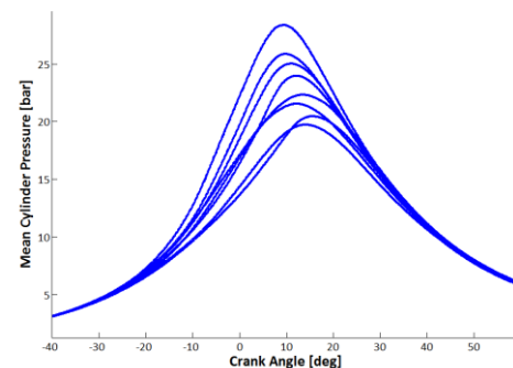
Cylinder pressure during the combustion phase for different engine cycles showing dispersion under parametric variation. Mapping the range and nature of cyclic dispersion of a wide parameter space helps understand the nature of factors contributing to cyclic variability.
