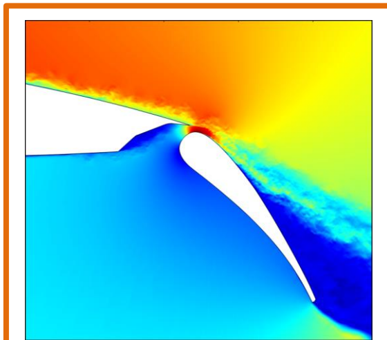
Streamwise velocity contours near multi-element airfoil flap.
