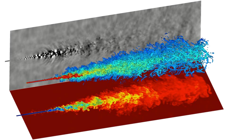
Three-dimensional rendering of supercritical fuel injection processes at Diesel engine conditions (n-dodecane – air, 60 bar). Axial velocity (center), pressure (back), temperature distribution (bottom).
