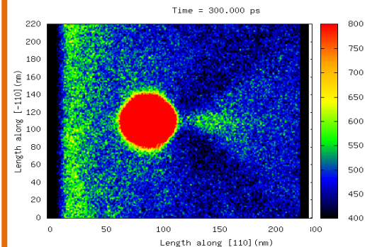
Caption: A triangular secondary hot zone forms beyond the circular-shaped primary hot spot
