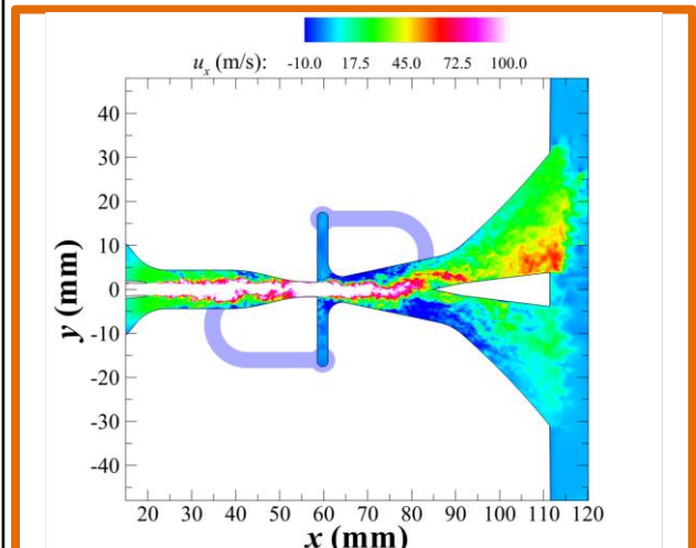
Streamwise velocity contours of Internal SaOB actuator flow (47M cvs)
