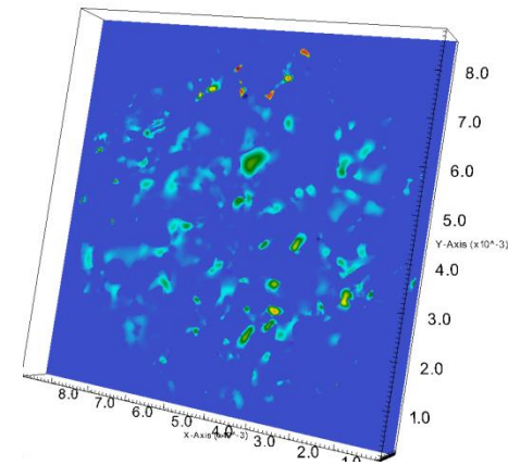
Computational domain from image and steady state flow in Bedford limestone (D. Trebotich)
