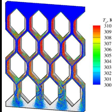
DEM simulations of 300 micron particles colored by temperature
