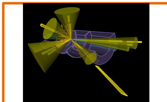
An example of an LHC proton-proton collision event simulated at NERSC. This event produced two electrons (yellow) accompanied by several jets of particles (green).
