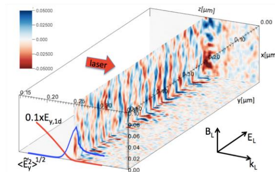
Field fluctuations [ E_y - E_y, 1d ] due to plasma waves in a highly resolved 3D PIC simulation, shown near the target surface at z = 0.25 \mu\text{m} . Laser is incident from z = 0 .
