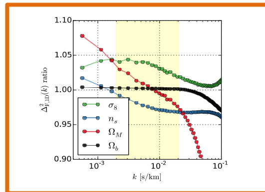
Figure: 1-d flux power spectra for different cosmologies from the Nyx simulation set.
