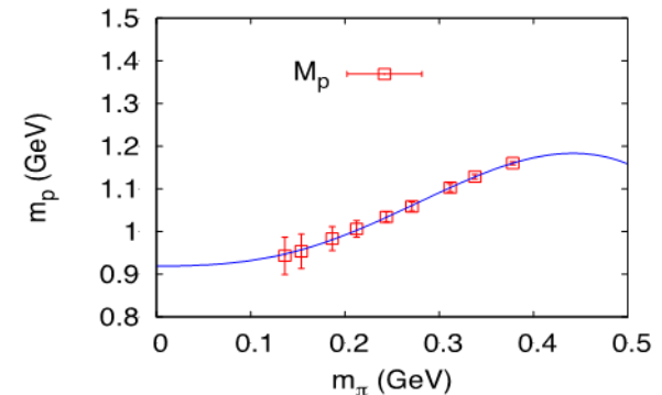
Nucleon mass as a function of the pion mass calculated with the sea quark mass at the physical point – chi QCD Collaboration
