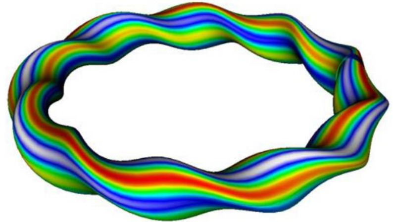
GTC simulation of Alfvén eigenmode structures in LHD. [Spong, 14 th IAEA Technical Meeting on Energetic Particles in Magnetic Confinement Systems, 2014, Vienna]
