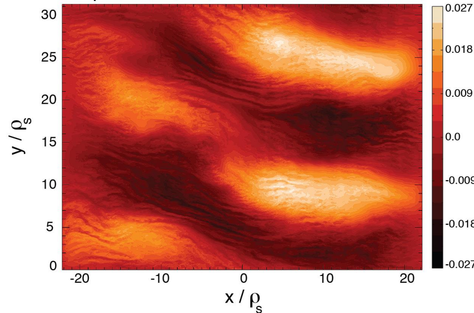
Snapshot of predicted midplane fluctuations in the Alcator C-Mod tokamak
