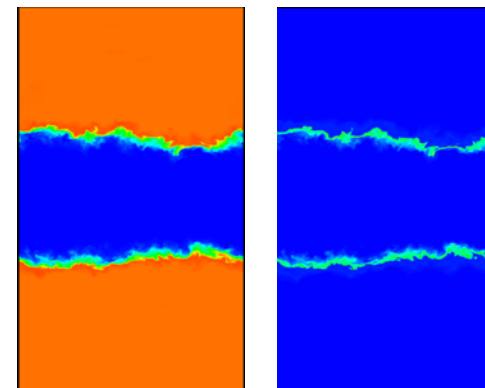
Snapshot images from simulation of periodic turbulent reacting jet (flow left to right). Transport part of the Navier-Stokes equations solved with CPUs and chemistry parts solved with GPUs.
