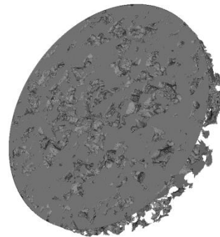
Computational domain from image and steady state flow in Bedford limestone (D. Trebotich)
