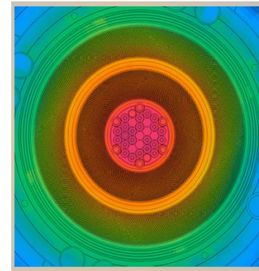
Neutron flux in a detailed simulation of the HFIR core
