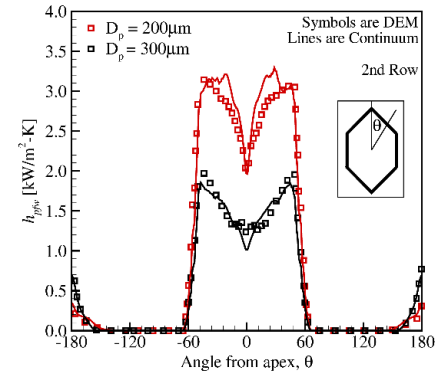
DEM and continuum (new model) comparisons of local heat transfer coefficient
