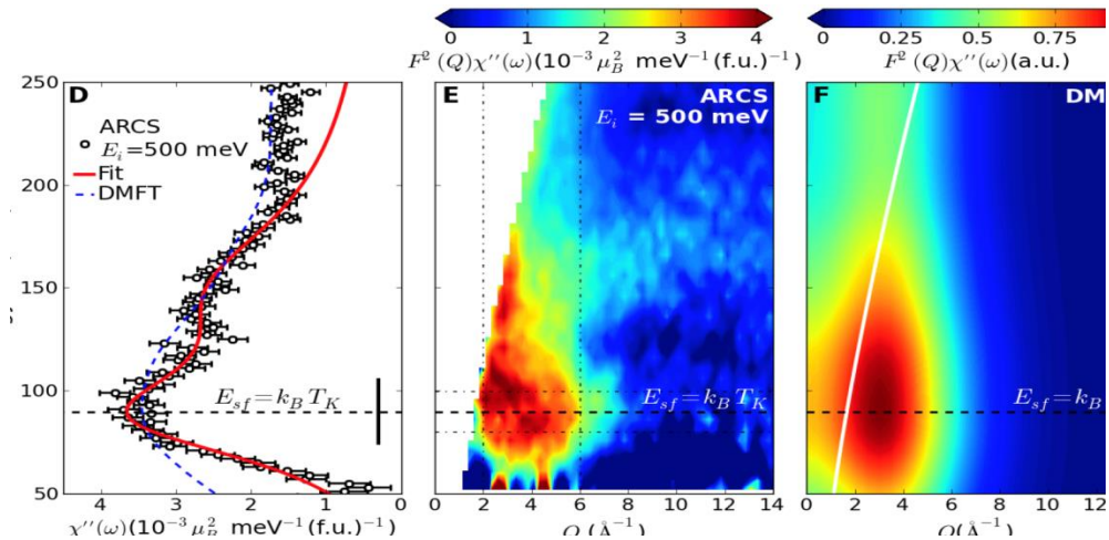
Comparison of the predicted S(q,\omega) for \delta -Pu (right) with the experimental observations (middle). Left panel shows the q integrated intensity in absolute units with statistical errors shown. Larger systematic error bars in the experimental data at low and high energy are not shown.
