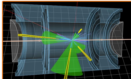
One of the two billion simulated events produced by Mira for ATLAS
