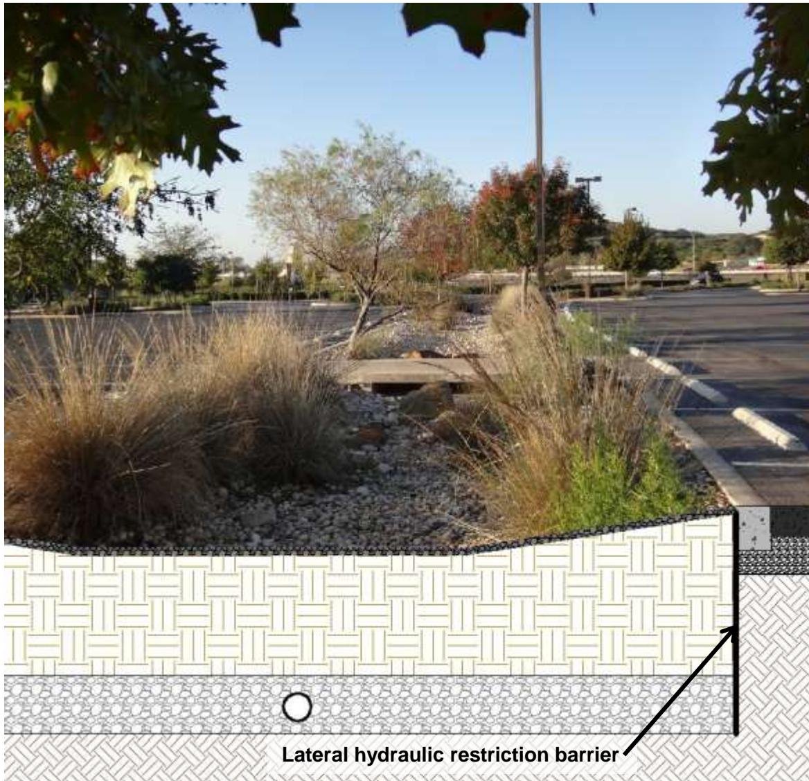
Bioswale at Rim Retail Center, San Antonio, Texas
