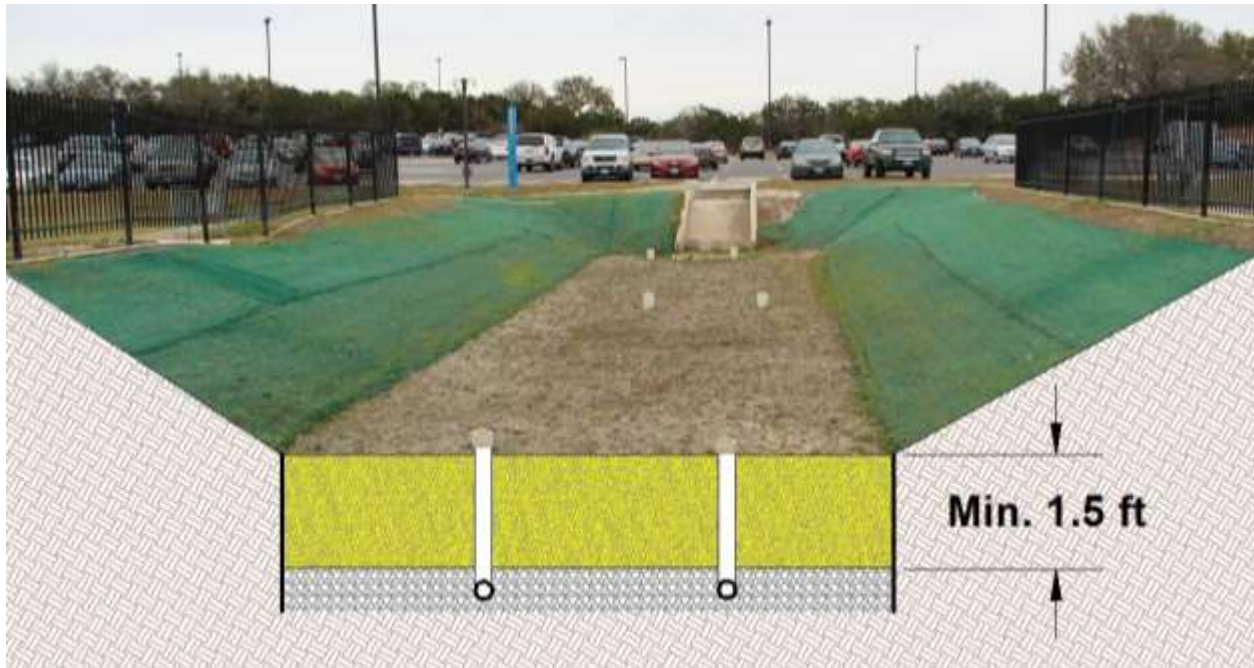
Figure B-6-4. Sand filter geometry and profile.
