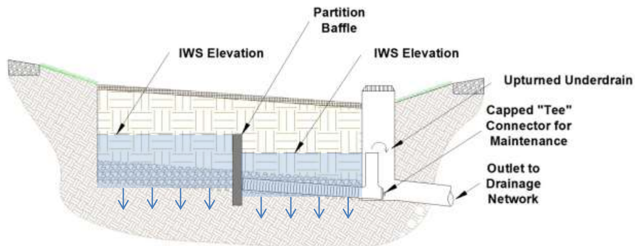
Figure B-2-3. Bioswale incorporating IWS and a partition baffle to enhance exfiltration.
