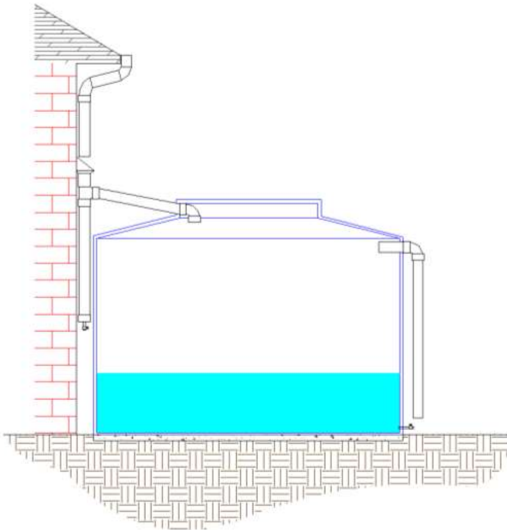
Figure B-8-5. Dry conveyance inlet configuration.
