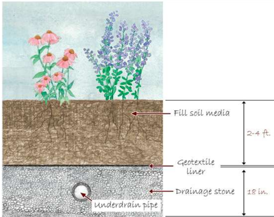
Figure B-11-14. Underdrain barrier option 2: geotextile liner.
