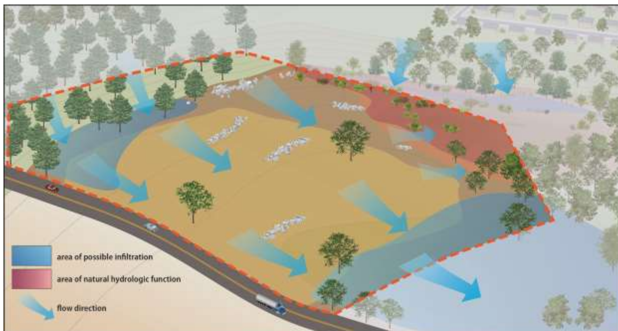
Figure 1-11. Identify and protect key hydrologic areas, such as infiltrating soils (blue area) and wetlands (orange areas).
