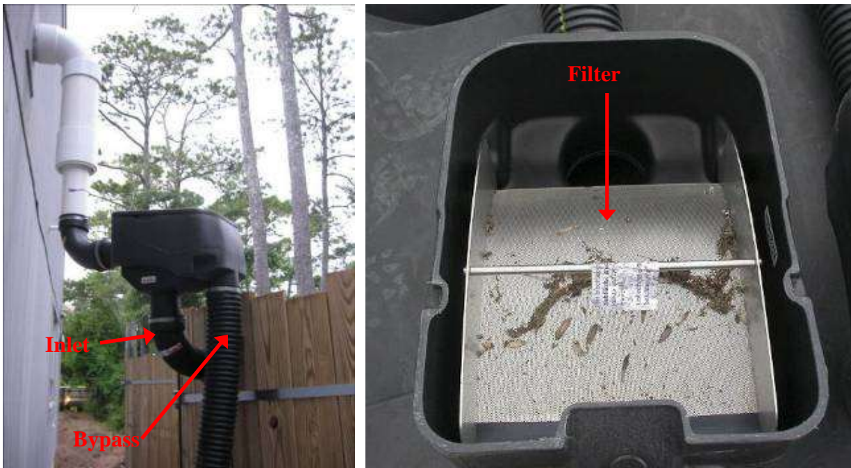
Figure B-8-13. Self-flushing filter with a bypass.
