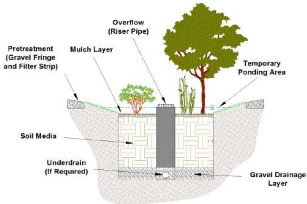
Figure B-1-10. Online bioretention area with a vertical riser overflow with a variable flow outlet structure.
