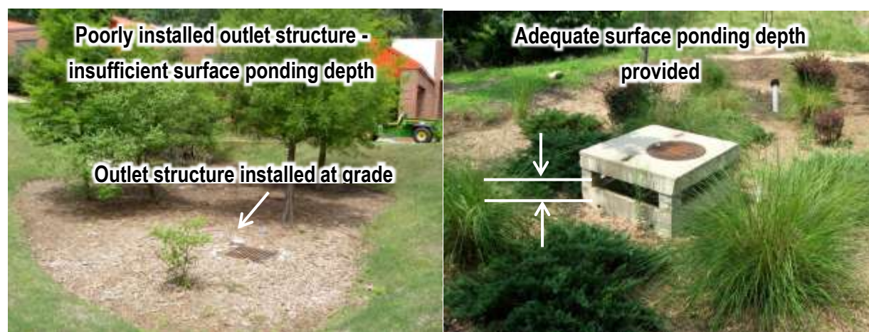
Figure 4-3. Accurate grading and outlet elevations must be provided to achieve intended hydrologic and water quality functions.
