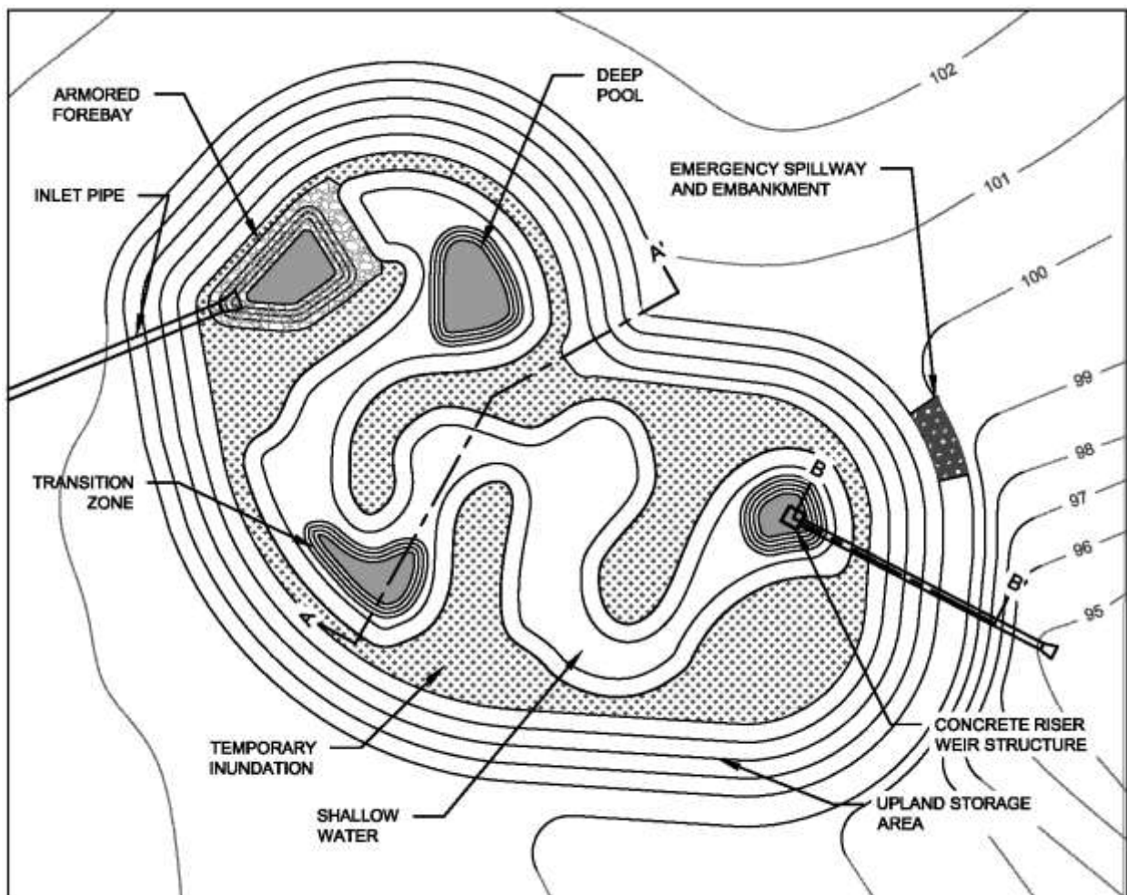
Figure B-7-1. Example wetland configuration.
