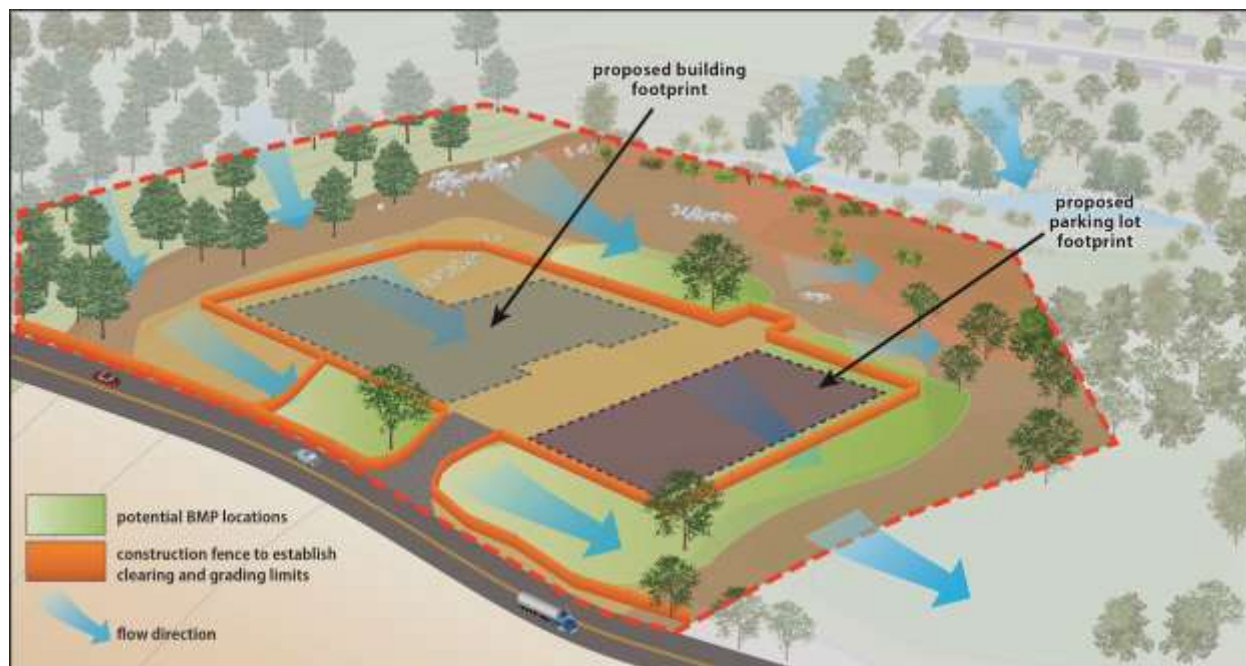
Figure 1-13. Establish grading envelope to protect natural areas and infiltrating soils.
