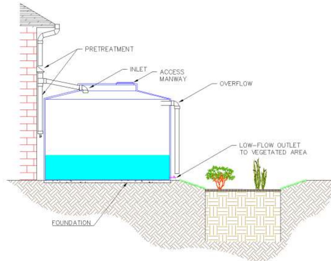
Figure B-8-1. Minimum design components of a rainwater harvesting system.
