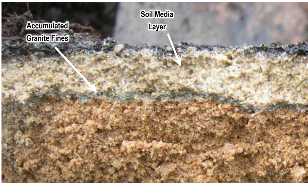
Figure 4-2. Accumulated fines layer as a result of improper construction sequencing.
