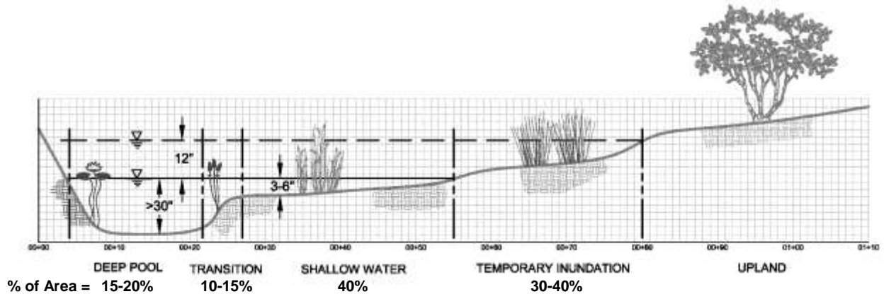
Figure B-7-5. Wetland zones.
