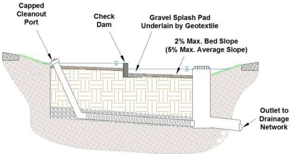
Figure B-2-5. Example profile of a bioswale with a check dam to retain the design storm volume.
