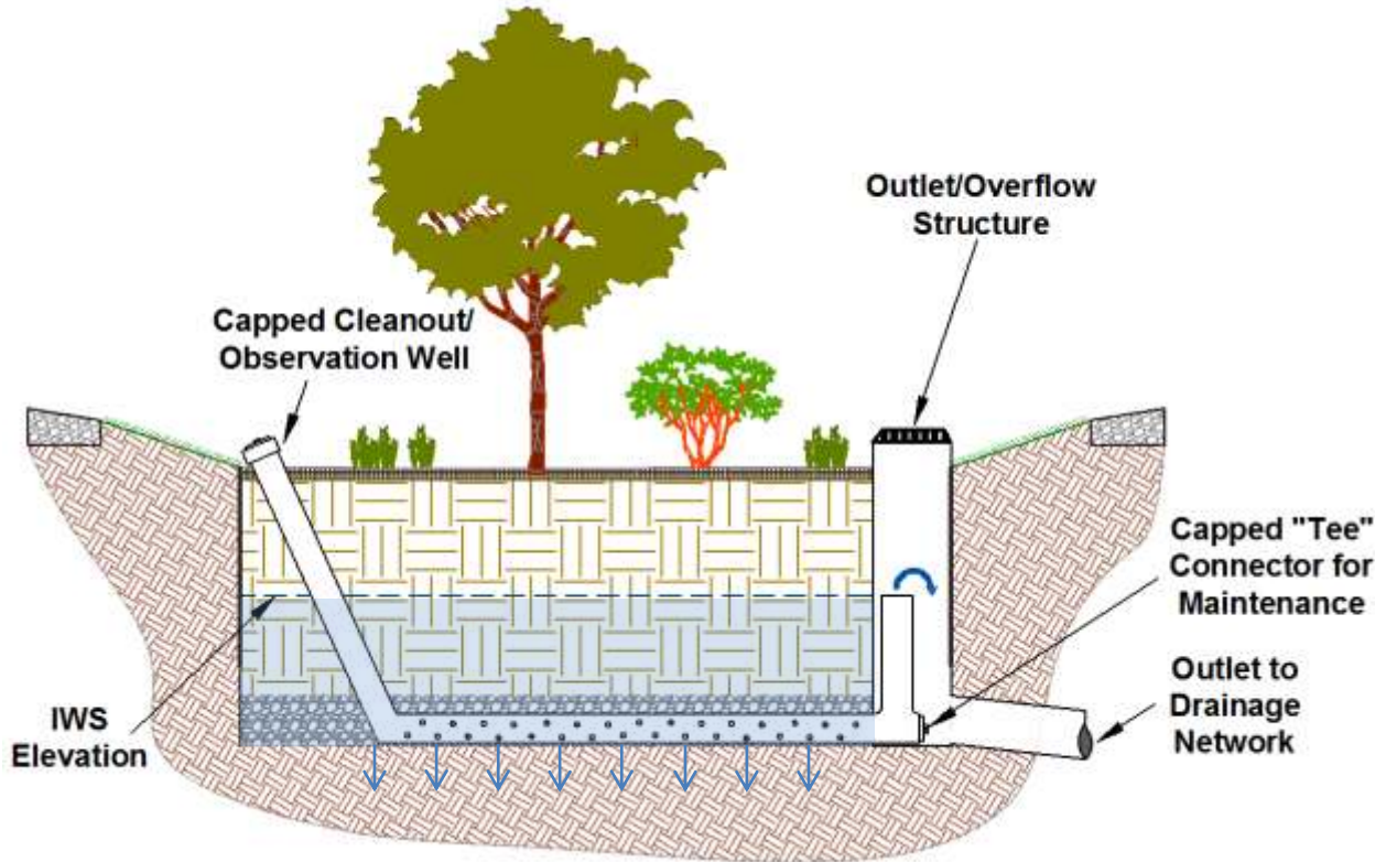
Figure B-1-3. Bioretention cell profile with IWS drainage configuration.
