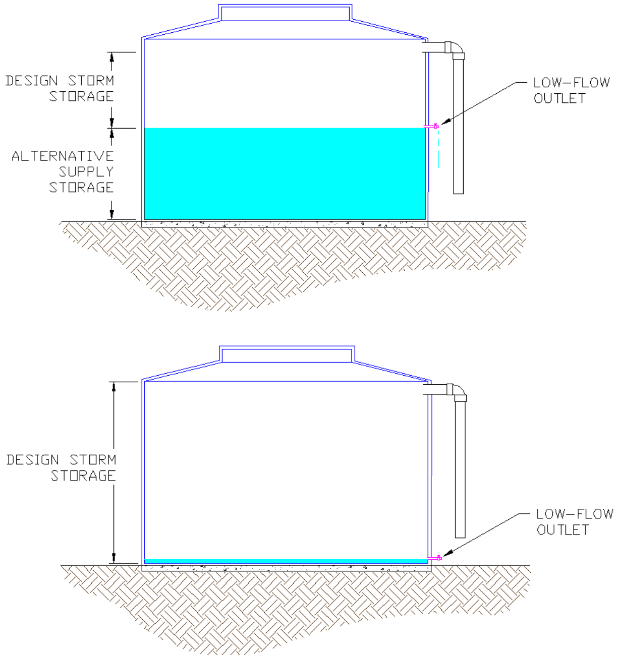
Figure B-8-17. Top: a low flow outlet is placed to provide equal parts detention storage and storage for alternative use. Bottom: placing the low flow outlet at the bottom of the cistern ensures maximum design storm storage.
