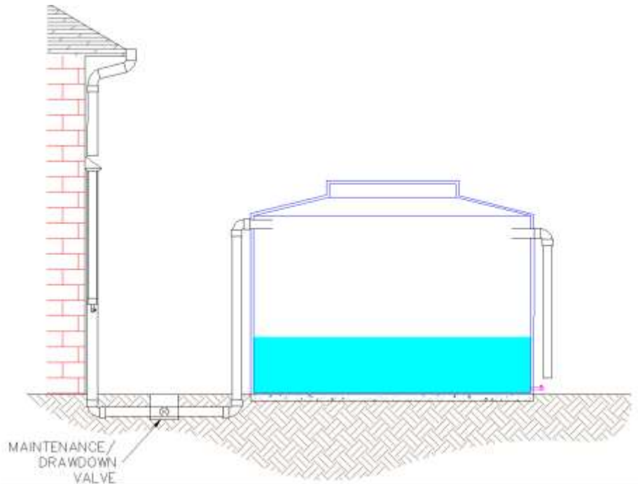
Figure B-8-8. Cistern with wet conveyance featuring a drawdown valve for maintenance.
