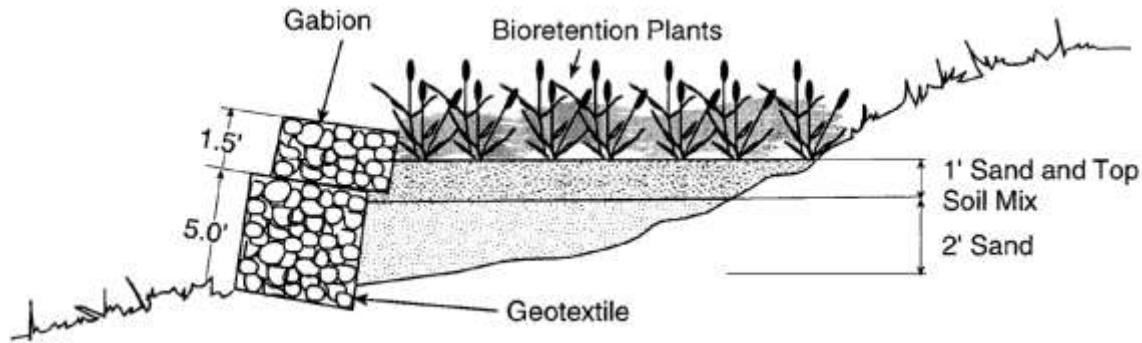
Figure 2-4. Bioretention Terrace Suitable for Use on Slopes 10-20% (NCDENR 2009)
