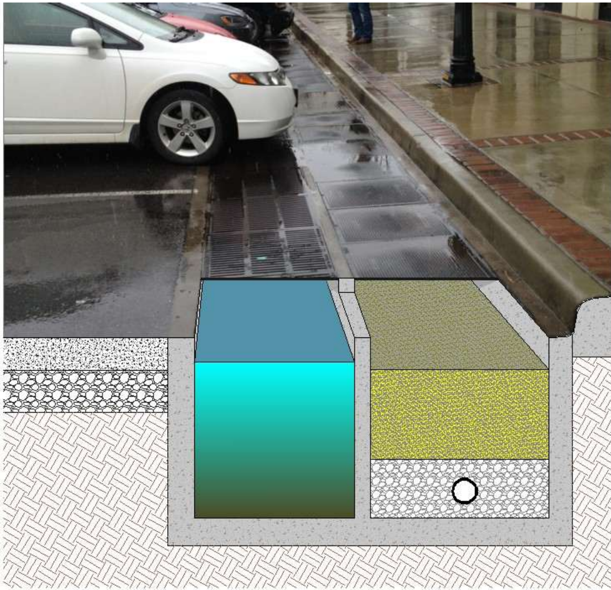
Figure B-6-5. Belowground sand filter with diffuse flow inlet and slot weirs between sedimentation chamber and sand filter chamber.
