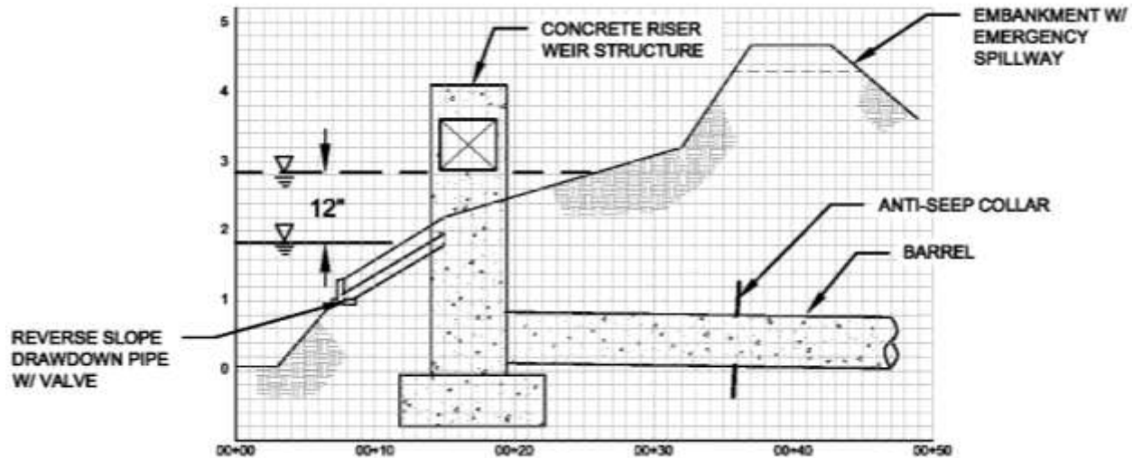
Figure B-7-6. Wetland outlet structure schematic.
