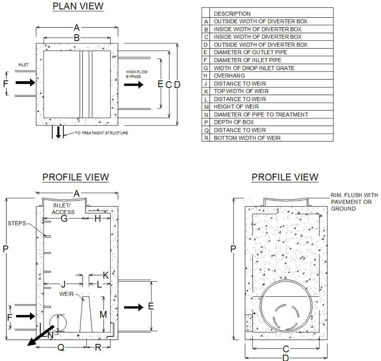
Figure B-11-18. Typical diversion structure.
