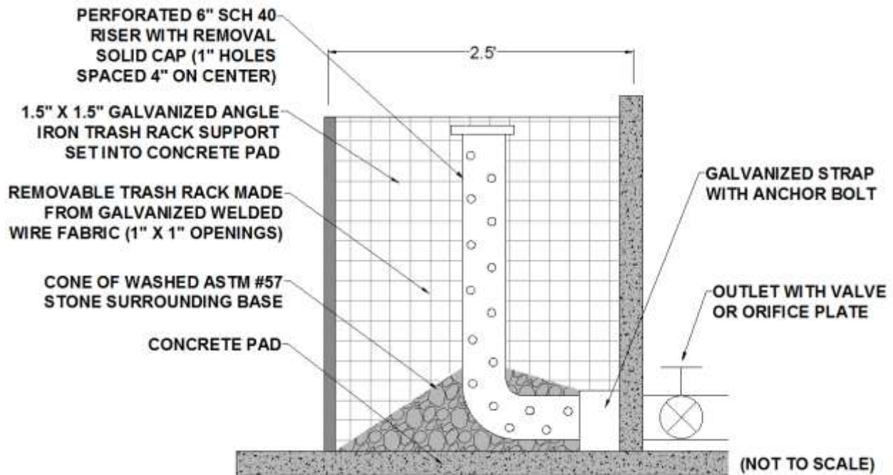
Figure B-11-17. Schematic of a trash rack for dewatering sedimentation chambers and stormwater wetlands (adapted from Barrett 2005).
