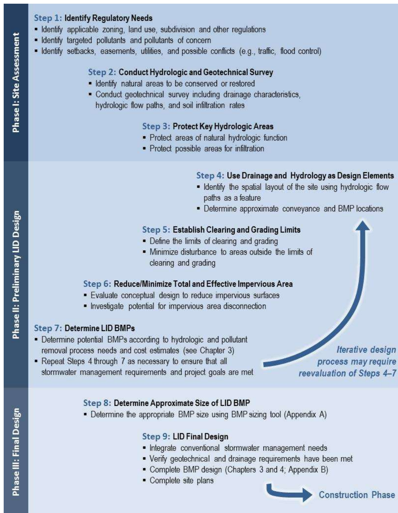
Figure 1-7. Steps to develop an LID-based site plan.
