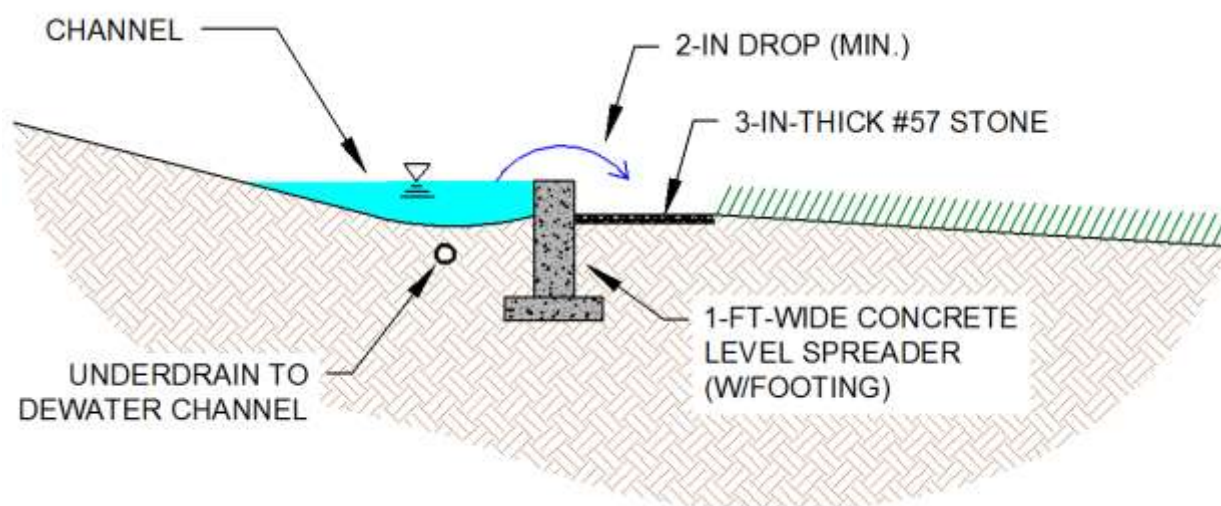
Figure B-11-10. Typical level spreader profile view.
