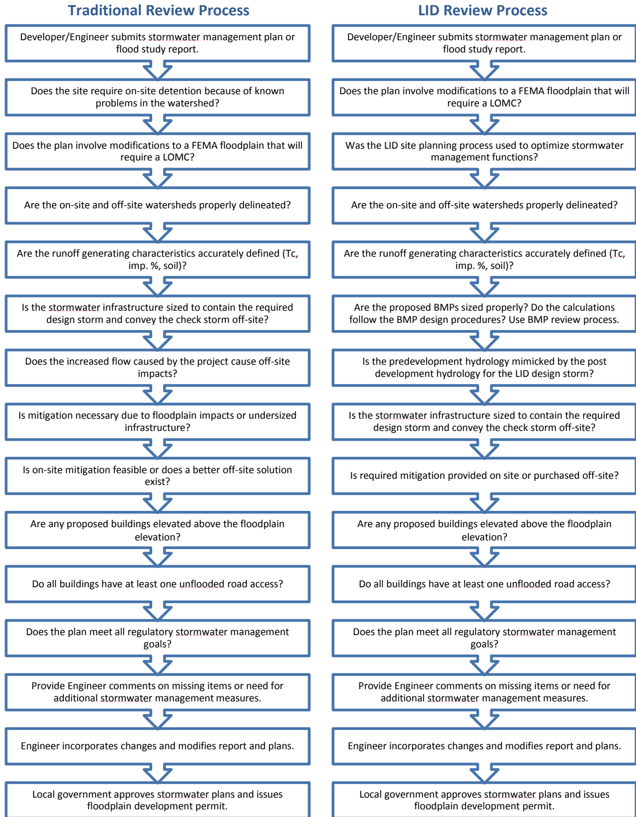
Figure 5-2. Traditional vs. LID design review process.
