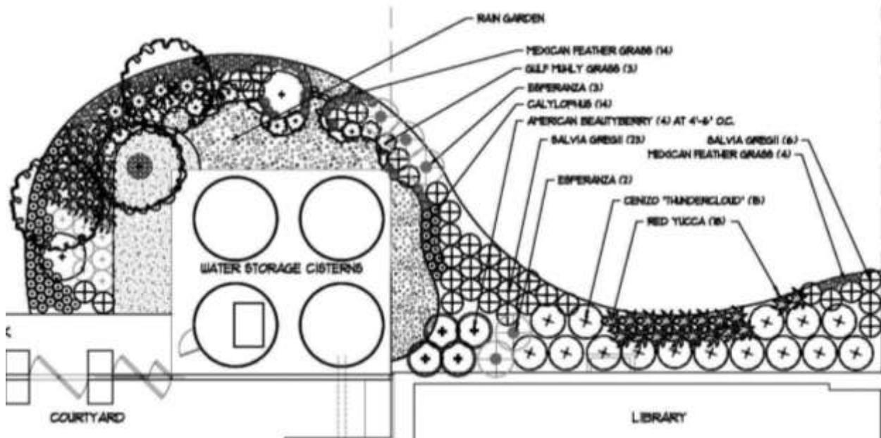
Figure B-1-13. Example bioretention planting plan.
