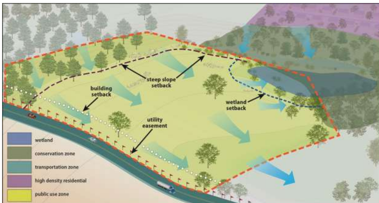
Figure 1-9. Identify applicable zoning requirements, utility easements, and site setbacks.
