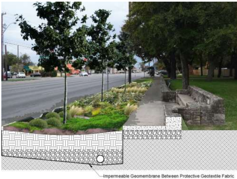
Figure B-11-21. Bioretention area with geomembrane liner.
