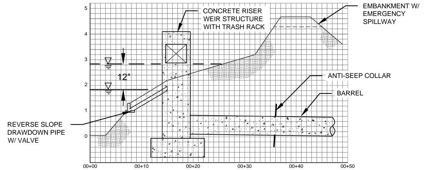
PROFILE B-B'
