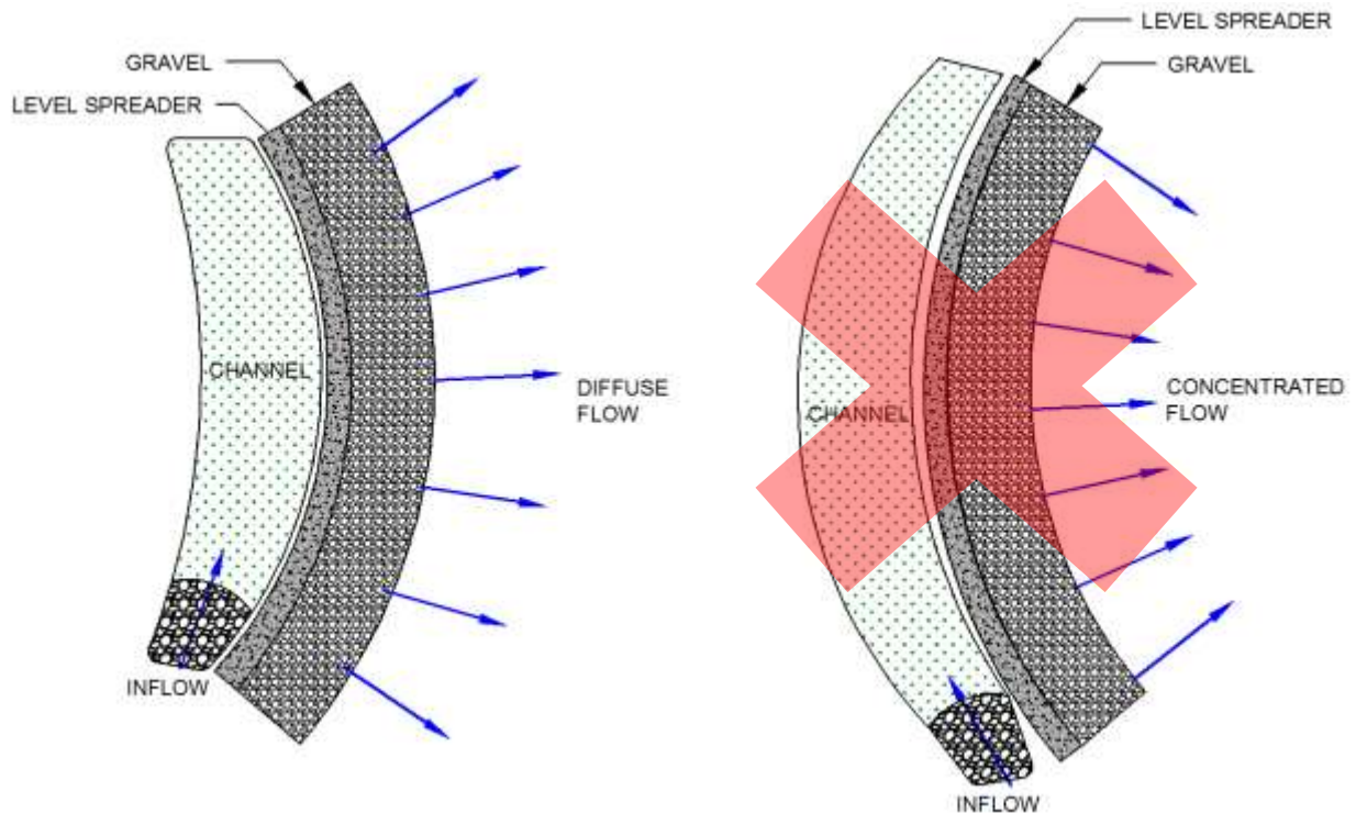
Figure B-11-12. Figure illustrating proper installation of arced level spreader (left) and improper level spreader arc (right)
