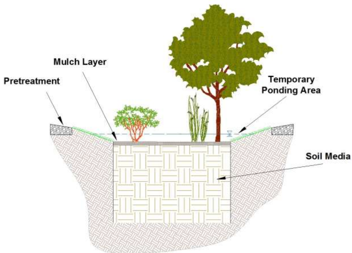
Figure B-1-1. Basic bioretention components.
