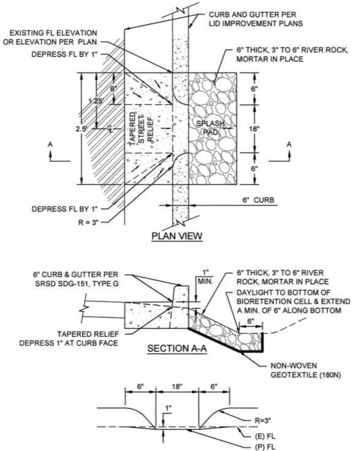
Figure B-11-1. Typical curb cut diagram.
