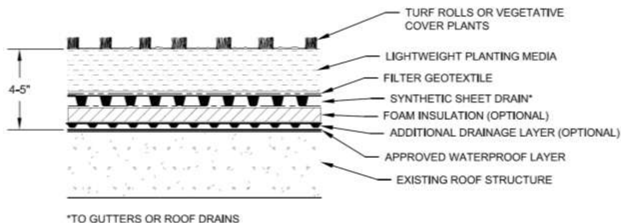
Figure B-5-3. Typical extensive green roof profile.
