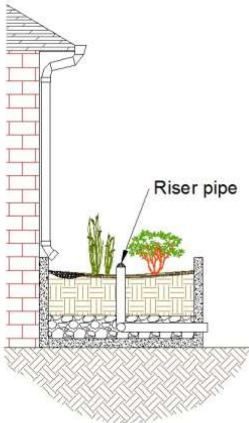
Figure B-4-3. Schematic of planter box with a vertical riser.
