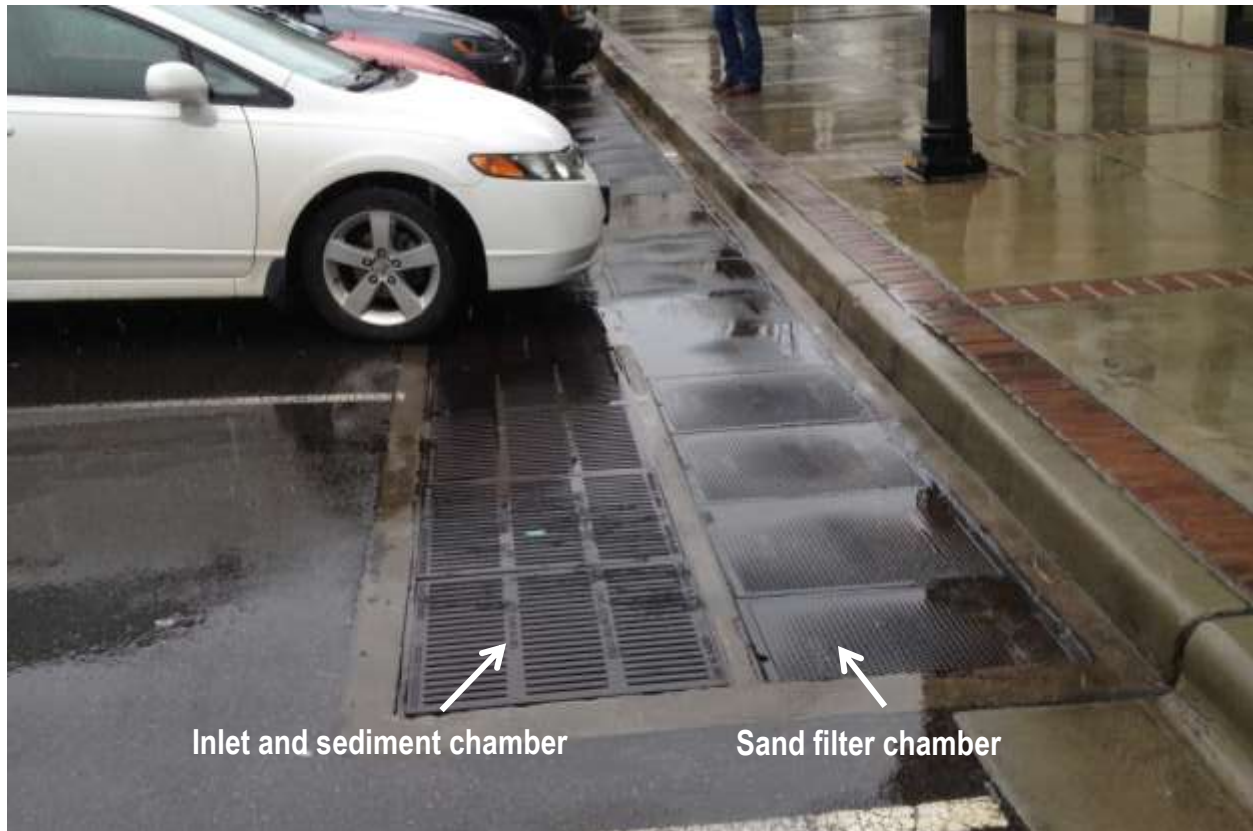
Figure B-6-2. Subsurface sand filter.
