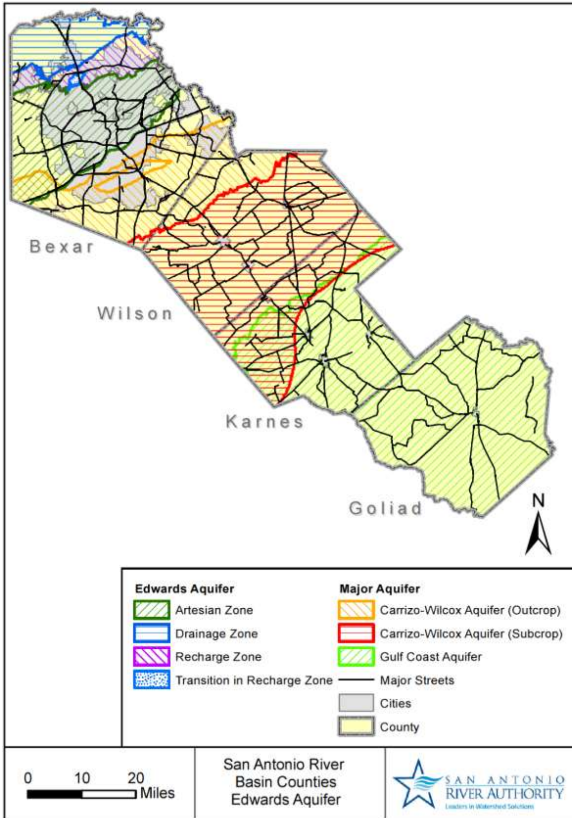
Figure 2-2. SARB artesian, drainage, recharge, and transition zones.
