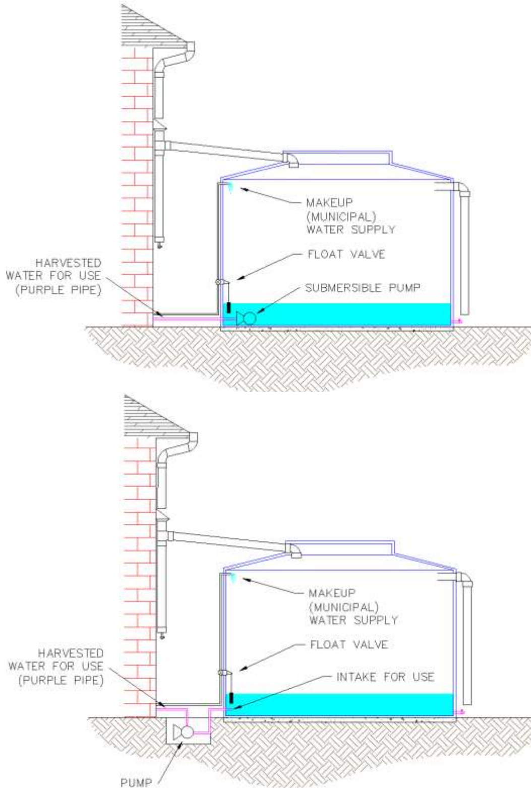
Figure B-8-20. Top: Conceptual schematic of cistern with submersible pump. Bottom: conceptual schematic of cistern with external pump.
