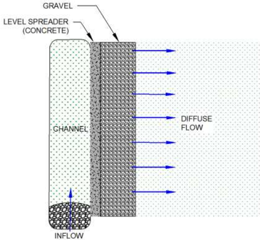
Figure B-11-11. Typical level spreader plan view.
