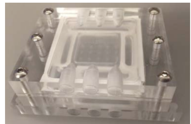
Prototype chassis machined from PMMA Concentration via Fresnel lens mounted to reactor
