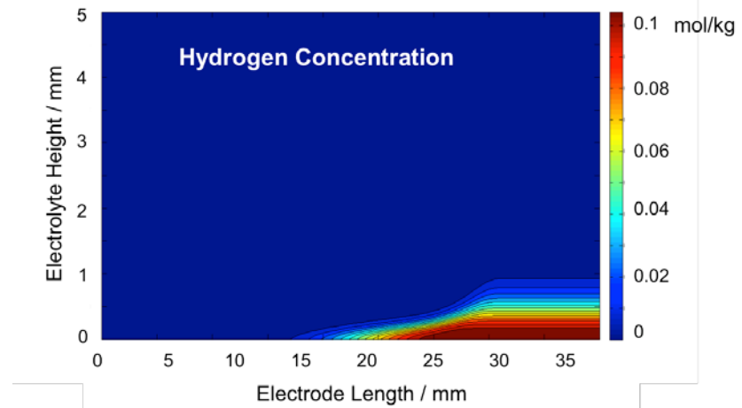
Only first 30 mm include generation: flow left→right 30 mm/s (avg) Minimum pressure to keep hydrogen in solution : 147 atm
