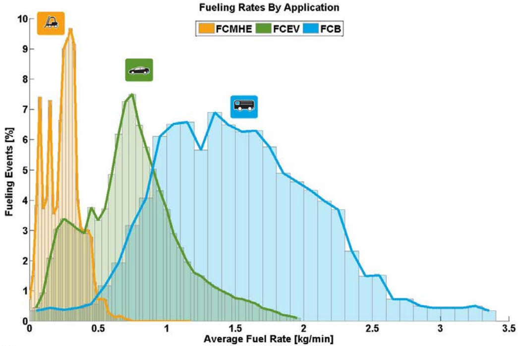
Figure 3.6.5 An example of a cross-application CDP, comparing fueling rates for fuel cell cars, buses, and forklifts.
