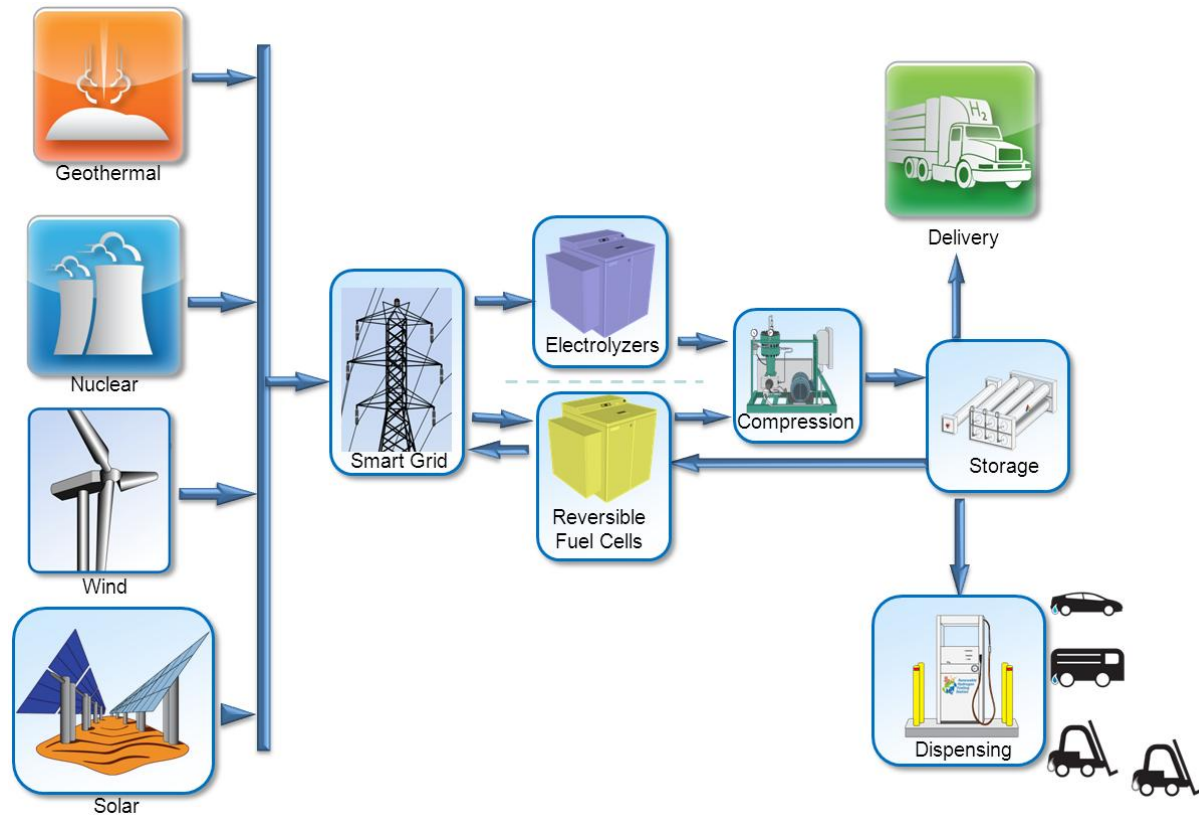
Figure 3.6.3 Electrolyzers and reversible fuel cells provide expanded market for base load and surplus renewable and zero-GHG power.
