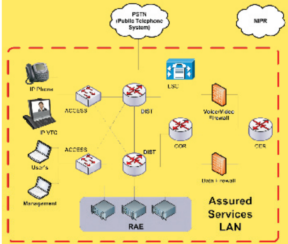
Figure 1. Voice over Secure IP (VoSIP)/Secure Voice over Internet Protocol and other secure real-time services provided by the voice systems integrated product team.
