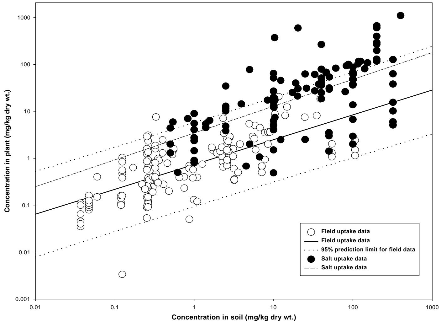
Fig. C.2. Scatterplot of cadmium concentrations in vegetation versus soil, where cadmium was added to soil in salt form or was present in a contaminated field soil. The regression lines for the salt uptake data and field uptake data are presented, as well as the 95% prediction limit for the field uptake data. All data are from published papers or reports.
