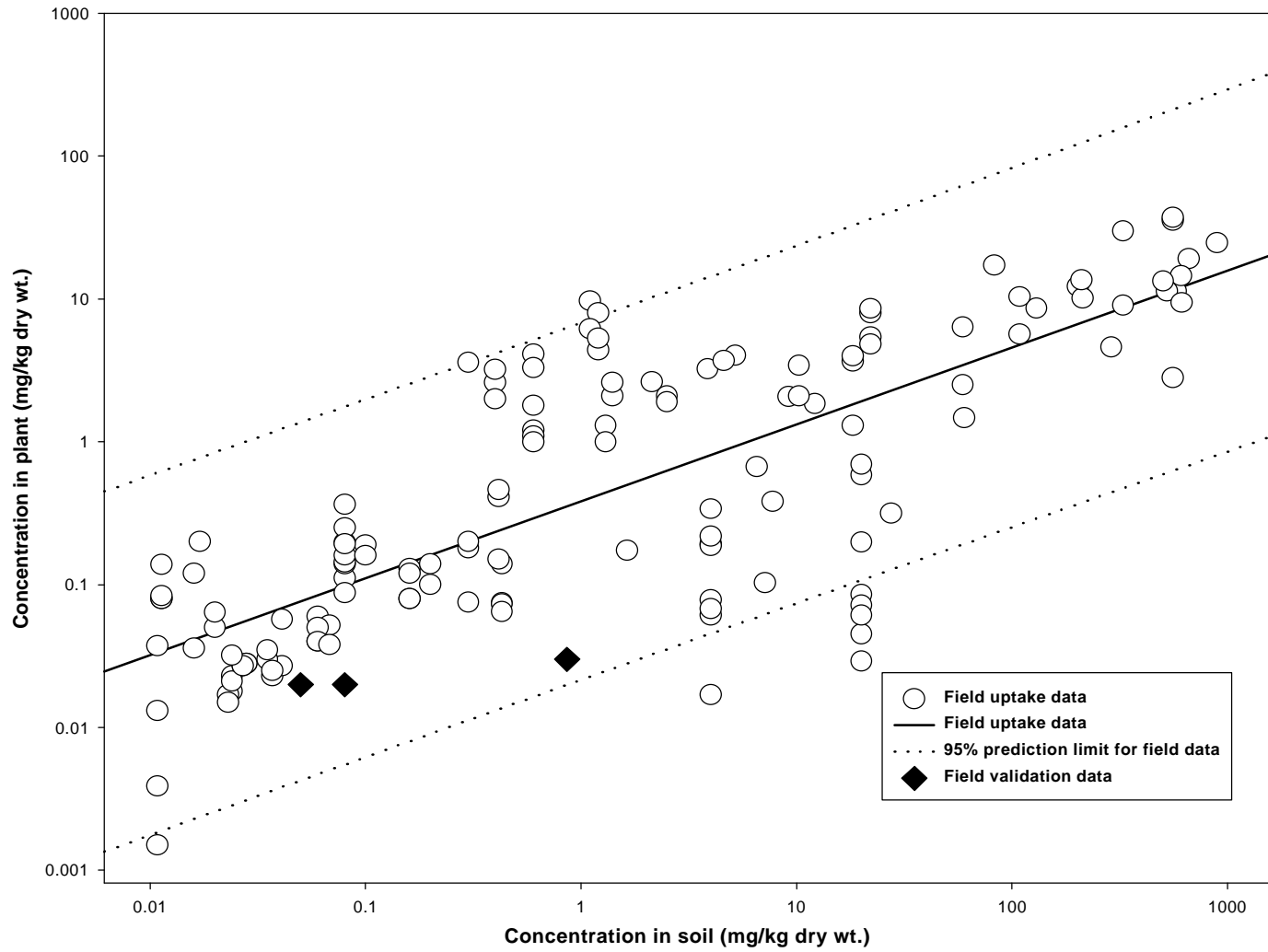
Fig. 5. Scatterplots of mercury concentrations in vegetation versus soil. Concentrations include both those from the initial model dataset and those from the validation dataset. The single-variable regression for the initial model dataset and the 95% upper prediction limit on the regression are depicted.
