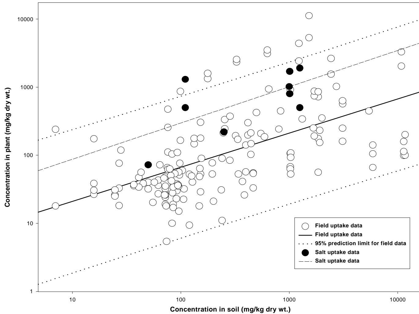
Fig. C.8. Scatterplot of zinc concentrations in vegetation versus soil, where zinc was added to soil in salt form or was present in a contaminated field soil. The regression lines for the salt uptake data and field uptake data are presented, as well as the 95% prediction limit for the field uptake data. All data are from published papers or reports.
