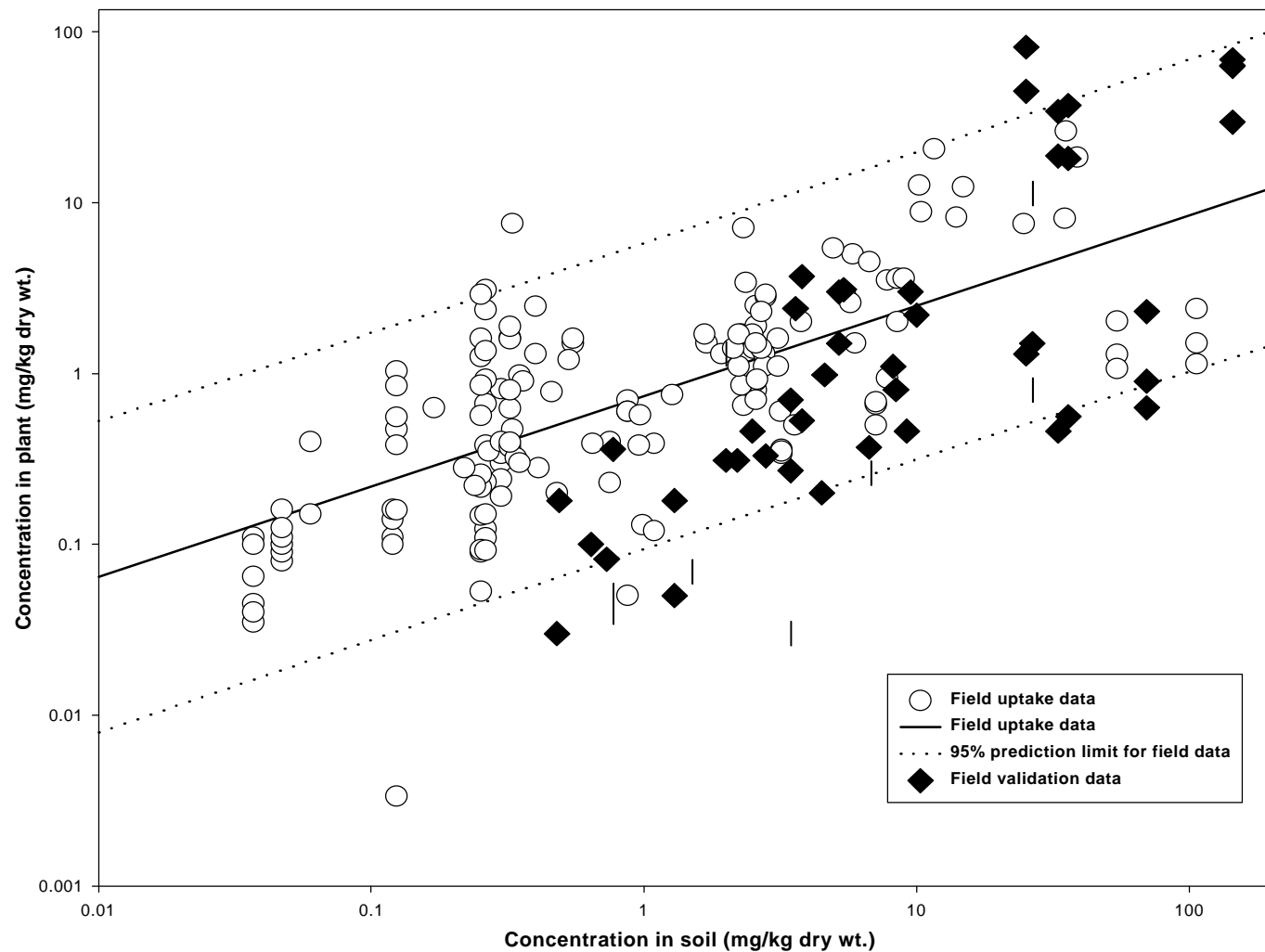
Fig. 2. Scatterplots of cadmium concentrations in vegetation versus soil. Concentrations include both those from the initial model dataset and those from the validation dataset. The single-variable regression for the initial model dataset and the 95% upper prediction limit on the regression are depicted.
