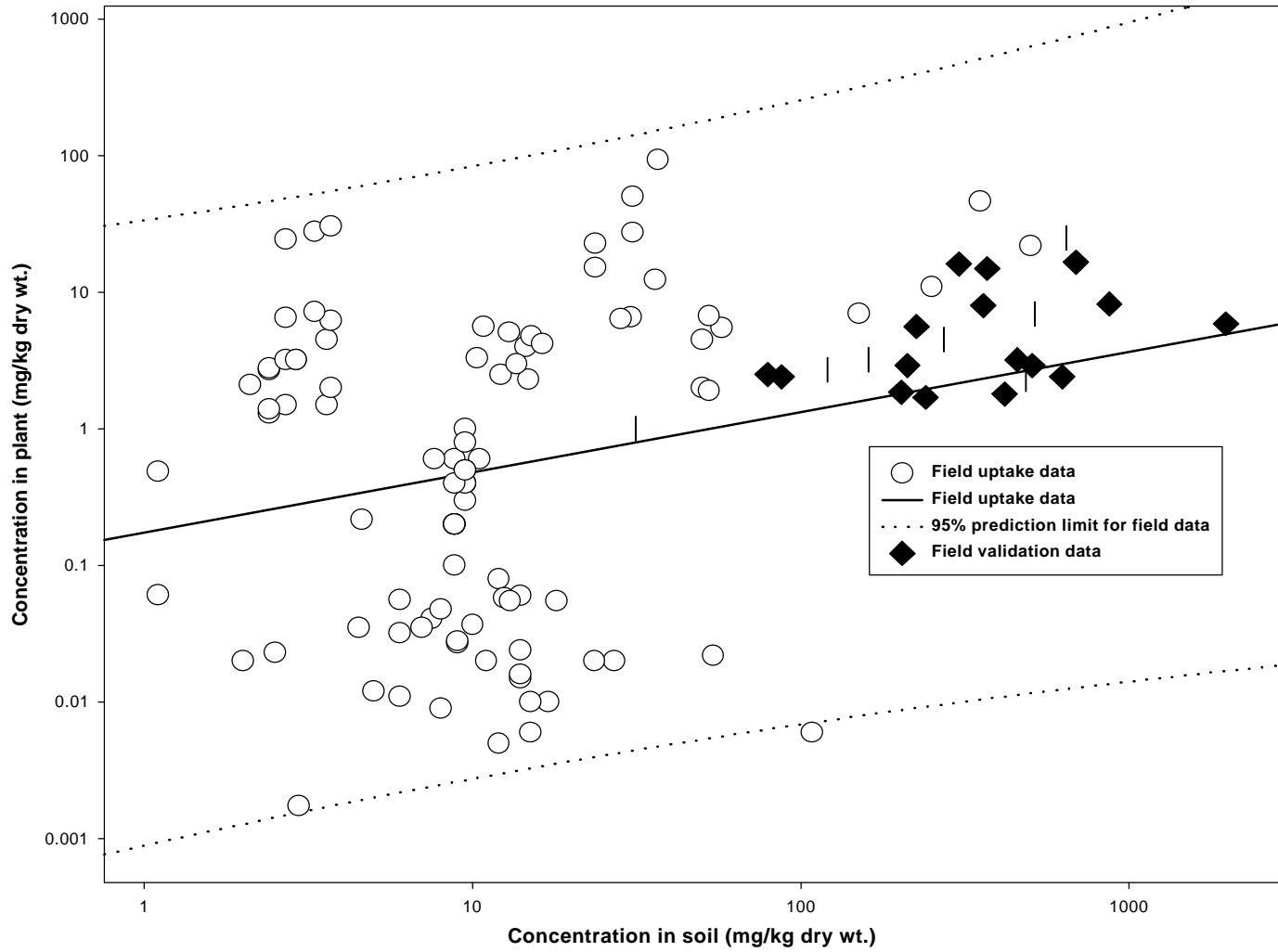
Fig. 1. Scatterplots of arsenic concentrations in vegetation versus soil. Concentrations include both those from the initial model dataset and those from the validation dataset. The single-variable regression for the initial model dataset and the 95% upper prediction limit on the regression are depicted.
