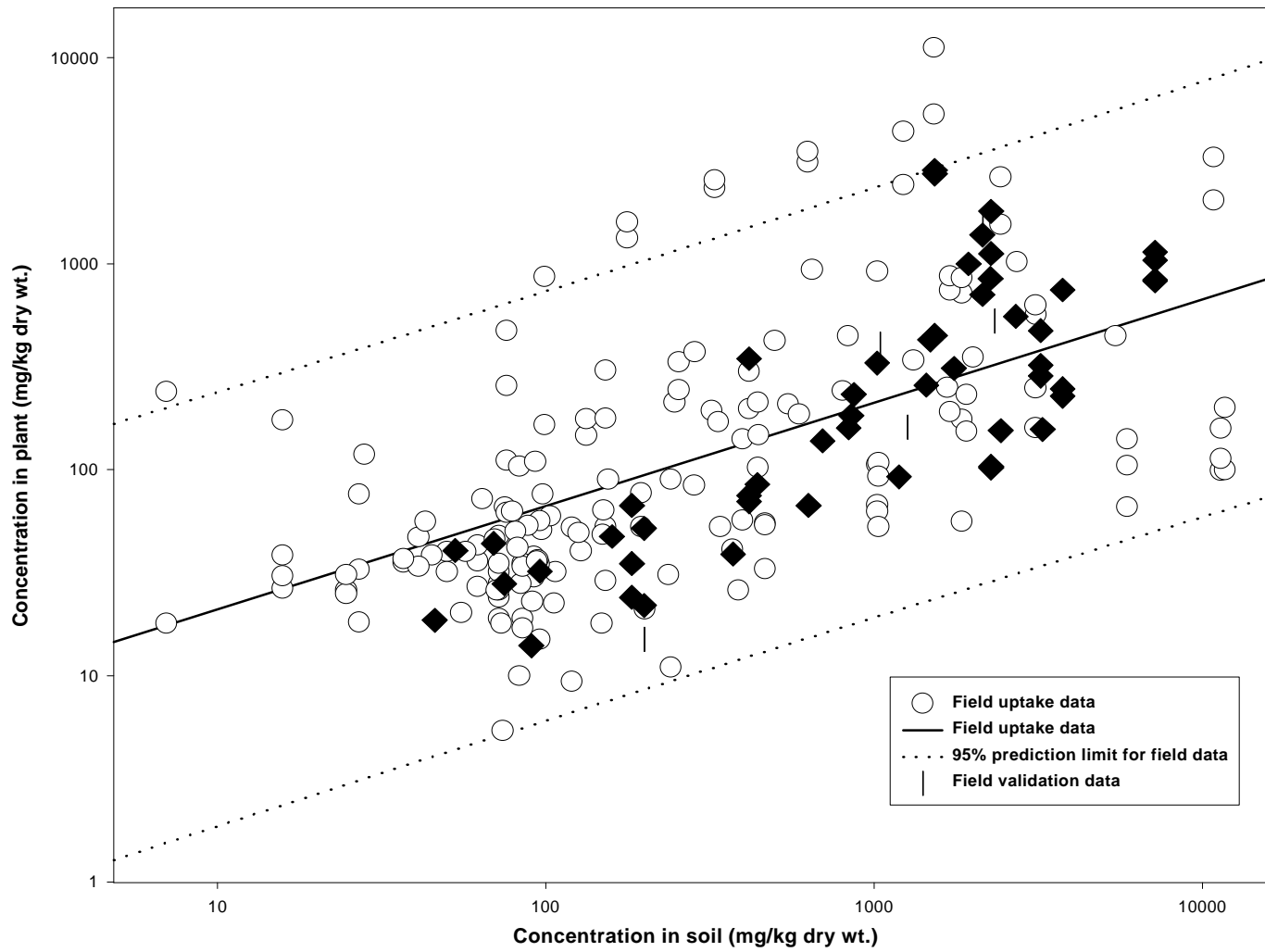
Fig. 8. Scatterplots of zinc concentrations in vegetation versus soil. Concentrations include both those from the initial model dataset and those from the validation dataset. The single-variable regression for the initial model dataset and the 95% upper prediction limit on the regression are depicted.
