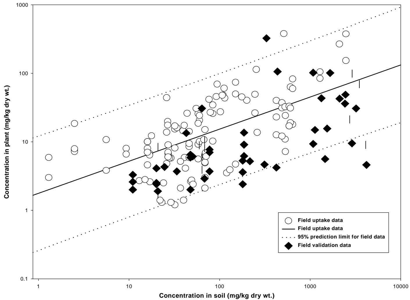
Fig. 3. Scatterplots of copper concentrations in vegetation versus soil. Concentrations include both those from the initial model dataset and those from the validation dataset. The single-variable regression for the initial model dataset and the 95% upper prediction limit on the regression are depicted.
