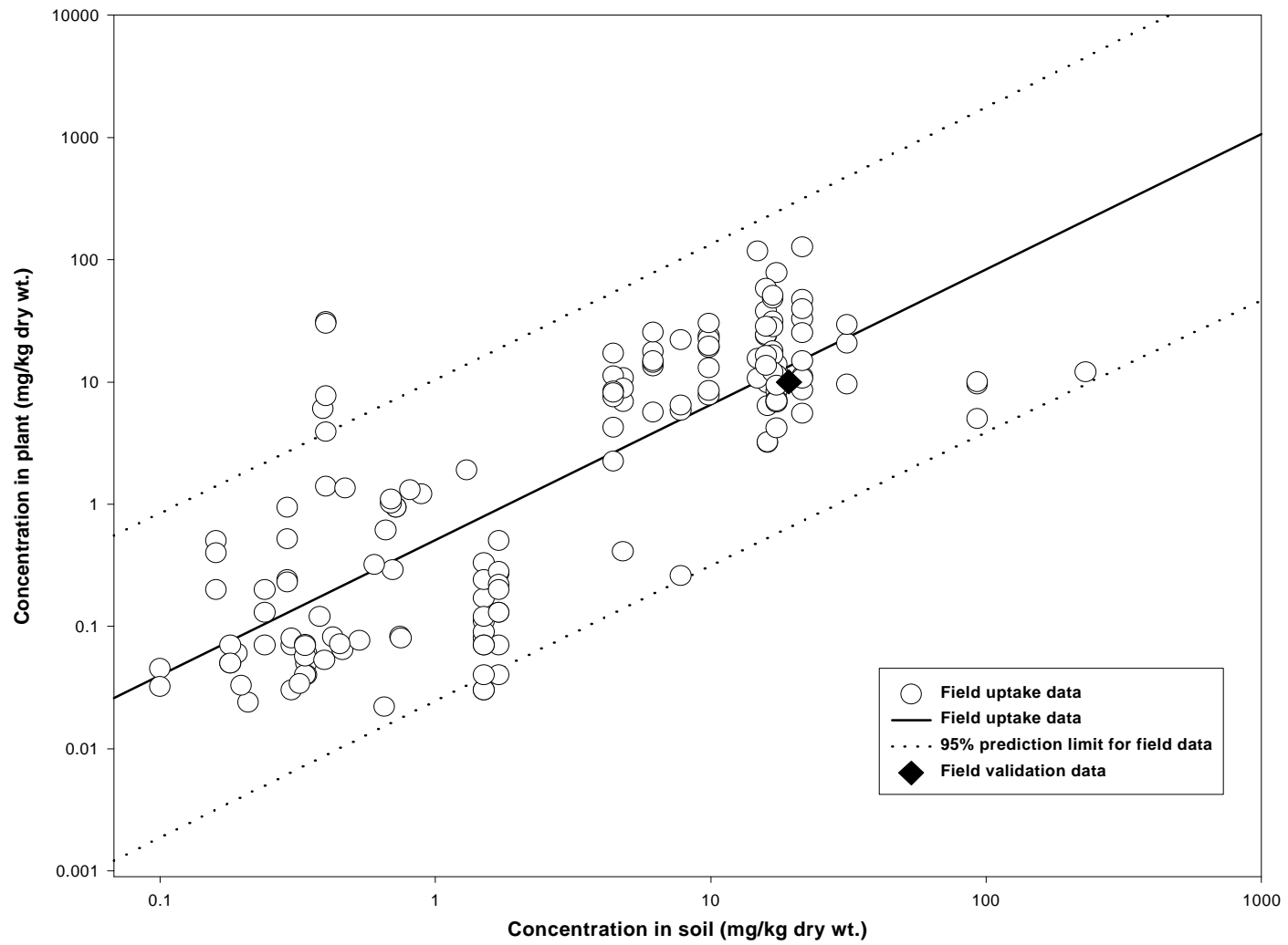
Fig. 7. Scatterplots of selenium concentrations in vegetation versus soil. Concentrations include both those from the initial model dataset and those from the validation dataset. The single-variable regression for the initial model dataset and the 95% upper prediction limit on the regression are depicted.
