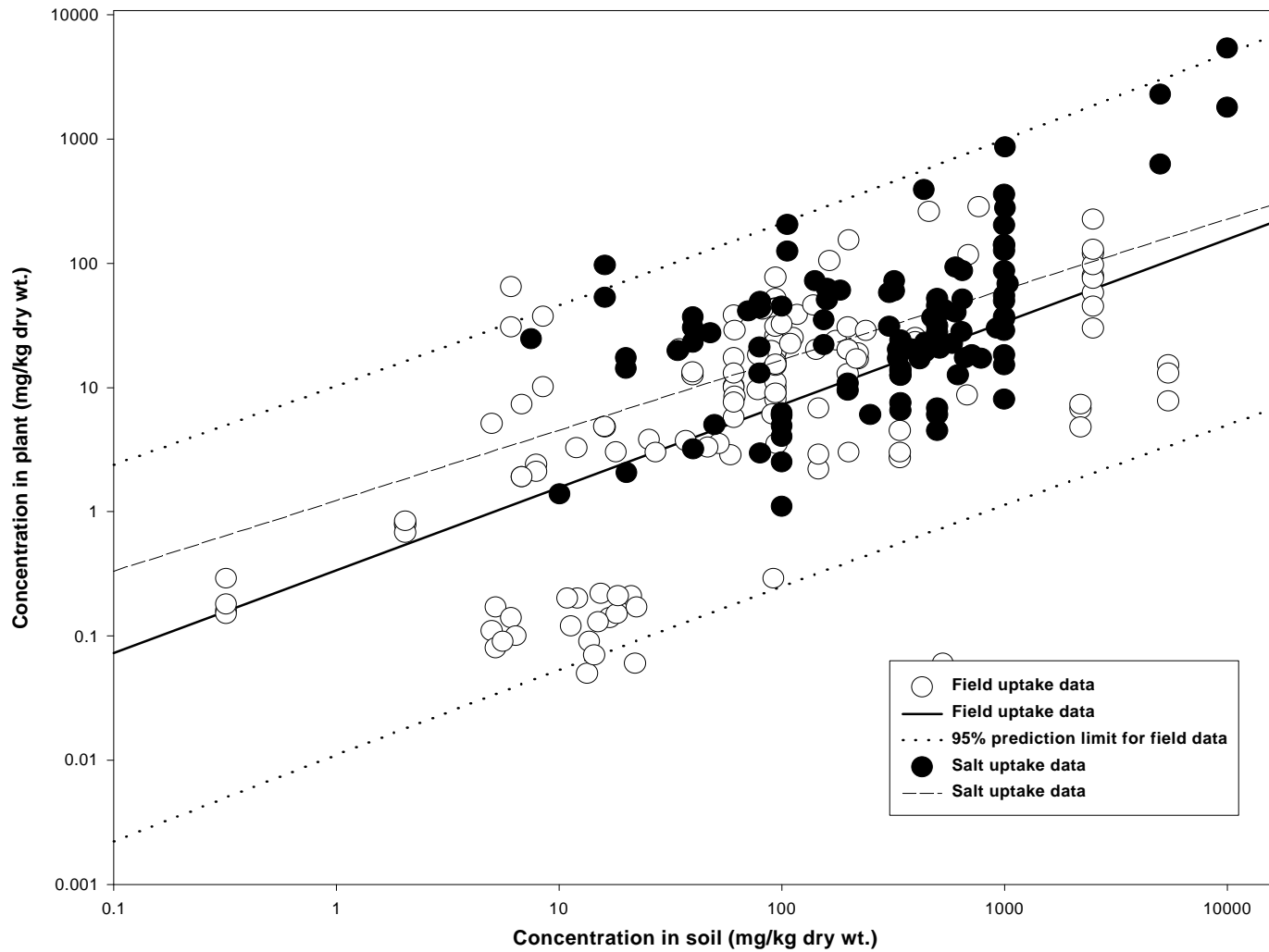
Fig. C.4. Scatterplot of lead concentrations in vegetation versus soil, where lead was added to soil in salt form or was present in a contaminated field soil. The regression lines for the salt uptake data and field uptake data are presented, as well as the 95% prediction limit for the field uptake data. All data are from published papers or reports.
