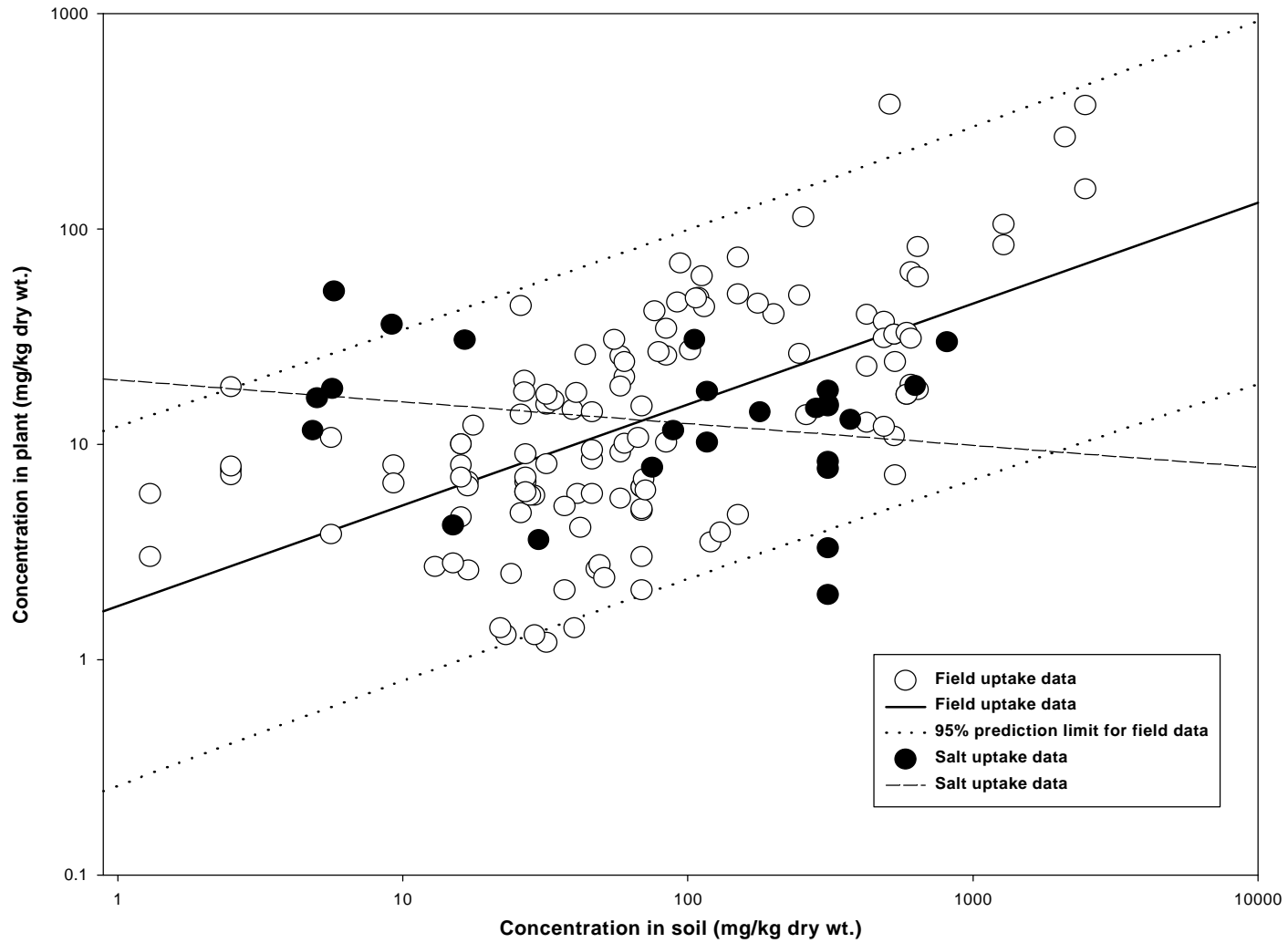
Fig. C.3. Scatterplot of copper concentrations in vegetation versus soil, where copper was added to soil in salt form or was present in a contaminated field soil. The regression lines for the salt uptake data and field uptake data are presented, as well as the 95% prediction limit for the field uptake data. All data are from published papers or reports.
