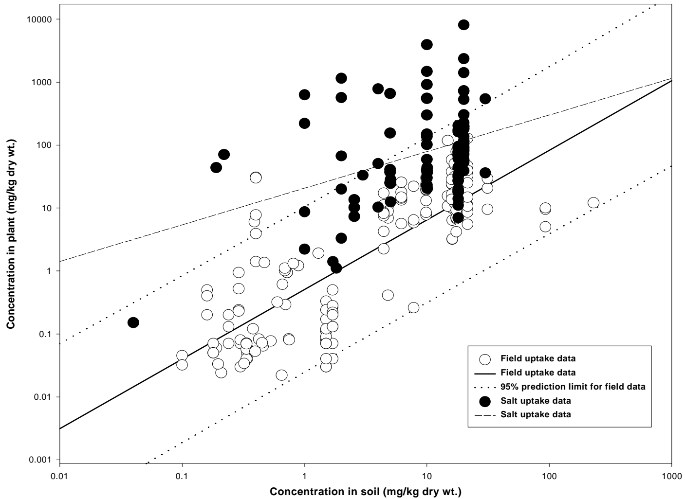
Fig. C.7. Scatterplot of selenium concentrations in vegetation versus soil, where selenium was added to soil in salt form or was present in a contaminated field soil. The regression lines for the salt uptake data and field uptake data are presented, as well as the 95% prediction limit for the field uptake data. All data are from published papers or reports.
