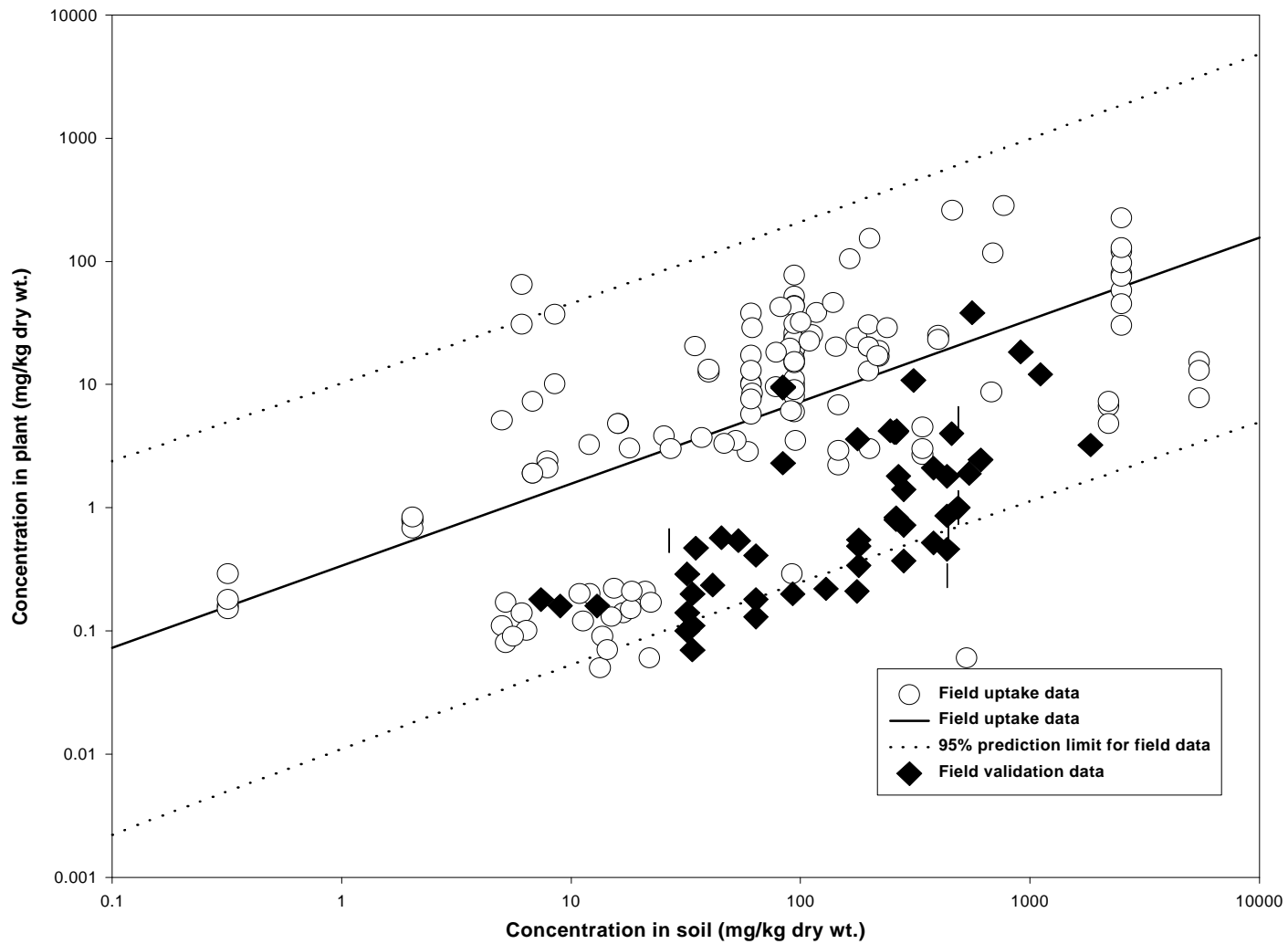
Fig. 4. Scatterplots of lead concentrations in vegetation versus soil. Concentrations include both those from the initial model dataset and those from the validation dataset. The single-variable regression for the initial model dataset and the 95% upper prediction limit on the regression are depicted.
