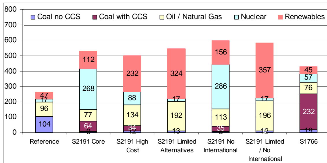
Figure 13: Cumulative Electricity Generating Capacity Additions (gigawatts)
