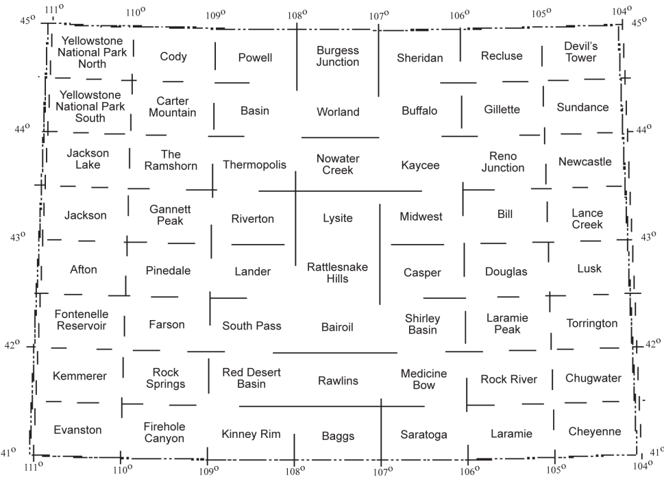
100K Index Map of Wyoming
