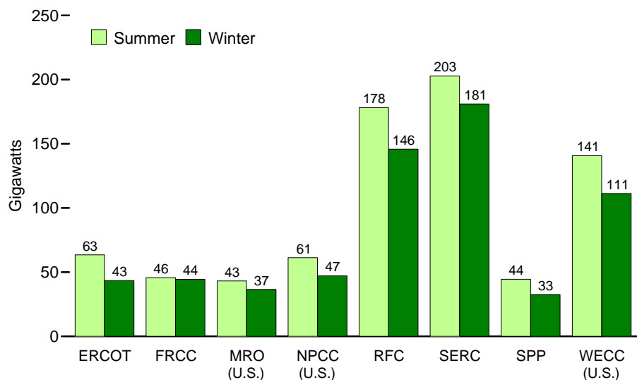
U.S. Peak Load by NERC Region, 2009
