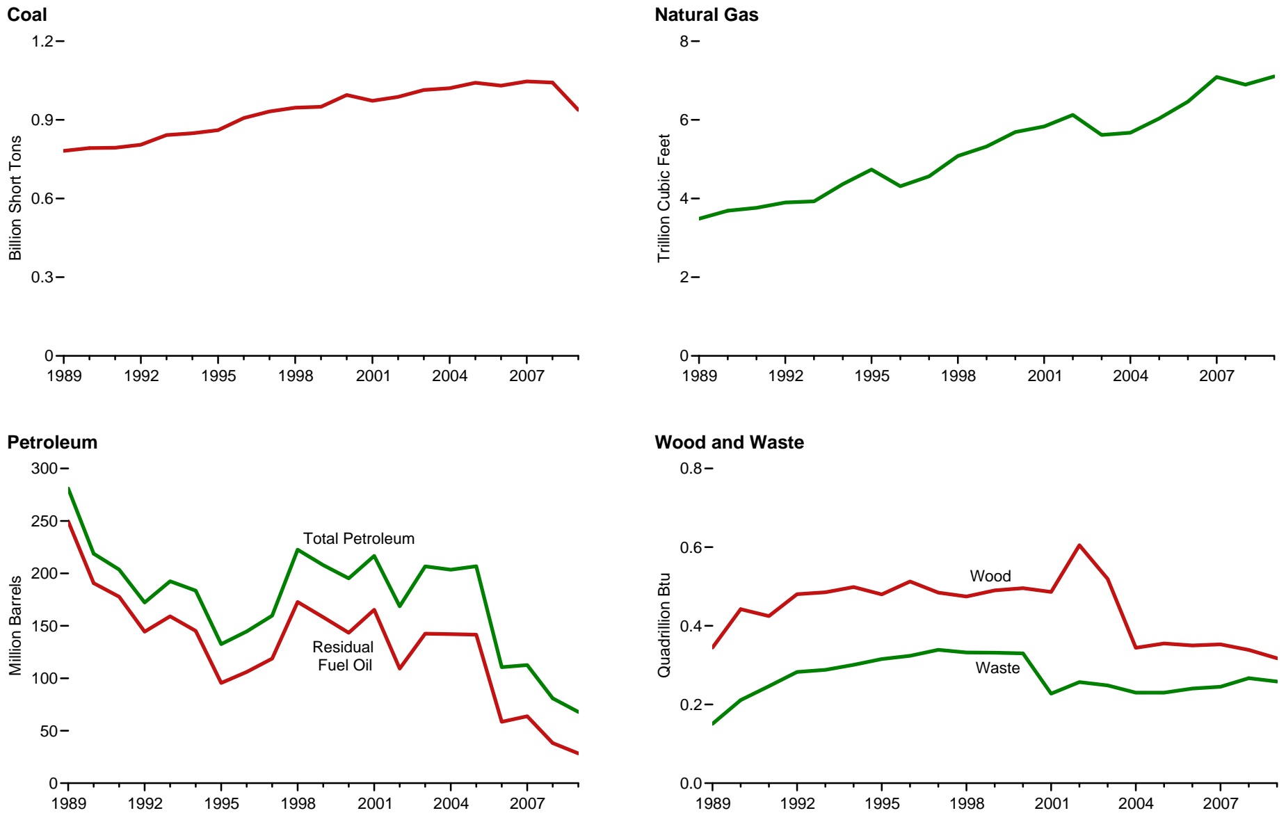
Figure 8.5a Consumption of Combustible Fuels for Electricity Generation (All Sectors), 1989-2009
