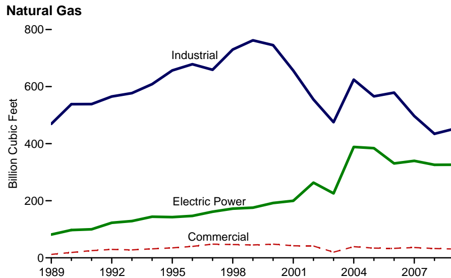
Figure 8.6 Estimated Consumption of Combustible Fuels for Useful Thermal Output at Combined-Heat-and-Power Plants by Sector, 1989-2009
