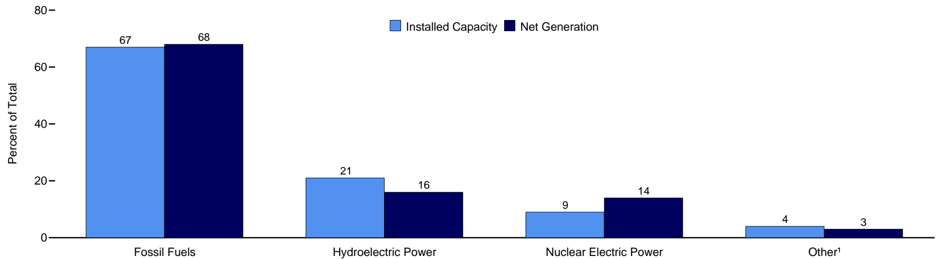
Installed Capacity and Net Generation Shares of Totals by Type, 2007
