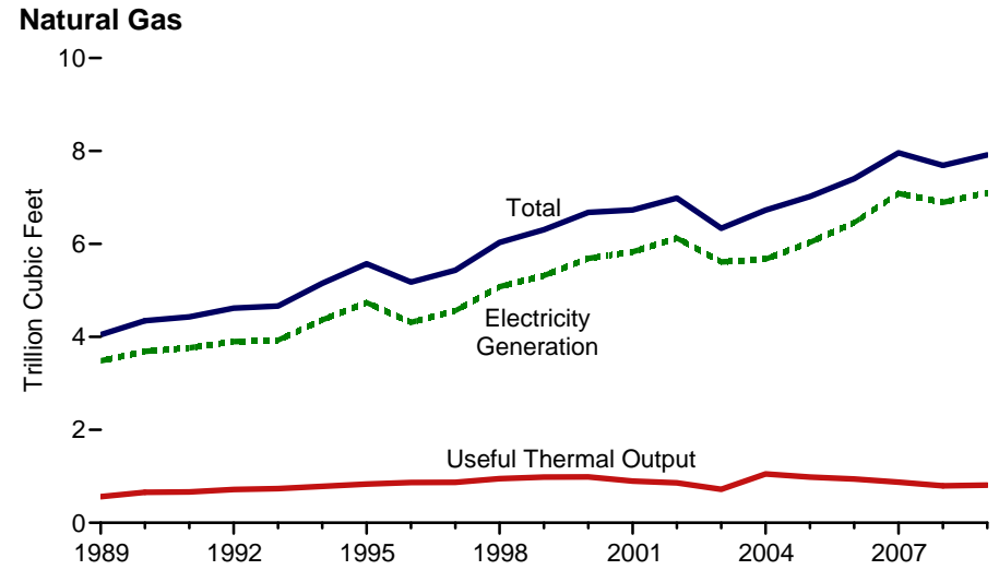
Figure 8.7 Consumption of Combustible Fuels for Electricity Generation and Useful Thermal Output, 1989-2009
