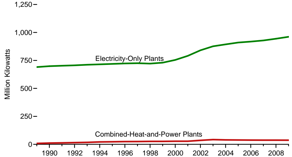
Electric Power Sector by Plant Type, 1989-2009
