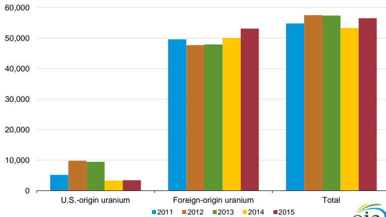
Figure 4. Weighted-average price of uranium purchased by owners and operators of U.S. civilian nuclear power reactors by origin and delivery year, 2011-15
