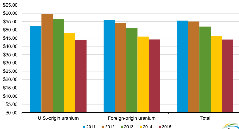
Figure 4. Weighted-average price of uranium purchased by owners and operators of U.S. civilian nuclear power reactors by origin and delivery year, 2011-15
