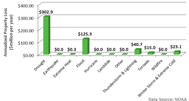
Annualized Property Loss due to Natural Hazards in Iowa (1996–2014)
