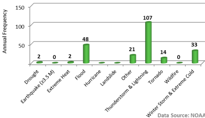
Annual Frequency of Occurrence of Natural Hazards in Iowa (1996–2014)
