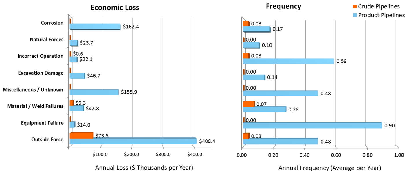
Top Events Affecting Crude Oil and Refined Product Pipelines in Iowa (1986–2014)
