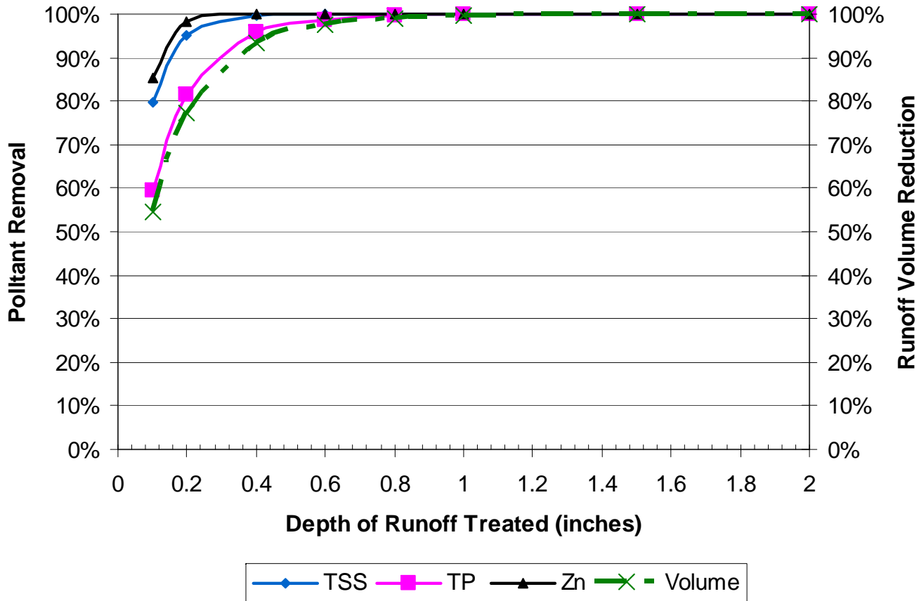
BMP Performance Curve: Infiltration Basin Land Use: High Density Residential (Soil infiltration rate 8.27 in/hr)
