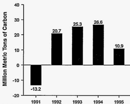
Annual Change in U.S. Carbon Dioxide Emissions, 1990-1995
