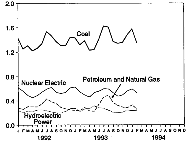
Input by Major Sources, February 1994
