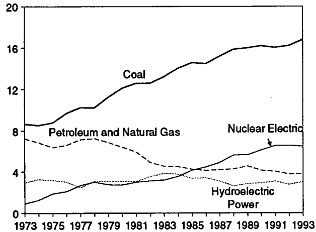
Input by Major Sources, 1973-1993
