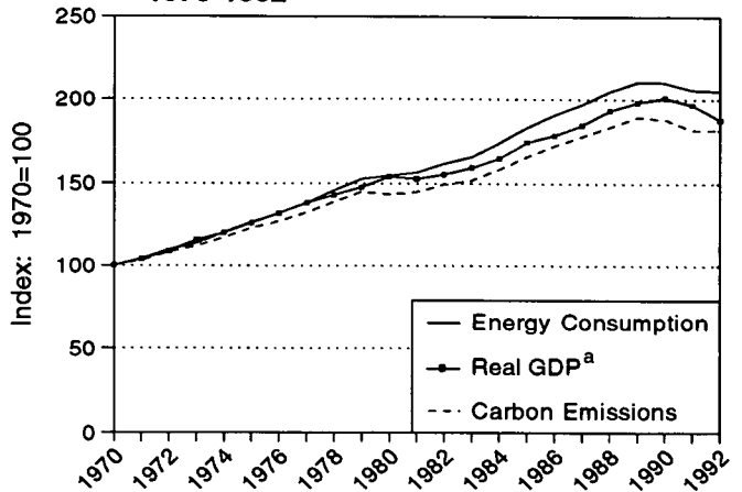
Figure 3. Non-OECD Economic Output, Energy Consumption, and Carbon Emissions, 1970-1992
