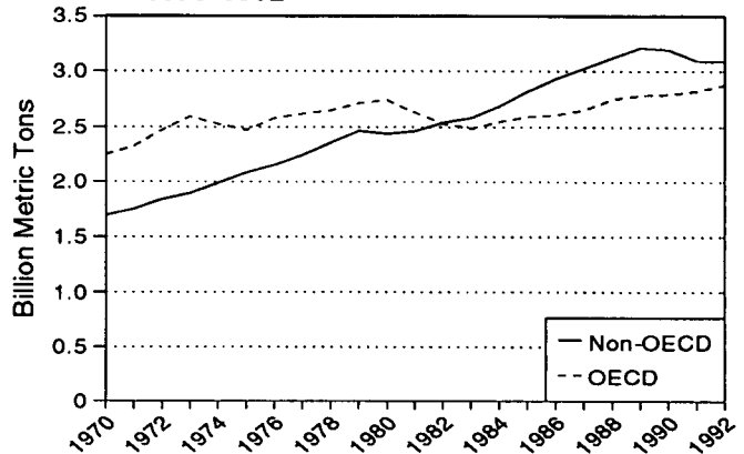
Figure 4. Energy-Related Carbon Emissions in OECD and Non-OECD Nations, 1970-1992
