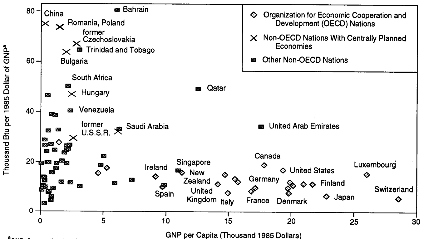
Figure 1. Energy Intensity Versus Per-Capita Gross National Product for 83 Countries, 1990
