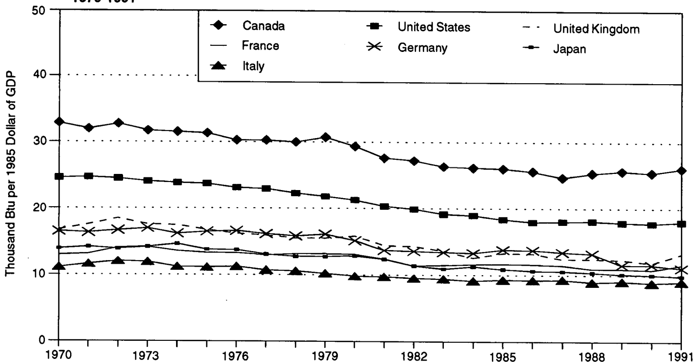
Figure 6. Energy Consumption per 1985 Dollar of GDP in the G-7 Nations, 1970-1991
